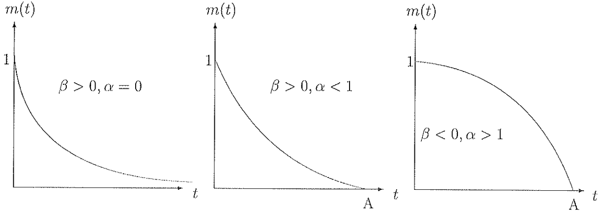
Figure 2: Survival laws
