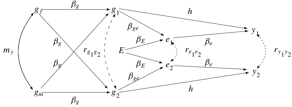
Figure 3: The Earnings of Brothers. In this diagram, g_f and g_m are the genotypes of father and mother, g_1 and g_2 are the genotypes of brothers, E is the common environment of brothers, e_1 and e_2 are the total environment of brothers, and y_1 and y_2 are the earnings of brothers. Here, m_y is the genetic relatedness of parents based on assortative mating, and as explained below, \beta_g = 1/2 , while h^2 is the heritability of earnings. The path labeled \beta_{ge} represents the tendency of genes to affect the environments ( \beta_{ge} > 0 means that identical twins experience more similar environments than fraternal twins).
