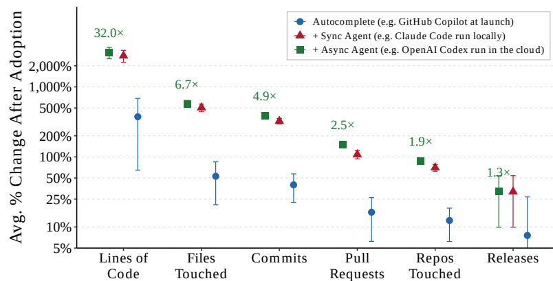
(c) Average level effect
