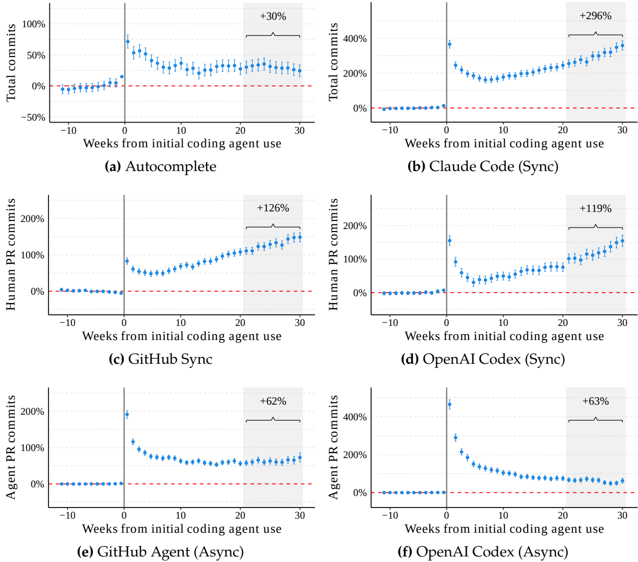
Figure OA-4: Task-Level Productivity Effect by AI Coding Tool
