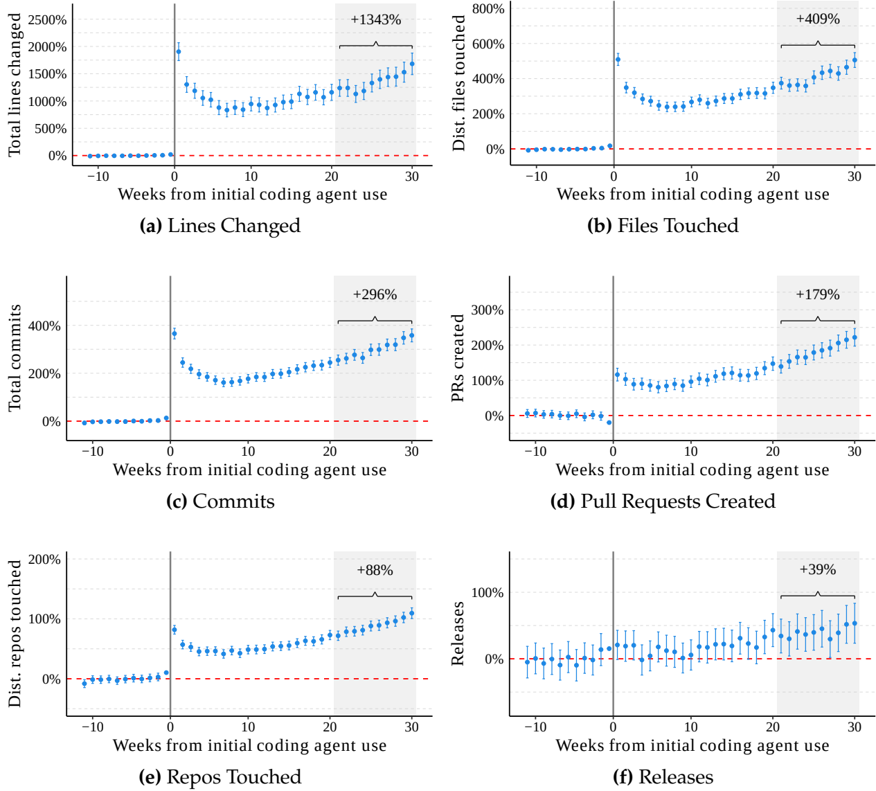
Figure OA-6: Productivity Effects Across the Production Hierarchy (Claude Code)
