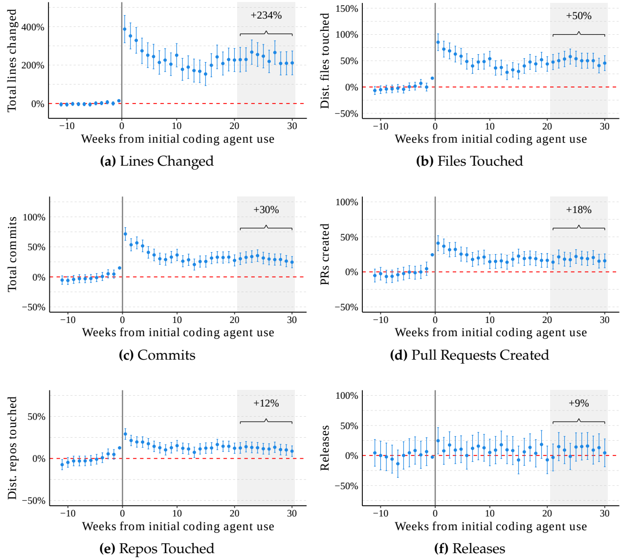
Figure OA-5: Productivity Effects Across the Production Hierarchy (Autocomplete)
