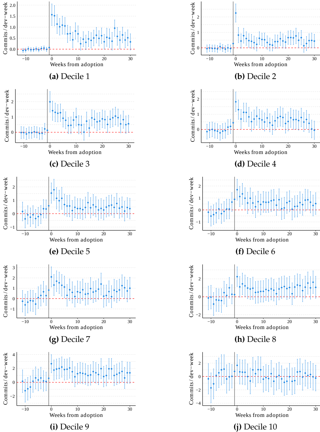
Figure OA-14: Level-Specification Event Studies by Pre-Period Decile: Autocomplete
