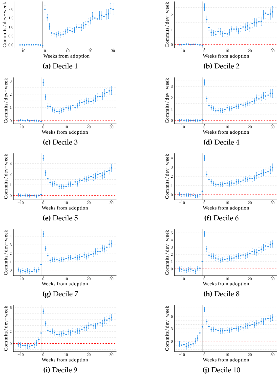
Figure OA-15: Level-Specification Event Studies by Pre-Period Decile: Pooled Sync
