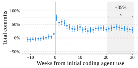
(e) No activity window: Autocomplete
