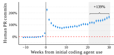
(j) Uniform commit+PR requirement: Pooled Sync
