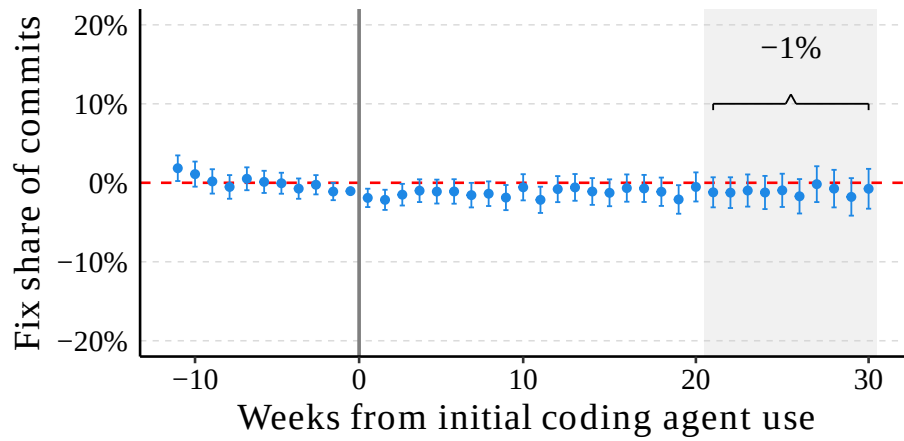
(b) Pooled Sync
