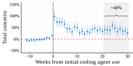
(g) Average effect: Autocomplete
