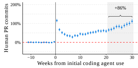
(b) Contemporaneous control: Pooled Sync
