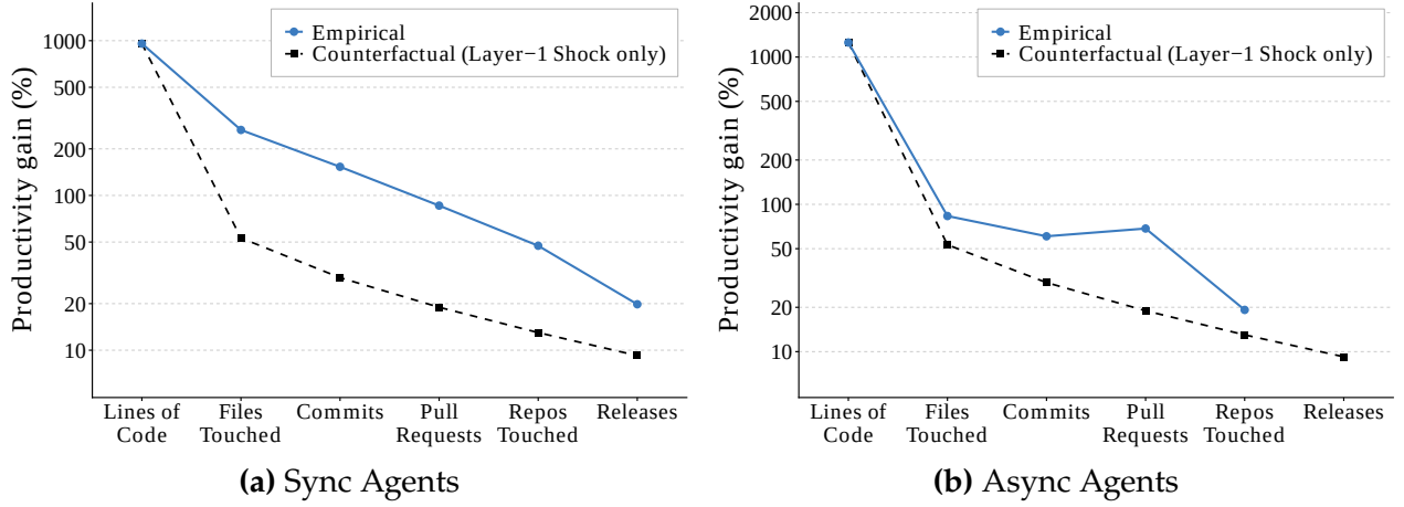
Figure 9: Measuring the Layers where Sync and Async Agents Intervene
