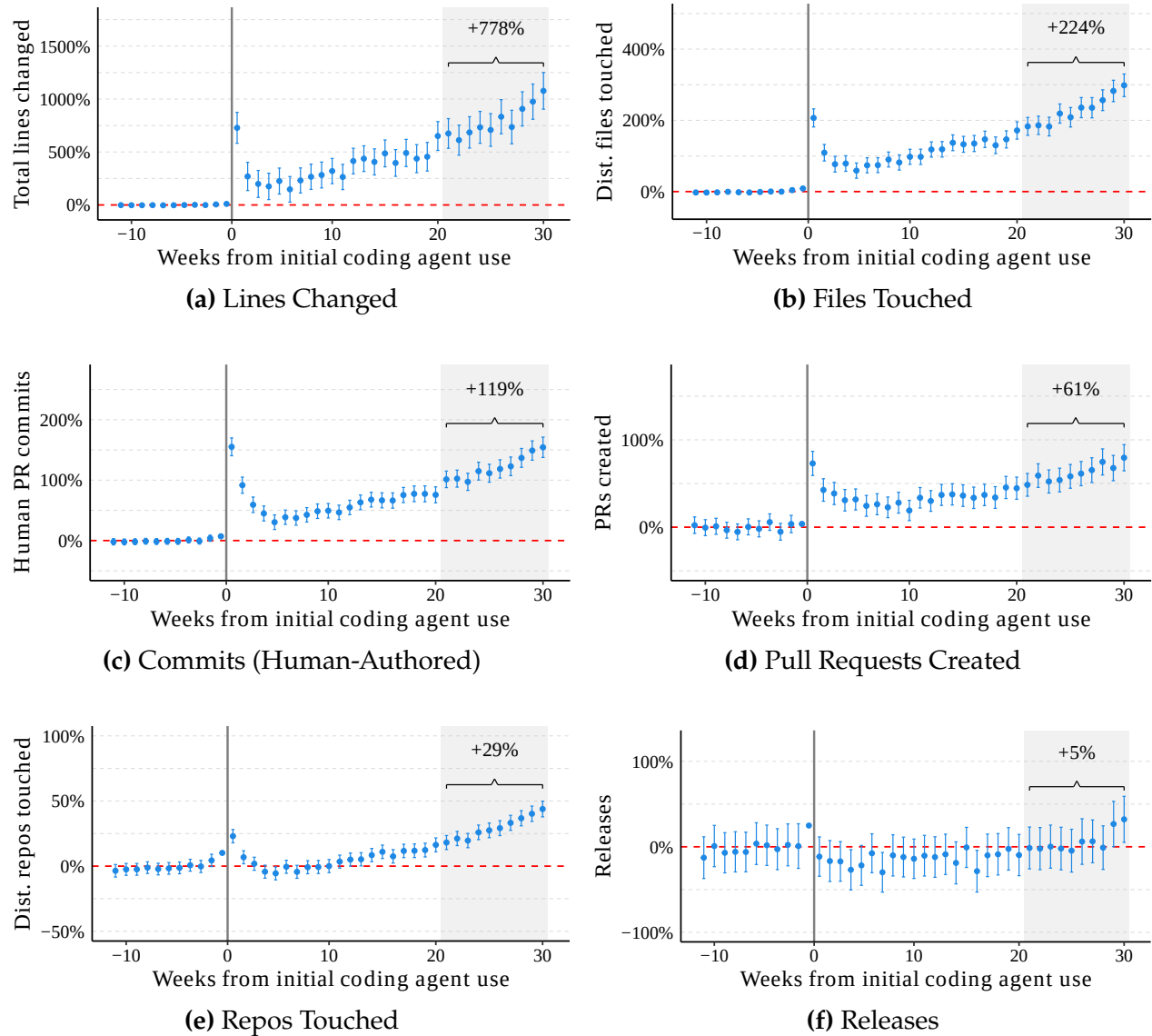
Figure OA-8: Productivity Effects Across the Production Hierarchy (Codex Sync)
