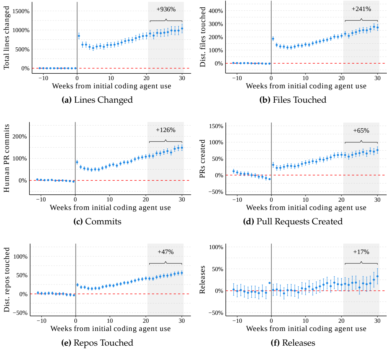
Figure OA-7: Productivity Effects Across the Production Hierarchy (GitHub Sync, Pooled)
