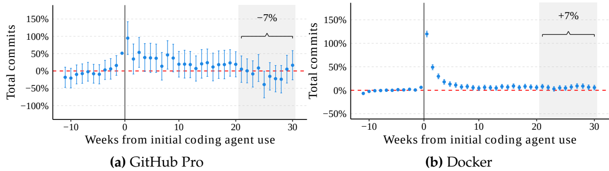
Figure 6: Placebos: Productivity Effects of Other Coding Tools
