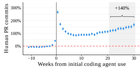
(h) Uniform PR requirement: Pooled Sync
