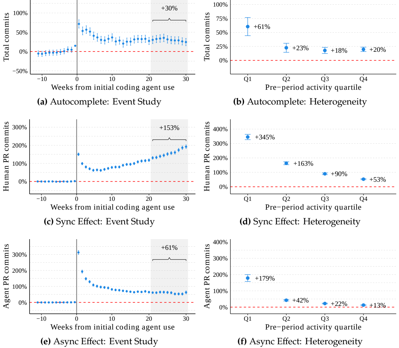
Figure 4: Task-Level Productivity Effects of AI Coding Tools
