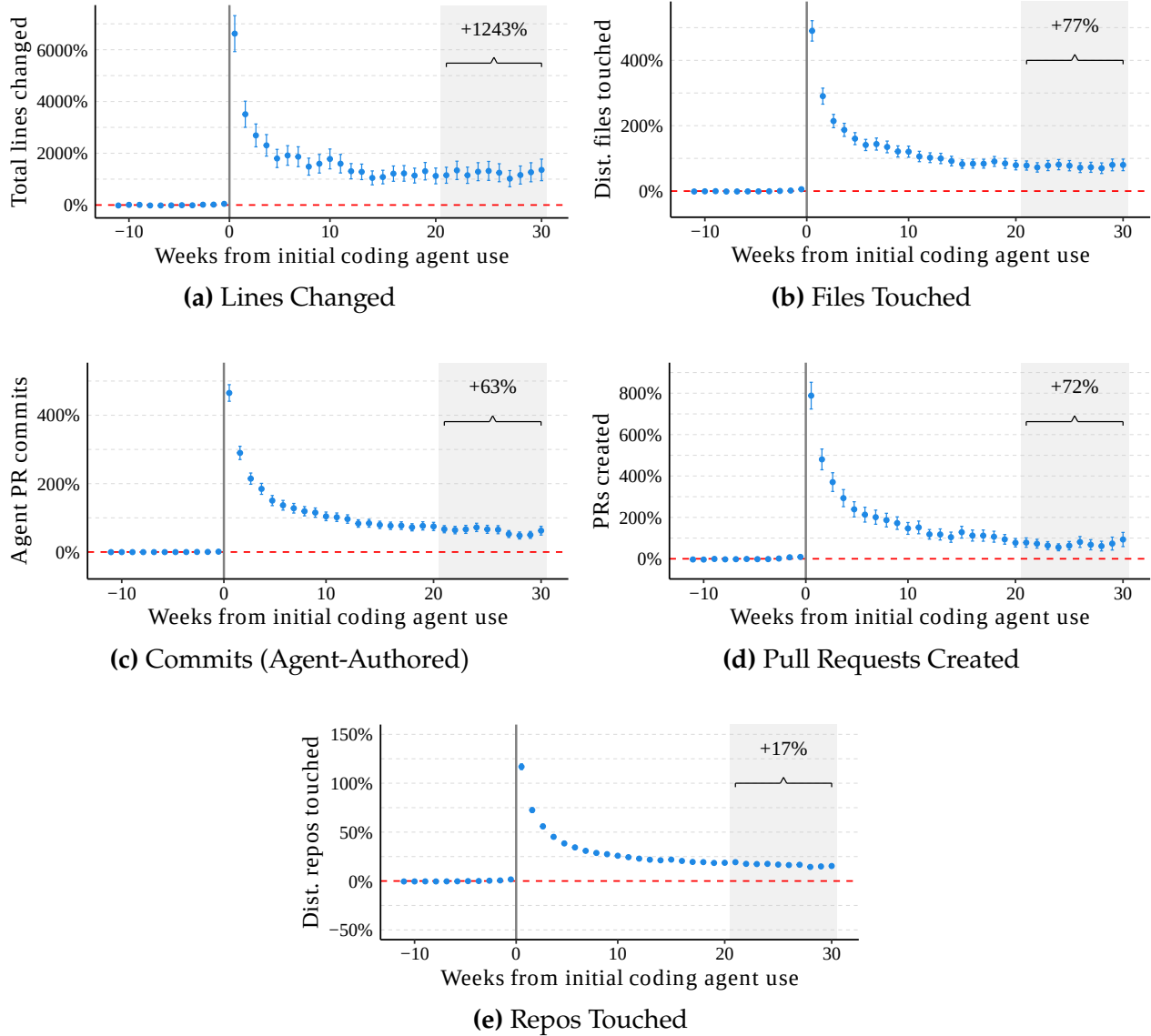
Figure OA-10: Productivity Effects Across the Production Hierarchy (Codex Async)
