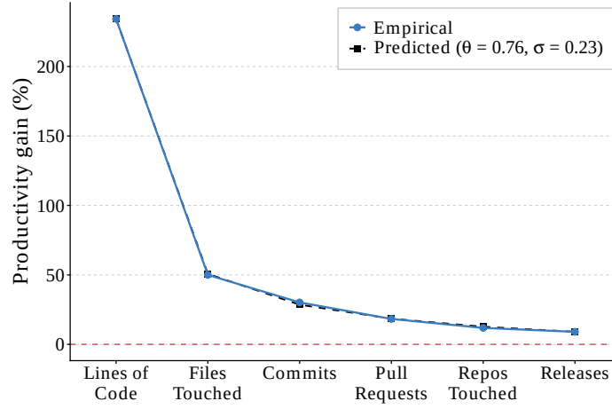
Figure 8: Calibrated Model Fit for Autocomplete
