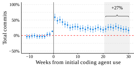
(a) Contemporaneous control: Autocomplete
