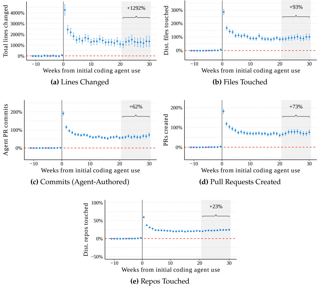
Figure OA-9: Productivity Effects Across the Production Hierarchy (GitHub Agent Async)
