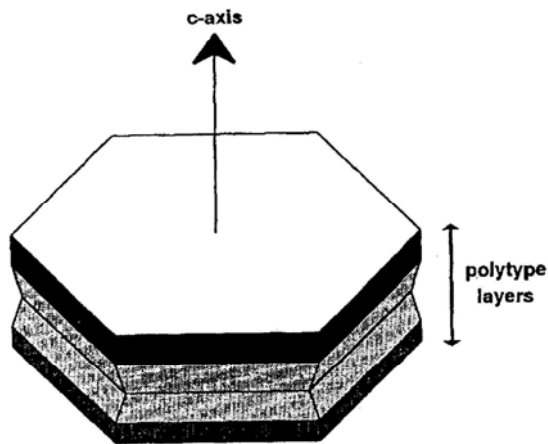
Figure 2. Crystals of SiC grown by the modified Lely technique form hexagonal platelets varying in thickness from about 100 \mu m up to approximately 3mm containing various combinations of polytypes parallel to the crystallographic c-axis as illustrated. The exact locating of these individual polytype layers and their immediate neighbours and intervening regions of disorder has been significantly improved with the advent of synchrotron edge topography schematically depicted in Figure 3.
