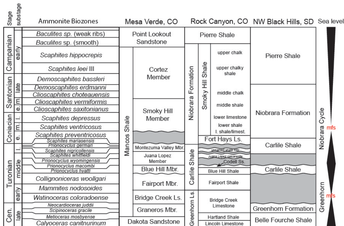
Figure 4. Summary of ammonite biozones, representative stratigraphic sections different regions of the study area, and broad sea level trends. Ammonite biozonation displayed is after Leckie et al. (1997) and
