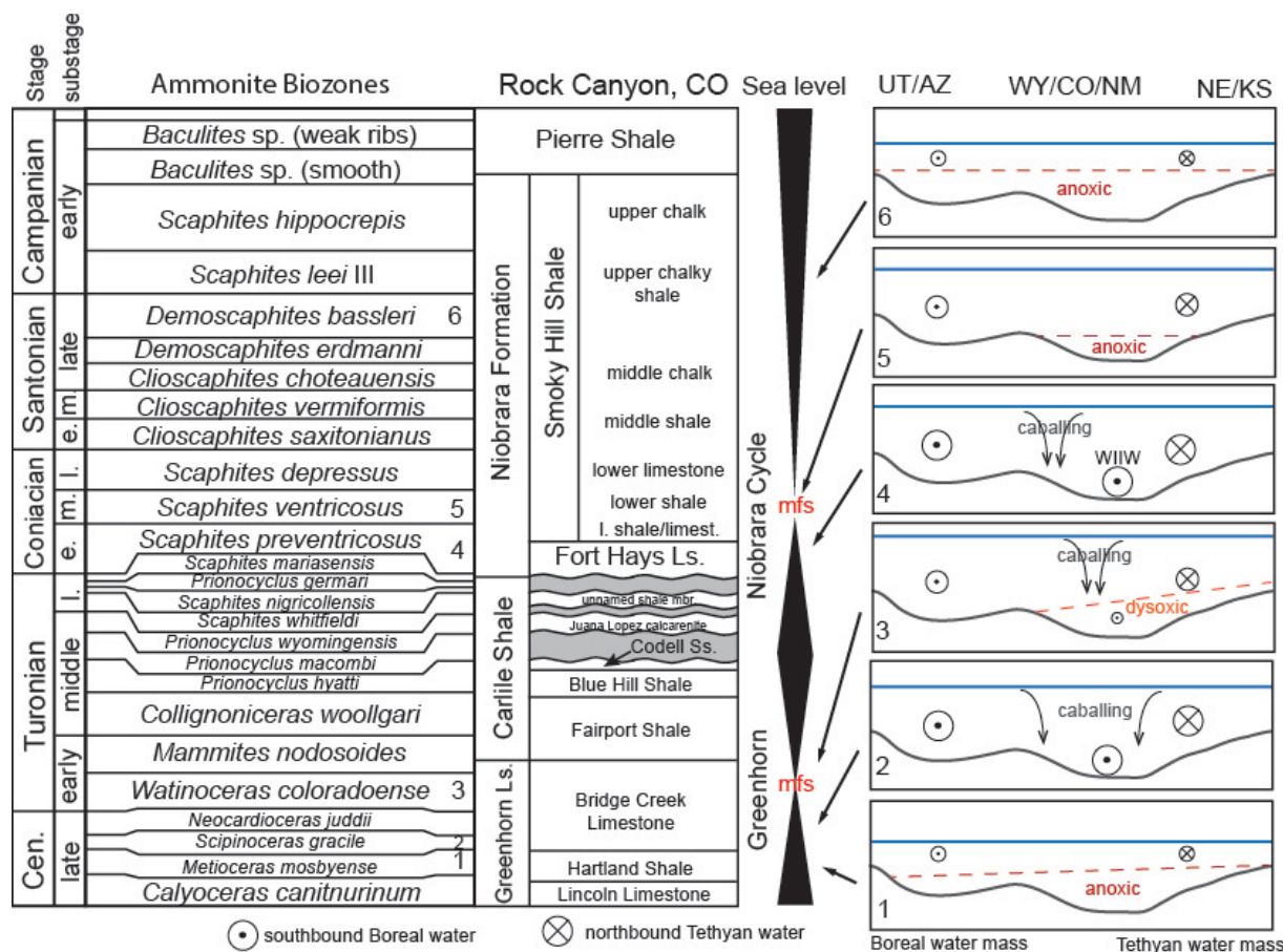
Figure 8. Conceptual model of the relationship between sea level and oxygen in the Western Interior Sea along an east-west transect. When sea level is high, mixing water masses along an oceanographic front in the central axis of the seaway results in a downwelling of a third water mass that exports oxygen to the seafloor. As sea level falls the amount of oxygen exported to the seafloor declines, and eventually falls below benthic oxygen demand, anoxia develops on the seafloor. Numbers in the ammonite biozones correspond to respective boxes summarizing conditions during those time intervals.
