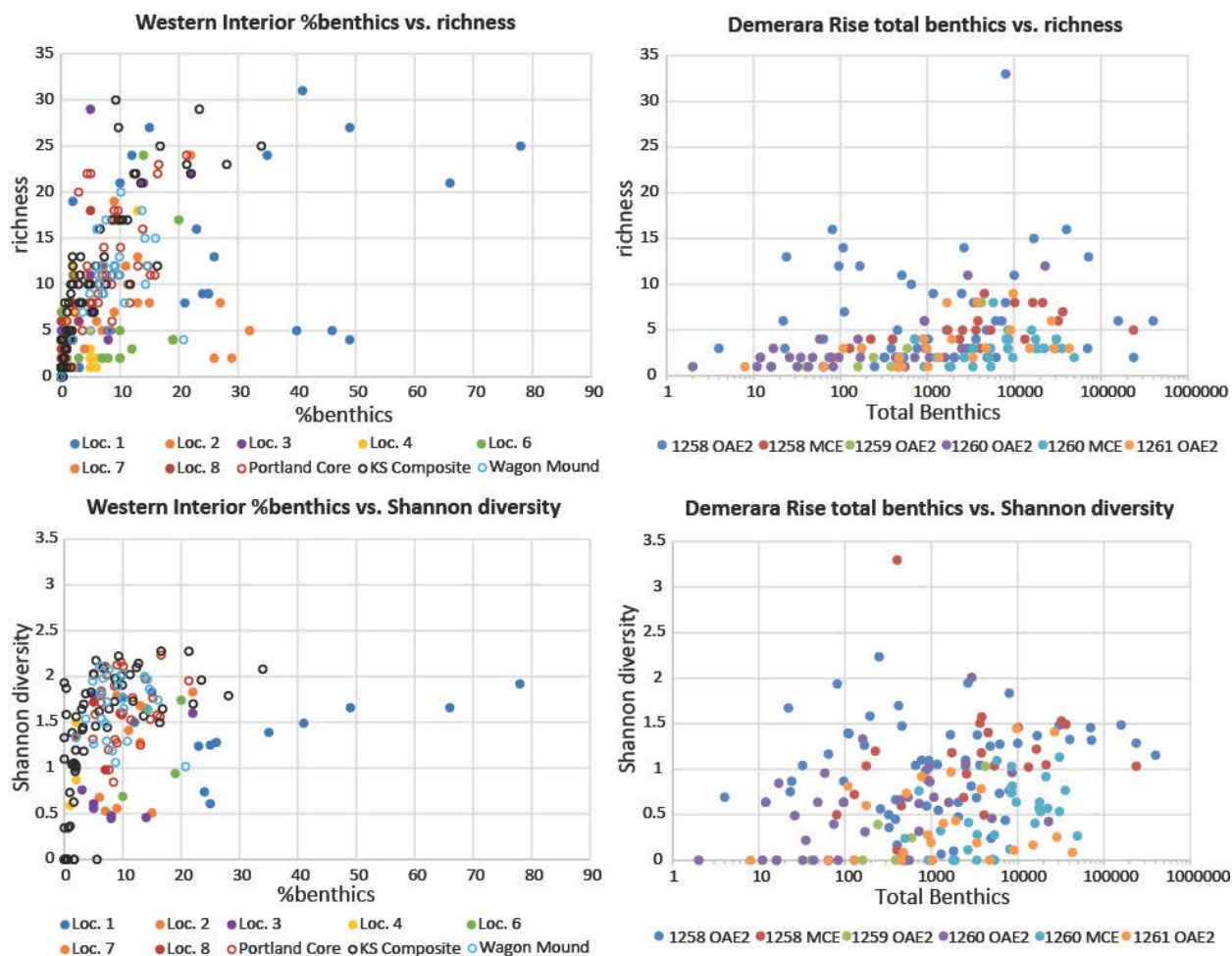
Figure 5. Cross plots of benthic foraminiferal abundance with benthic richness (top) and Shannon diversity (bottom) in the Western Interior (left) and Demerara Rise (right). Western Interior data primarily comes from the Greenhorn cycle sites of Eicher and Worstell (1970; their Localities 1-8, with the exception of Loc. 5, which did not include benthic foraminifera diversity data) and the Niobrara interval of the Portland Core (Lowery et al., 2017a). Demerara data from the Mid-Cenomanian Event (MCE) at ODP Sites 1259 and 1260 (Friedrich et al., 2009) and OAE2 at ODP Sites 1258, 1259, 1260, and 1261 (Friedrich et al., 2006). Note that while WIS data are plotted against %benthics, lack of planktic foraminiferal counts from the Demerara sites meant that those data had to be plotted against benthics per gram on a log scale.
