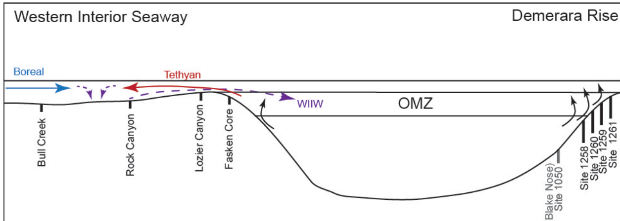
Figure 9. Schematic comparison of oceanography of the WIS with more typical open ocean sites, ODP Sites 1258-1261 (Demerara Rise) and Site 1050 (Blake Nose). The WIS is characterized by two water masses mixing and downwelling and the occasional encroachment of an OMZ during times of high sea level. The mid-depth continental margin sites of Demerara Rise are impinged by an OMZ and constantly sourced with nutrients due to upwelling, and are this highly productive. Blake Nose is a lower bathyal site well below the influence of the OMZ and did not experience anoxia during OAEs.
