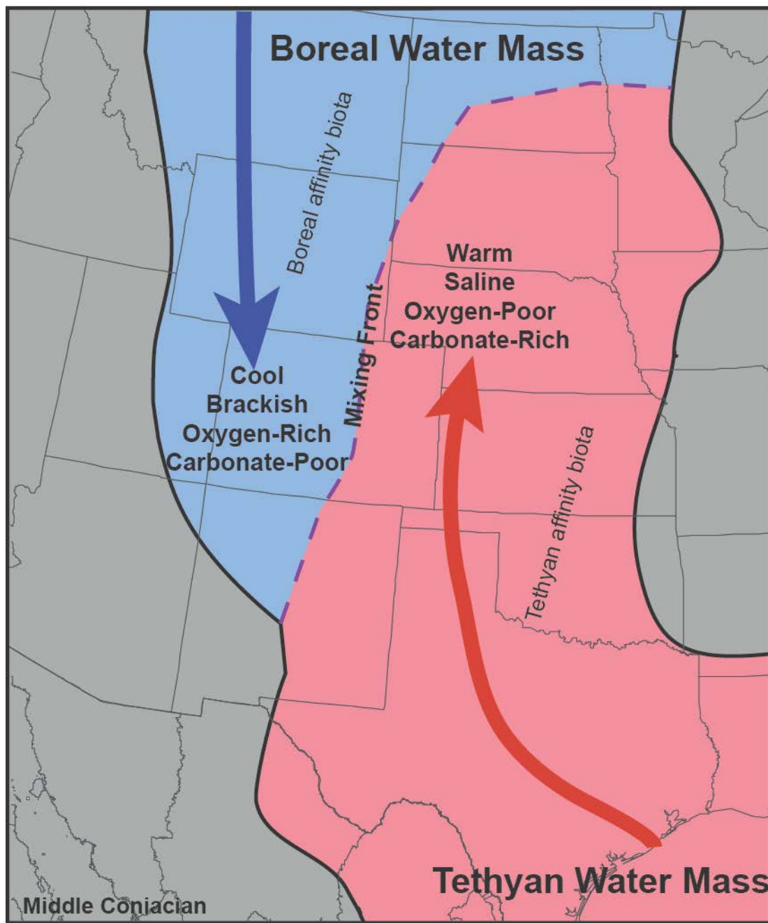
Figure 3. Summary of water mass and circulation in the Western Interior Sea, showing southern-sourced Tethyan water and northern-sourced Boreal water, and the approximate position of the boundary between the two along which mixing occurred. Based on Slingerland et al. (1996), Longman (1998), and Elderbak and Leckie (2016).
