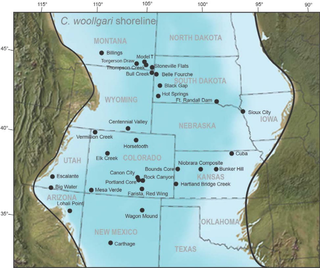
Figure 1. Location Map, showing the 32 total localities used in this study. Paleogeographic map representative of the middle Turonian Colignoceras woollgari Zone cropped from Blakey (2016).
