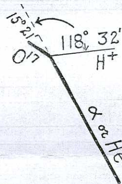
FIG. 2.—The space relations of the synthesis and disintegration exhibited in Fig. 1.
