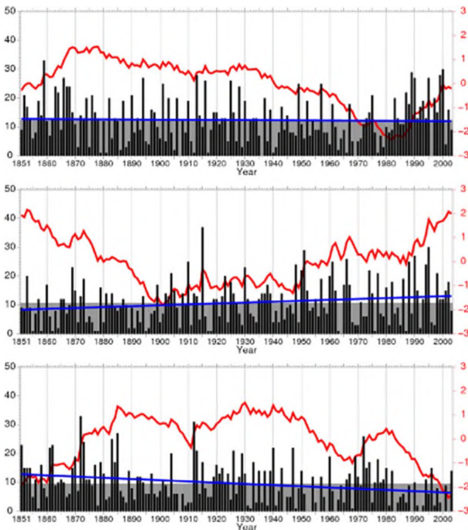
Figure 10. Seasonal frequencies (bars), linear trend (blue line), and normalized cumulative anomalies (red line), for the circulation types shown in Figure 9. The long term mean is indicated in gray. Cumulative anomalies indicate periods of prevailing positive/negative anomalies by sections of line increase/decrease.
