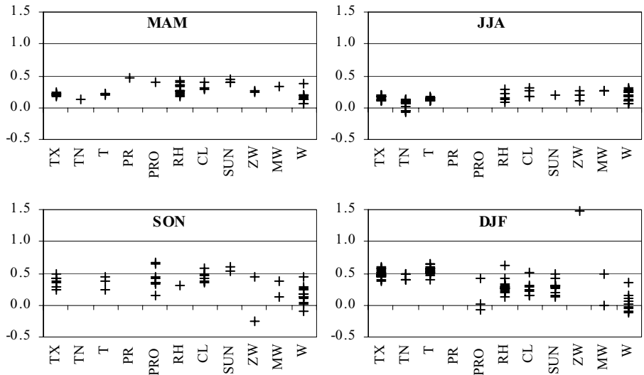
Figure 17. Ratio of “hypothetical” (from changes in the frequency of Hess–Brezowsky circulation types; see text) and observed seasonal trends at stations in the Czech Republic (1961–1998); only the values for the observed trends significantly different from zero are shown. TX, TN, T are maximum, minimum, and mean temperature, respectively; PR, PRO are precipitation amount and occurrence, respectively; RH, relative humidity; CL, cloudiness; SUN, sunshine duration; ZW, MW, W are zonal and meridional wind components and wind speed, respectively. (In color in Annals online.)
