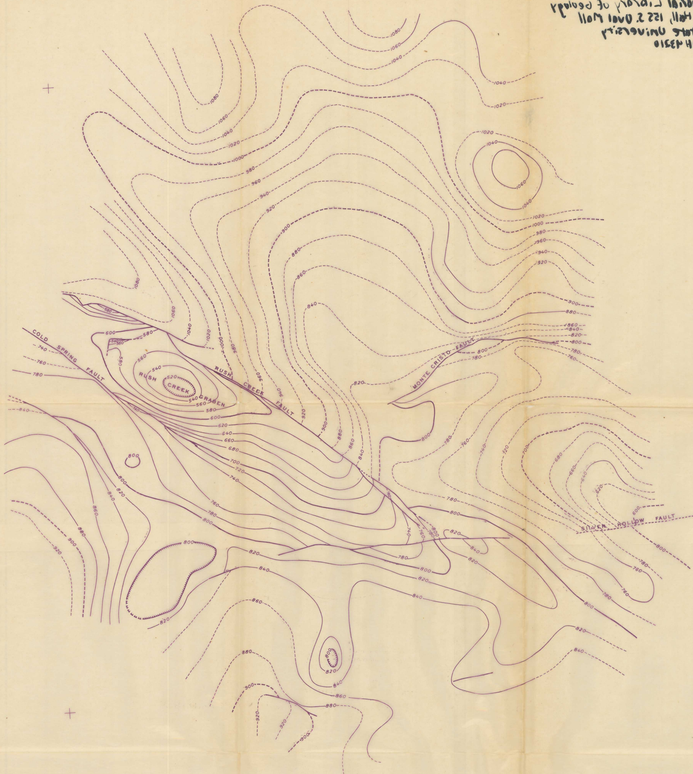
STRUCTURE CONTOURS ON BASE OF ST. JOE LIMESTONE IN RUSH DISTRICT, MARION COUNTY, ARKANSAS
