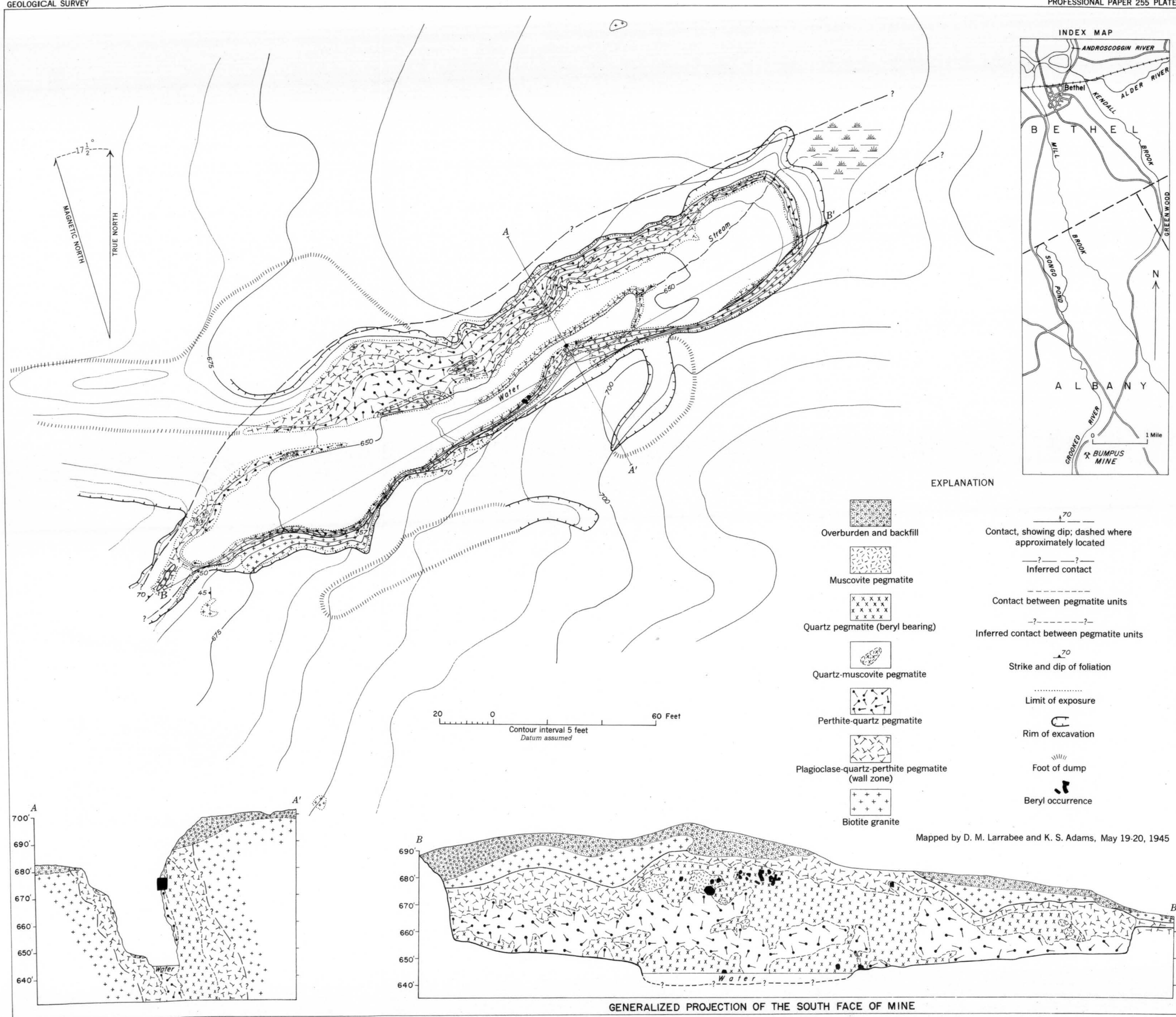
GEOLOGIC MAP AND SECTIONS OF THE BUMPUS FELDSPAR QUARRY, ALBANY, MAINE
