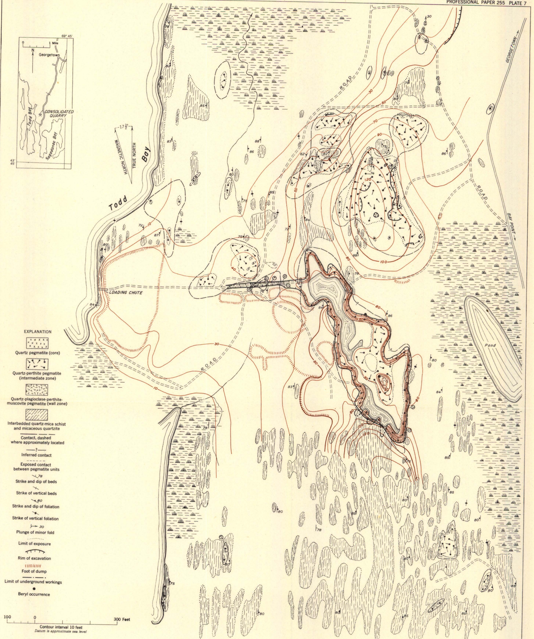
GEOLOGIC MAP OF THE CONSOLIDATED FELDSPAR QUARRY, GEORGETOWN, MAINE
