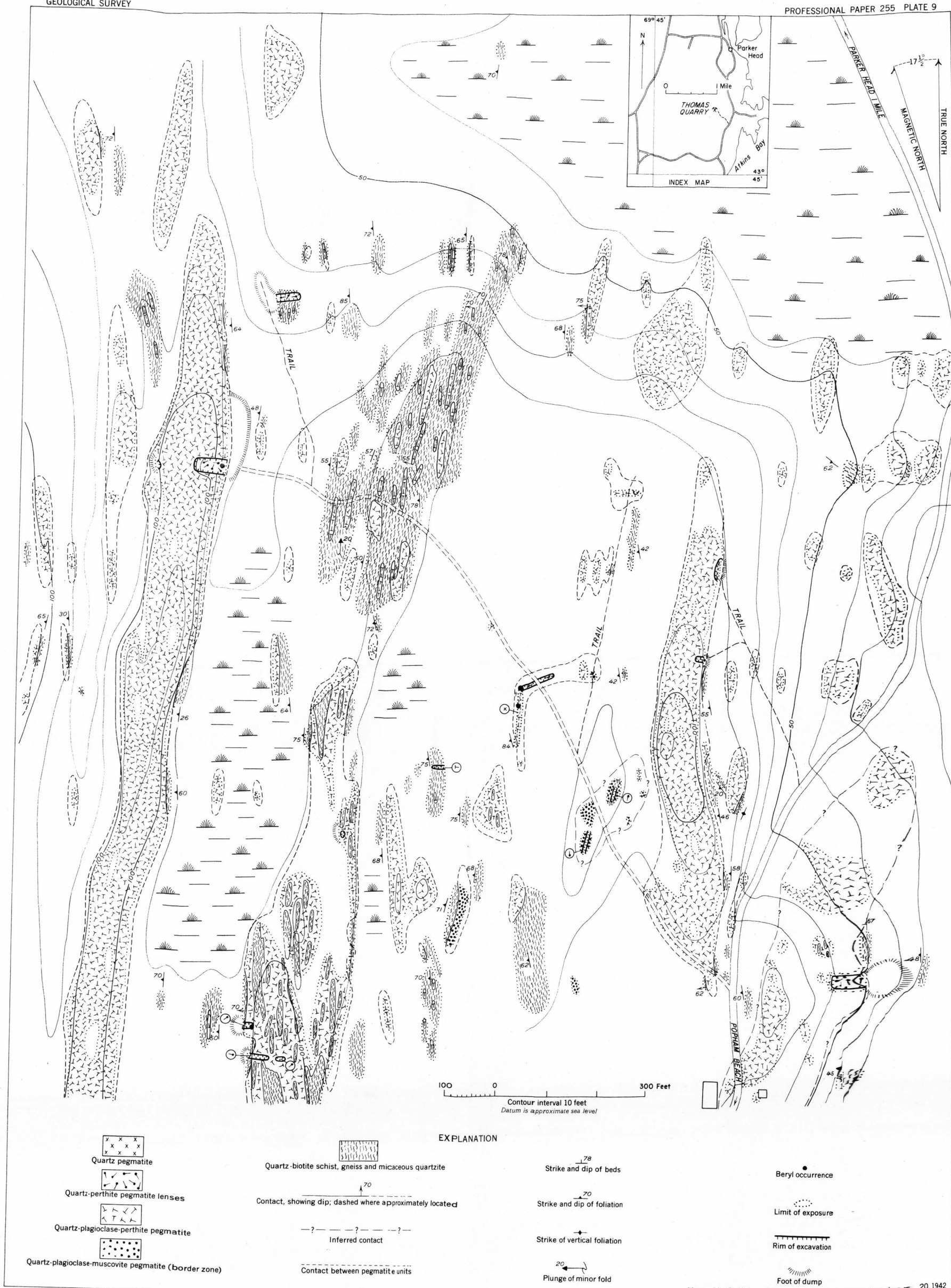
GEOLOGIC MAP OF THE THOMAS FELDSPAR QUARRY, PHIPPSBURG, MAINE
