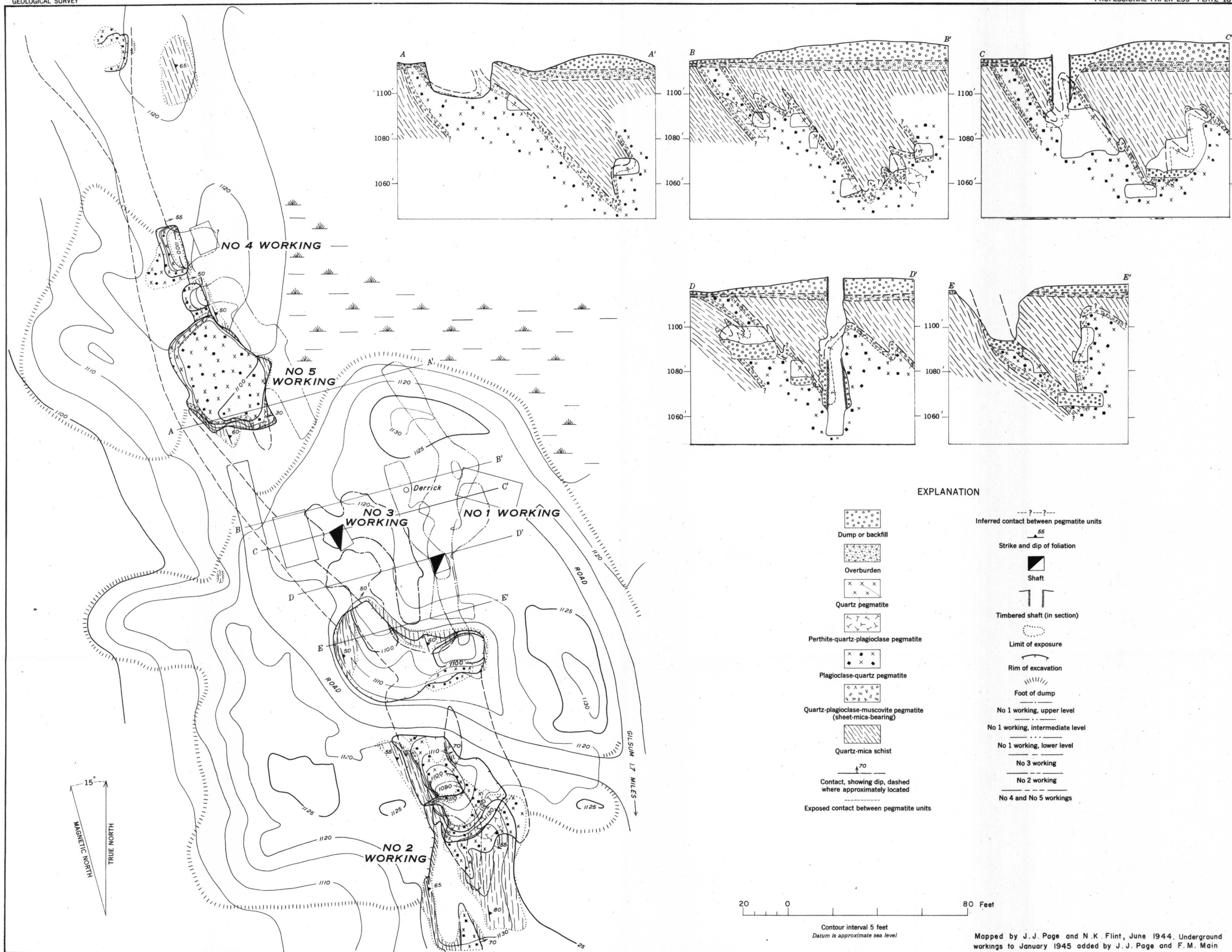
GEOLOGIC MAP AND SECTIONS OF THE NICHOLS MICA MINE, GILSUM, NEW HAMPSHIRE
