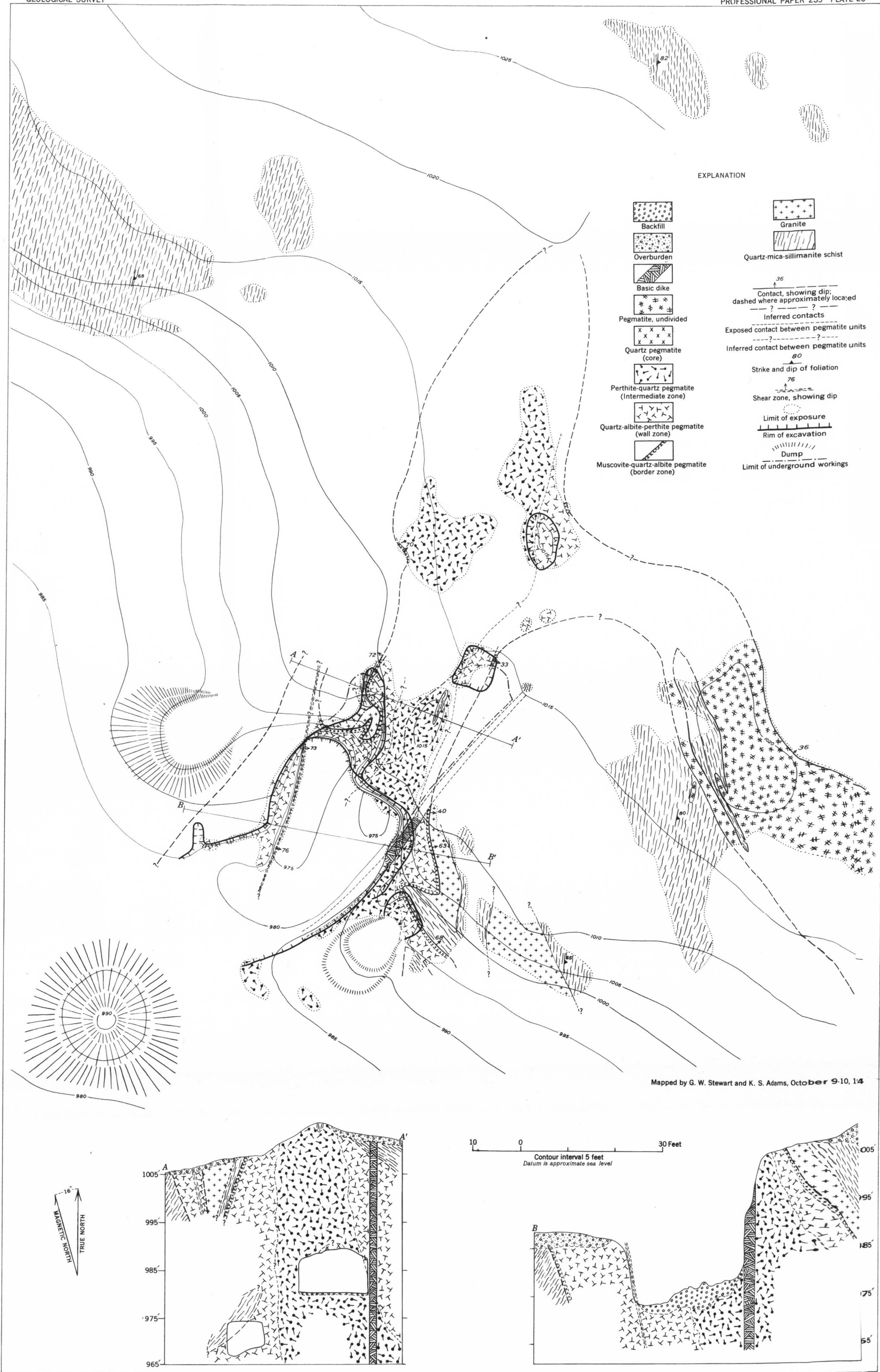
GEOLOGIC MAP AND SECTIONS OF THE BELDEN MICA MINE, RUMNEY, NEW HAMPSHIRE
