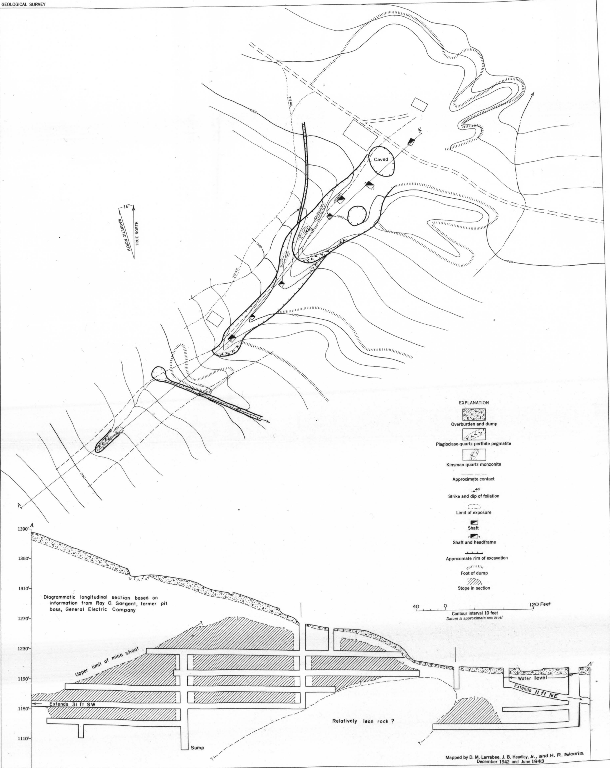
GEOLOGIC MAP AND SECTION OF THE MUD MICA MINE, ALEXANDRIA, NEW HAMPSHIRE
