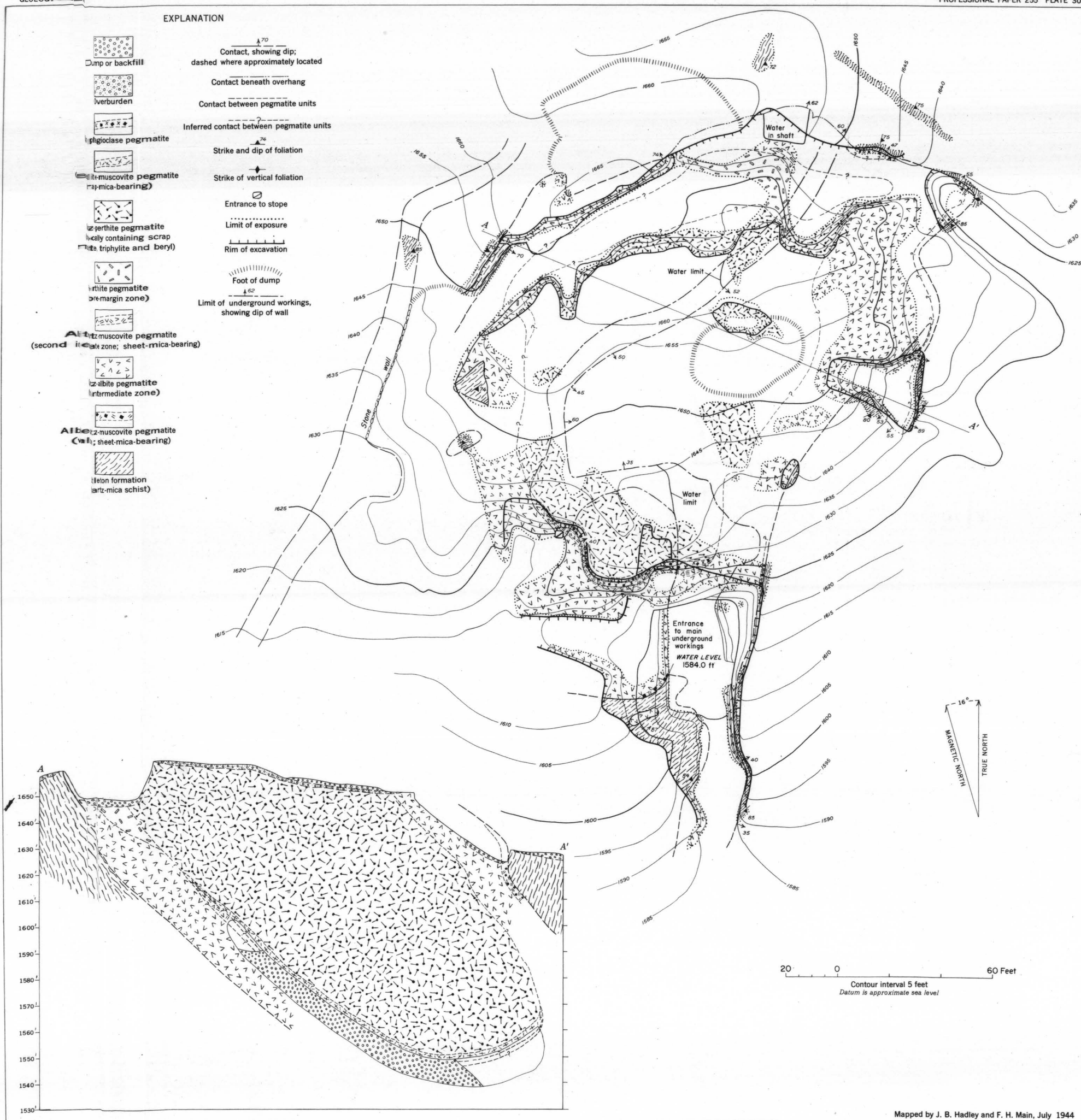
GEOLOGIC MAP AND SECTION OF THE PALERMO MINE NO. 1 (HARTFORD MINE), GROTON, NEW HAMPSHIRE
