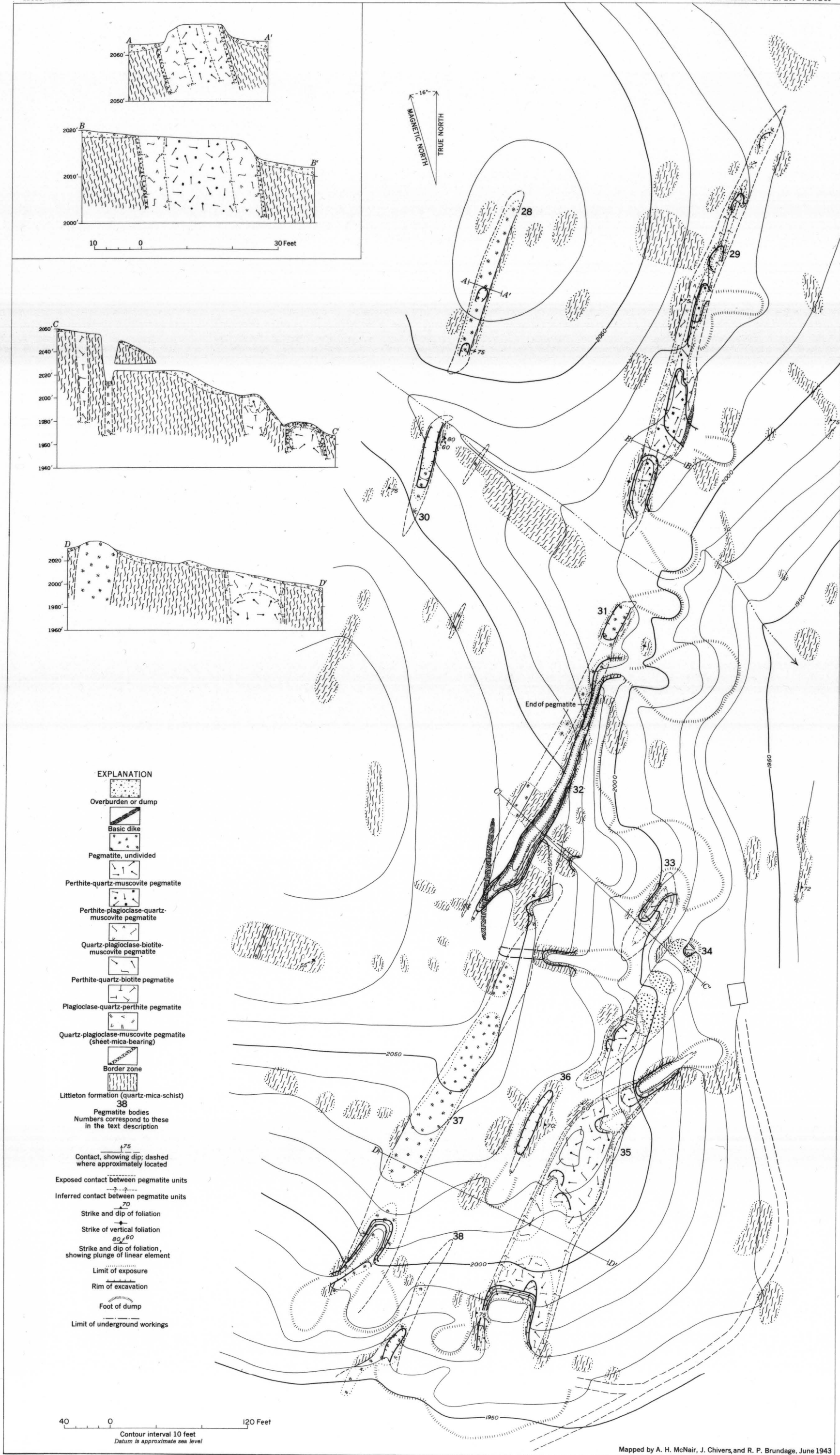
GEOLOGIC MAP AND SECTIONS OF THE RICE MICA MINE, GROTON, NEW HAMPSHIRE
