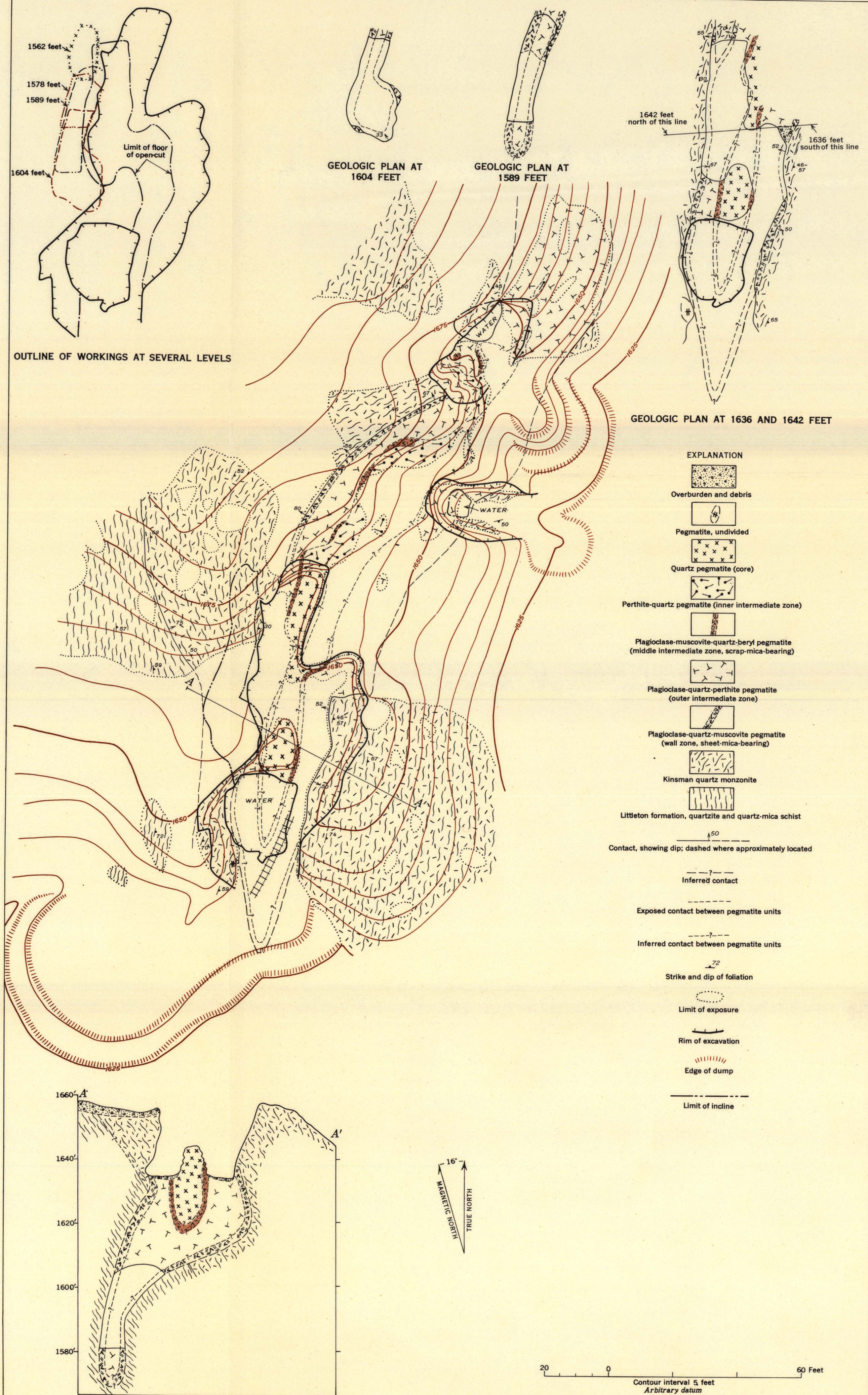
GEOLOGIC MAP, PLANS, AND SECTION OF THE E. E. SMITH MICA MINE (UPPER MINE), ALEXANDRIA, NEW HAMPSHIRE
