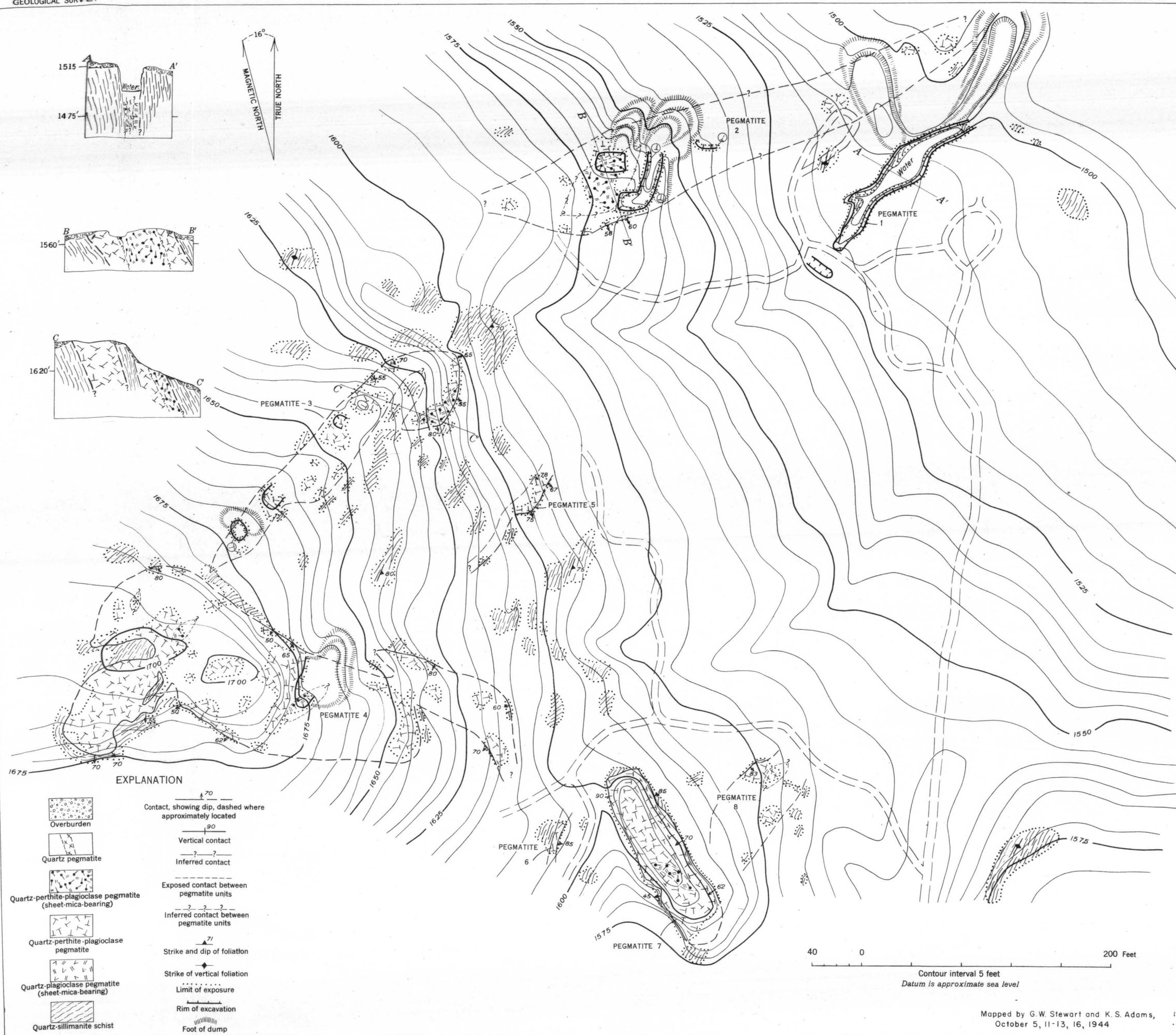
GEOLOGIC MAP AND SECTIONS OF THE UNION MICA MINE AND PROSPECTS, GROTON, NEW HAMPSHIRE.
