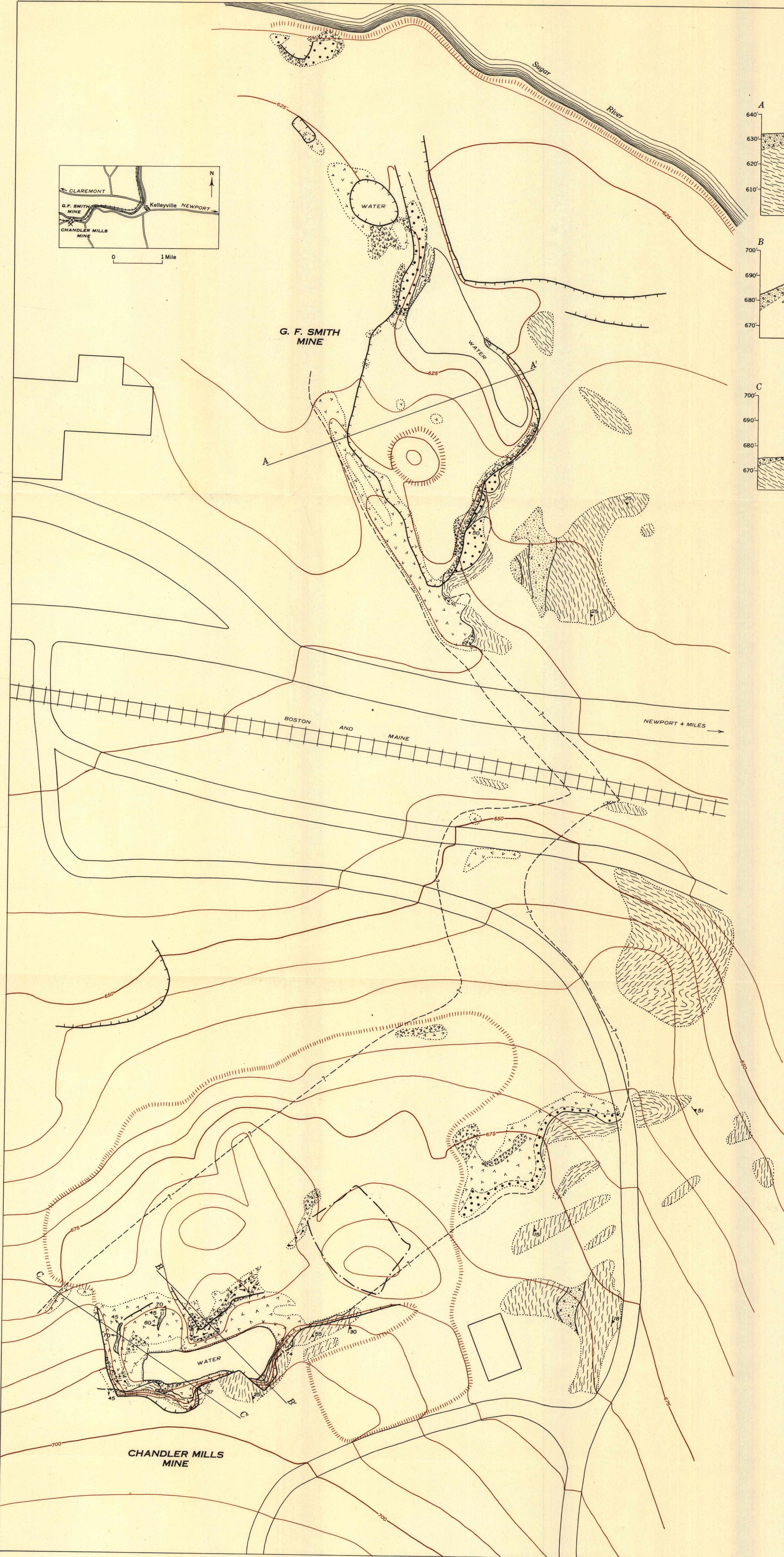
GEOLOGIC MAP AND SECTIONS OF THE G. F. SMITH AND CHANDLER MILLS MICA MINES, NEWPORT, NEW HAMPSHIRE
