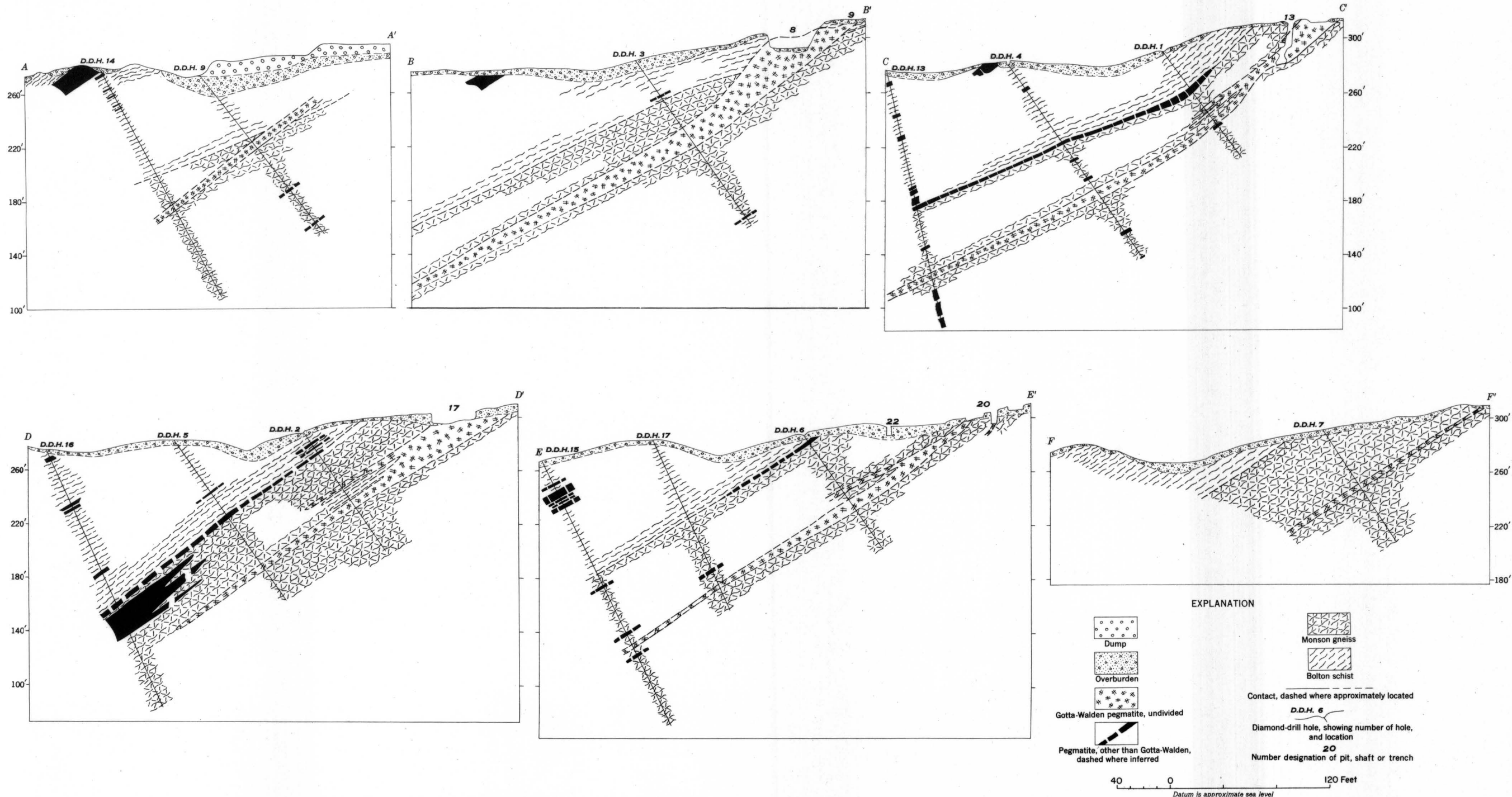
SECTIONS OF THE GOTTA-WALDEN BERYL-MICA PROSPECT, PORTLAND, CONNECTICUT 255298-4/a
