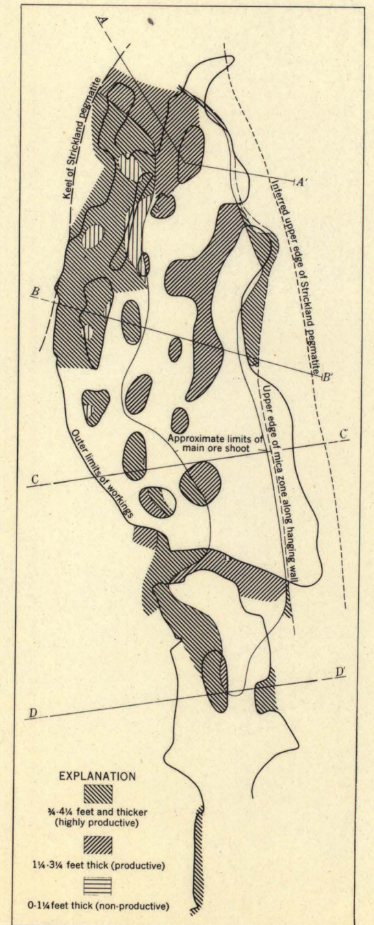
ISOPACH MAP OF PART OF THE MICA ZONE ALONG HANGING WALL OF STRICKLAND PEGMATITE
