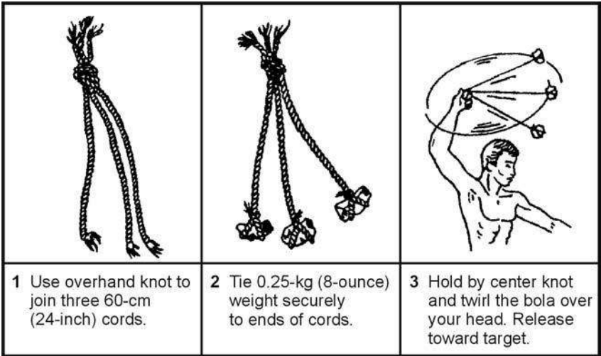
Figure 12-7. Bola
