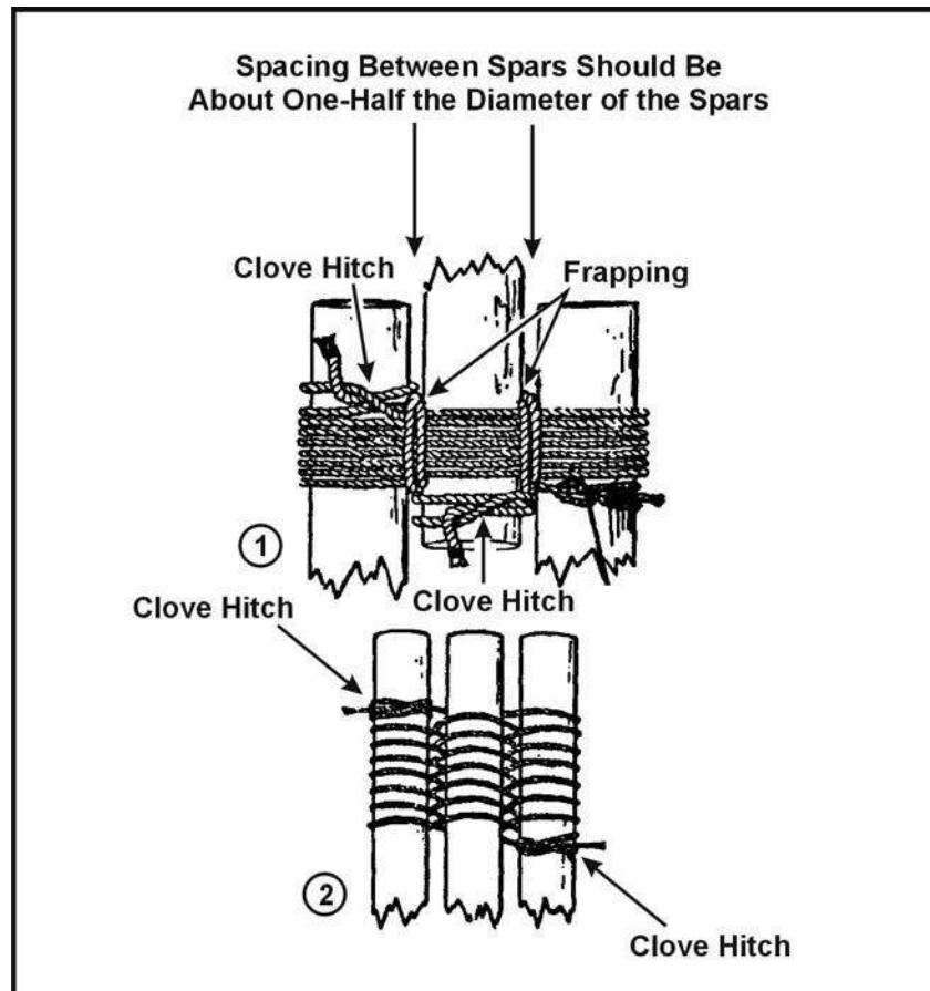
Figure G-16. Tripod Lashing
