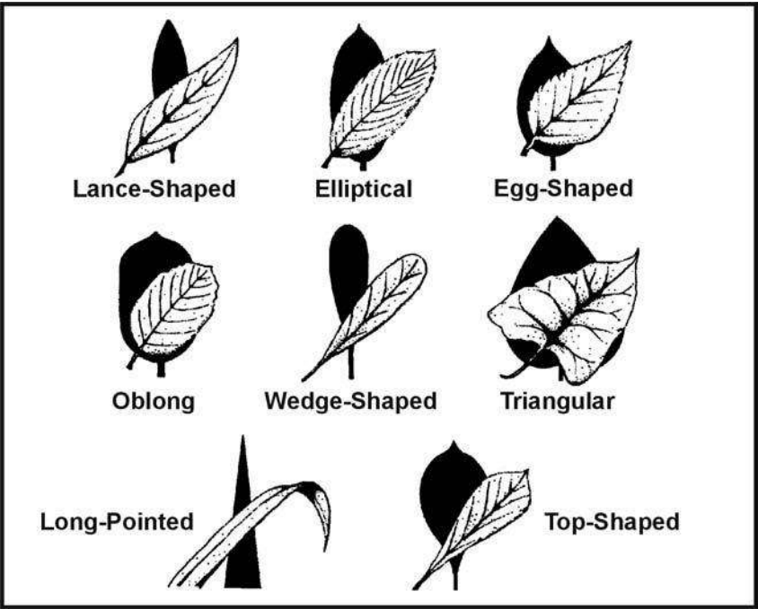
Figure 9-2. Leaf Shapes
