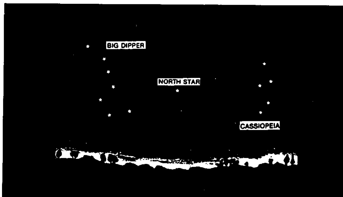
Figure 2-3. Big Dipper.
