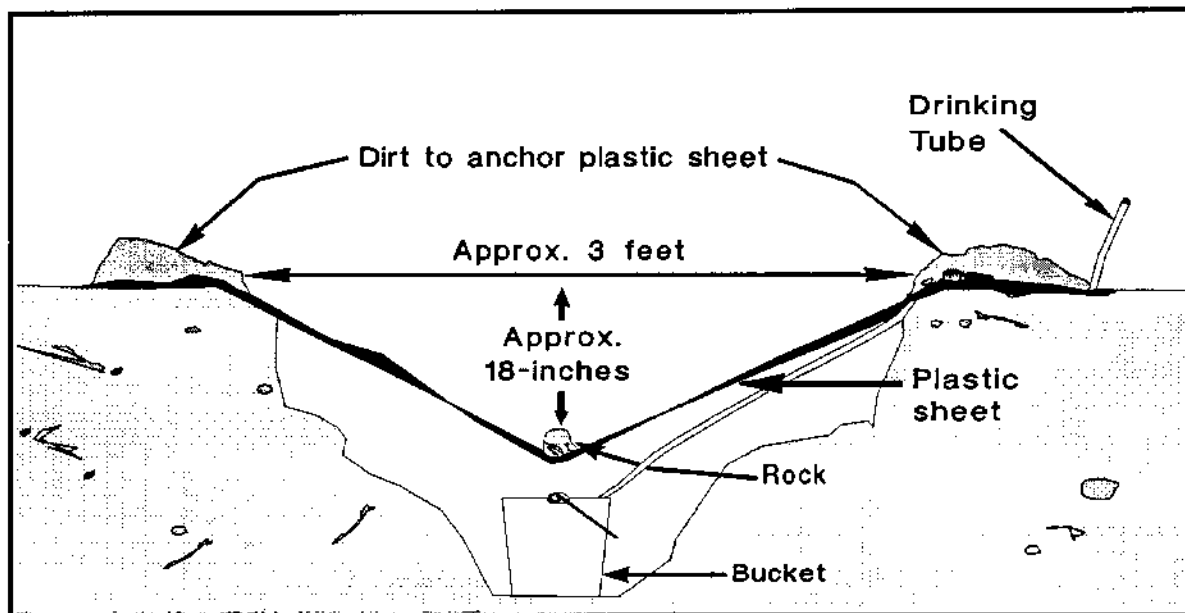
Figure 1-15. Cross-section of a survival still.
