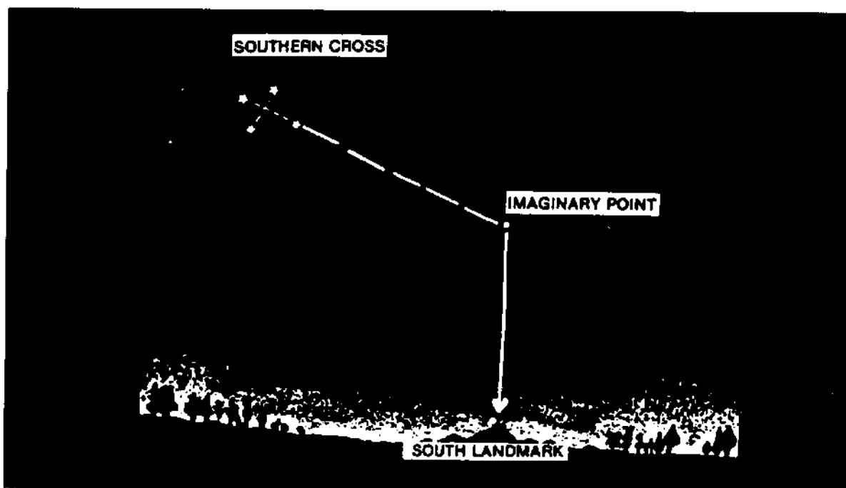
Figure 2-4. Southern Cross.
