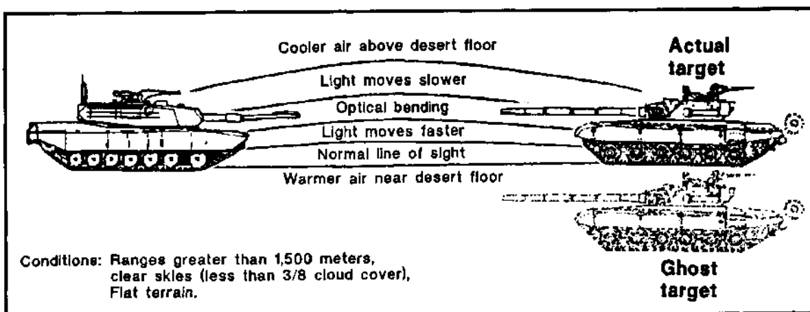
Figure 1-18. Day refraction.
