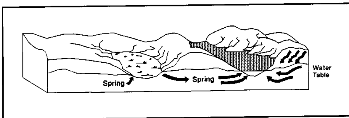
Figure 1-13. Water tables.
