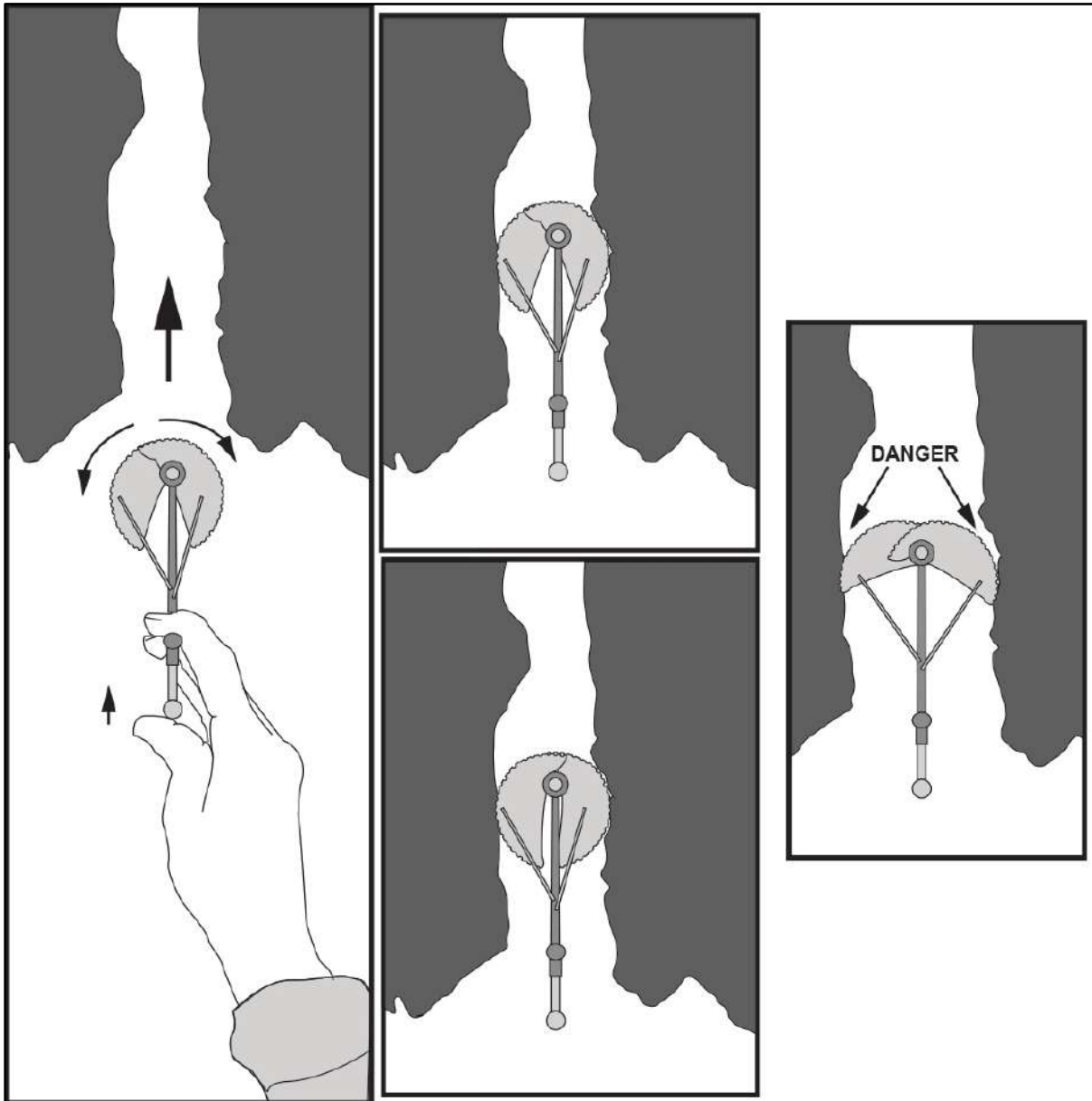
Figure 9-20. Spring-loaded camming device placement
