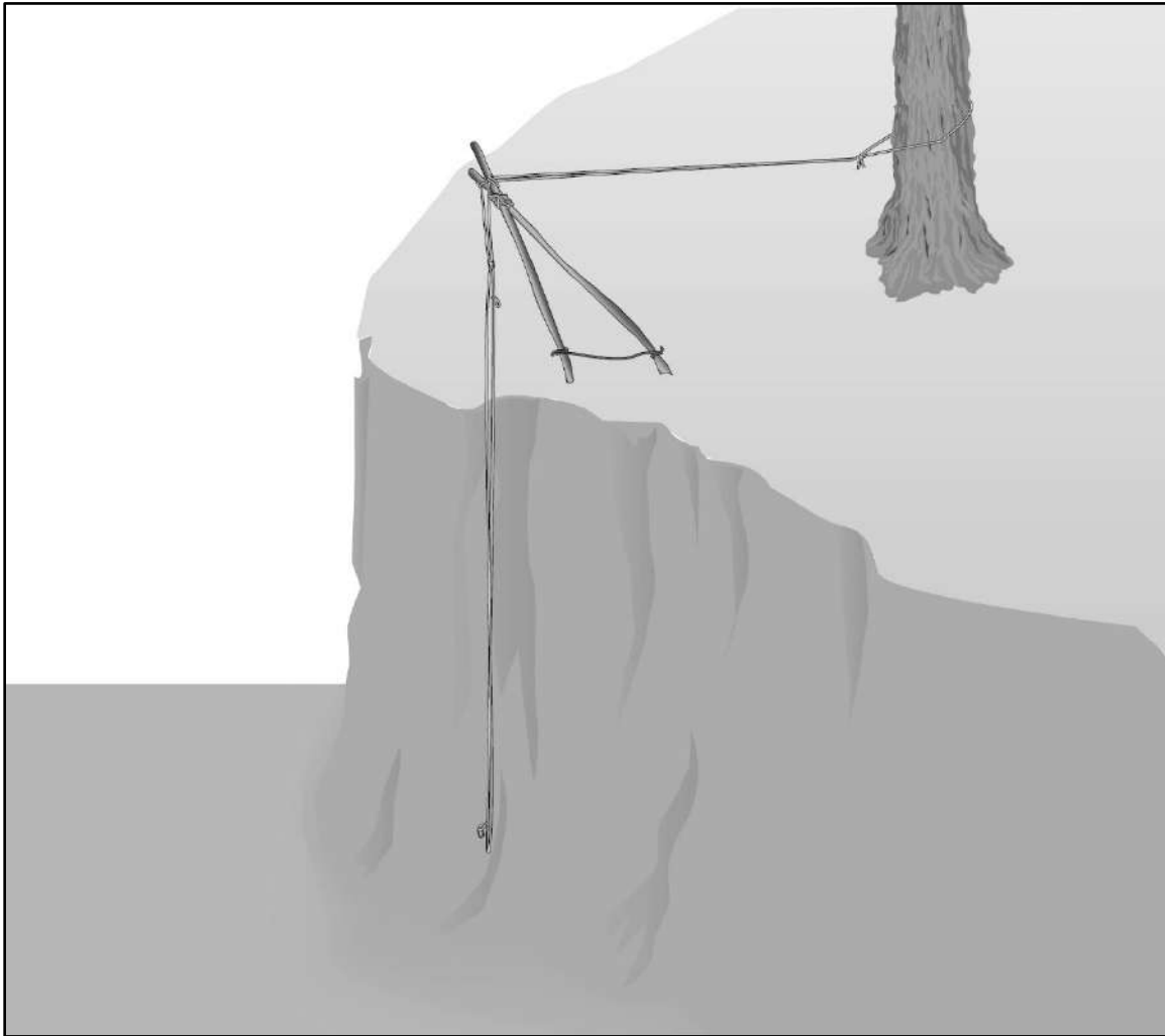
Figure 12-10. Vertical haul line
