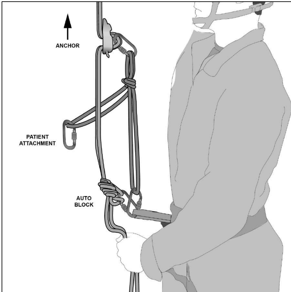
Figure 15-3. Tandem rappel rigging
