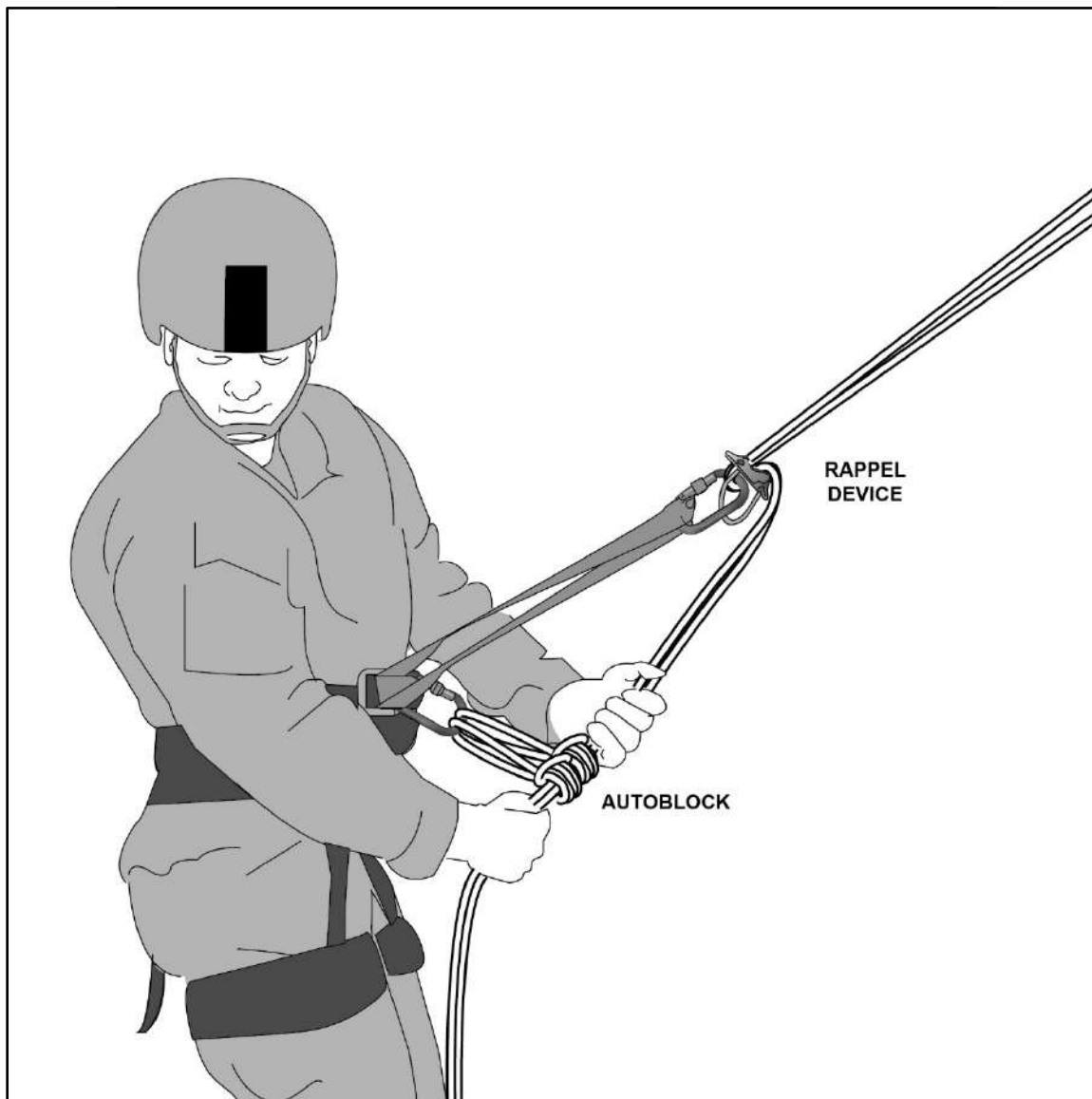
Figure 11-14. Extended device and hands-free break
