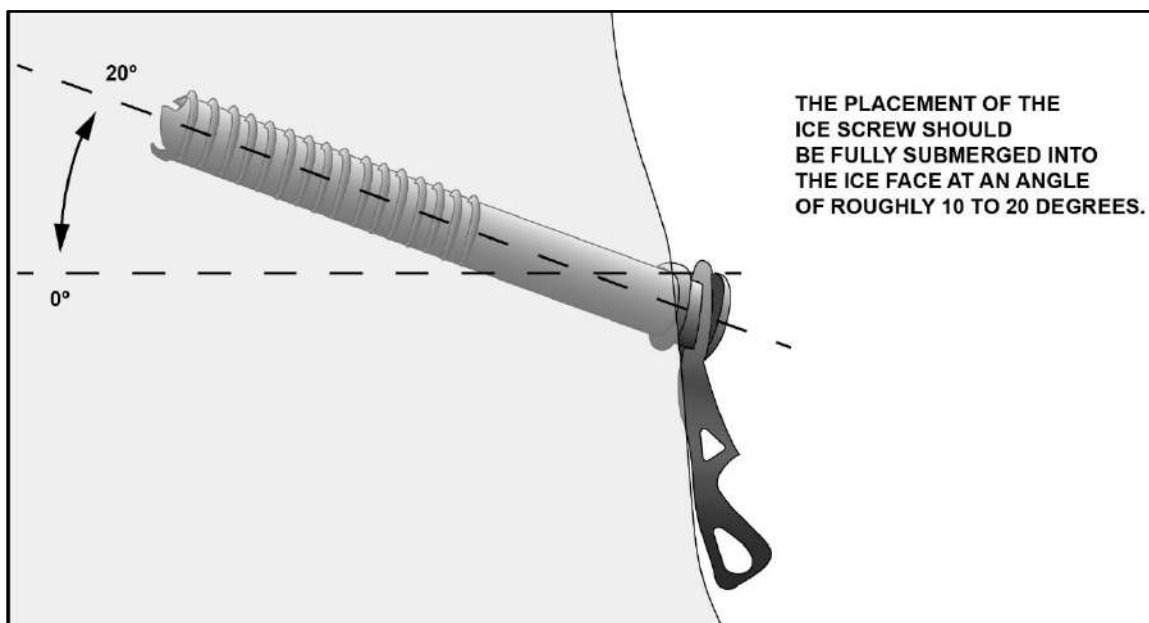
Figure 9-25. Ice screw placement
