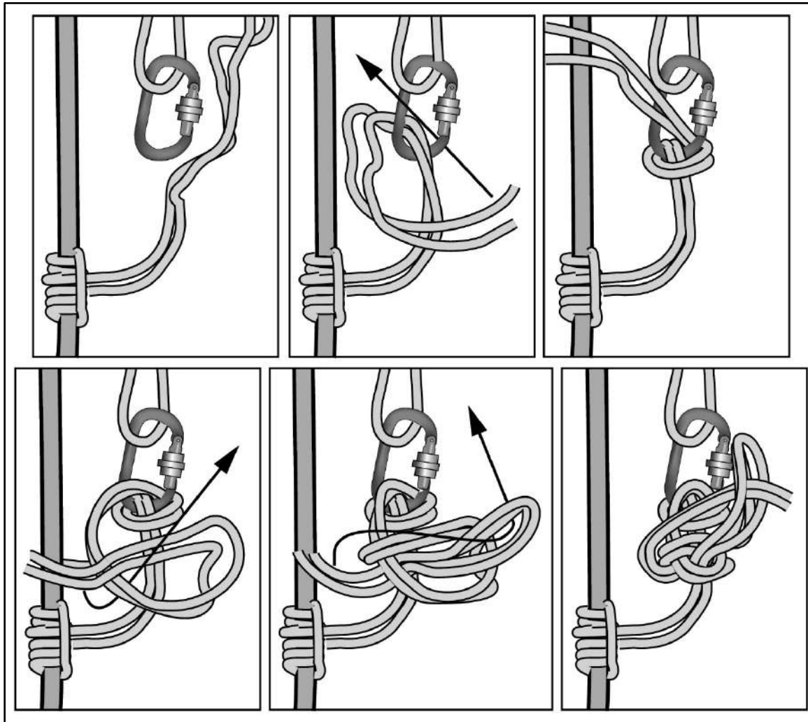
Figure 8-32. Munter mule knot using cord
