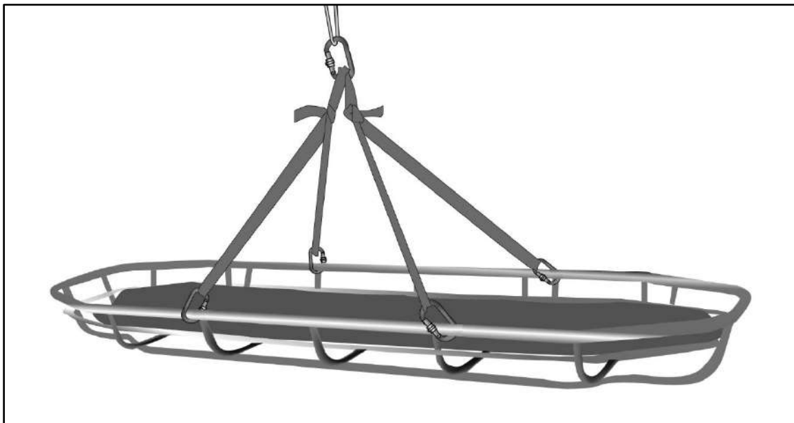
Figure 15-9. Basket litter rigged for horizontal orientation
