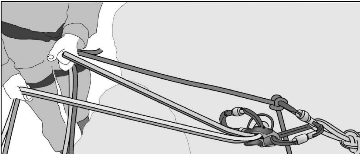
Figure 10-26. Belaying two climbers with an autolocking device
