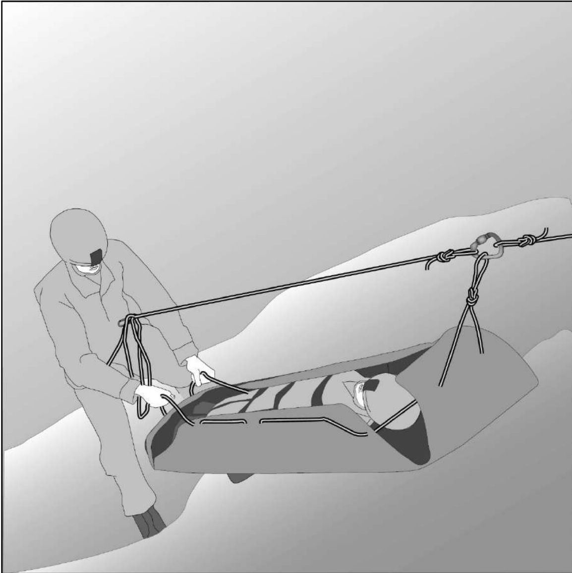
Figure 15-7. Litter rigged for lowering with long-tailed bowline and attendant attached
