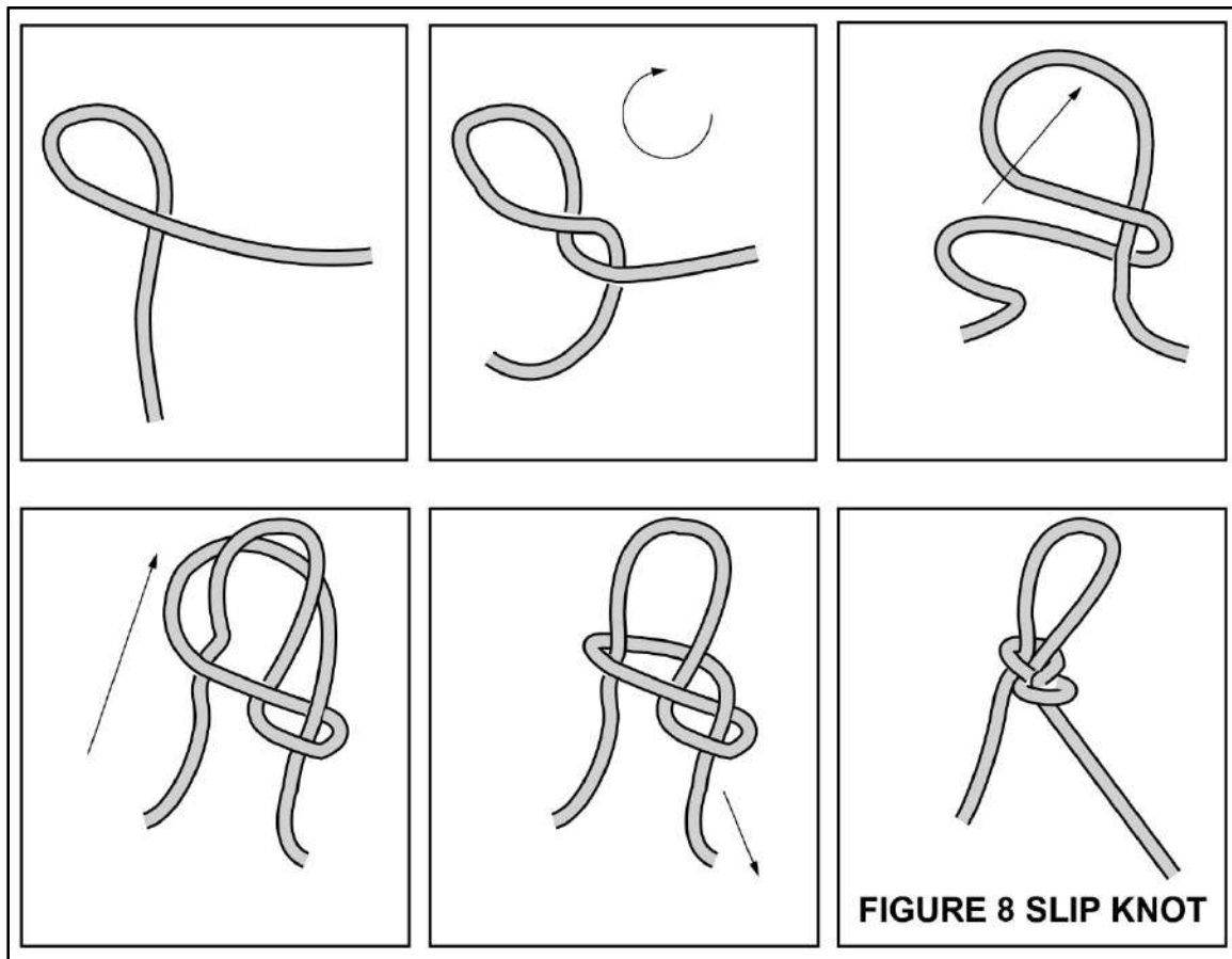
Figure 8-8. Figure-eight slip knot
