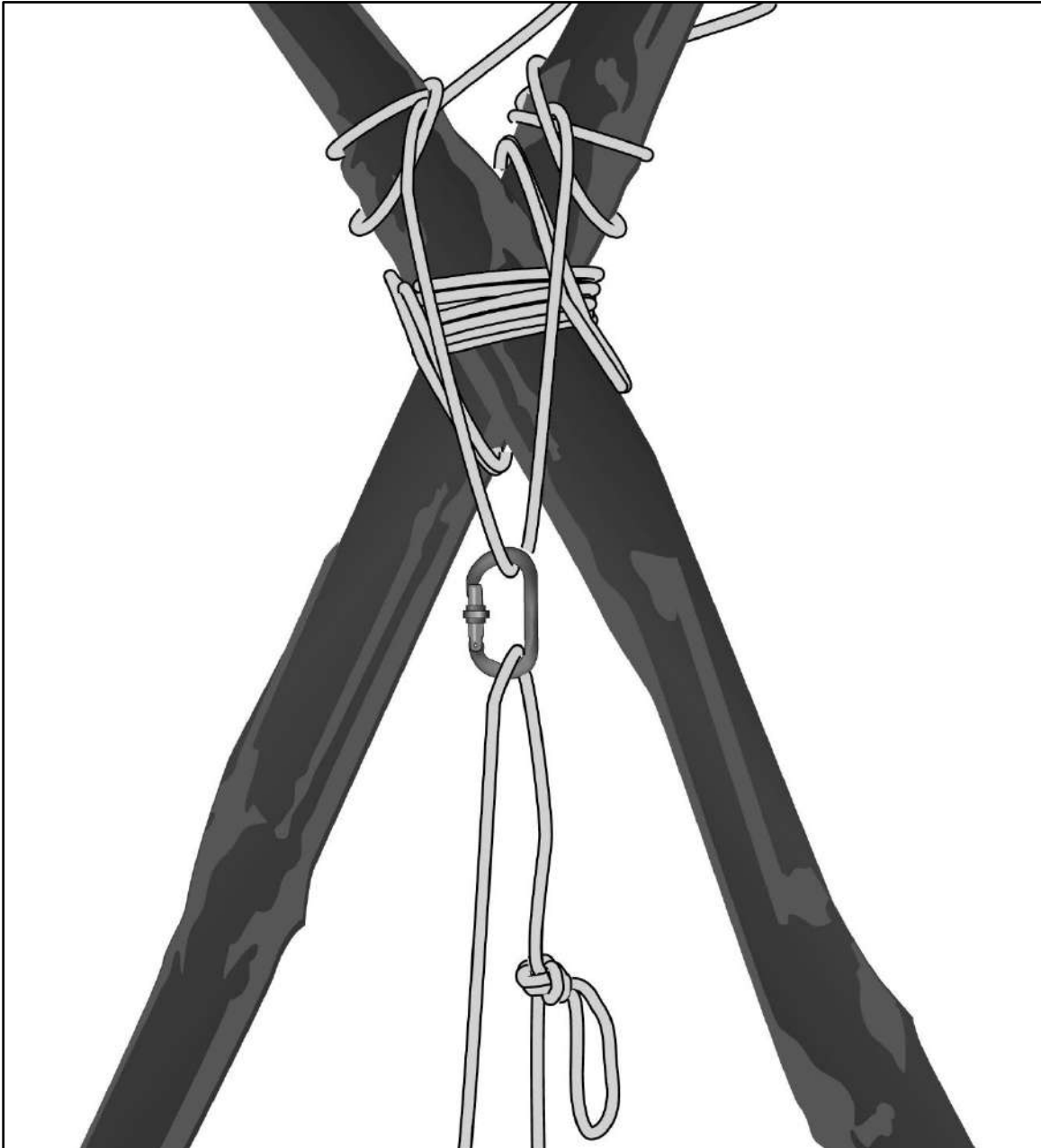
Figure 12-11. A-frame or master point
