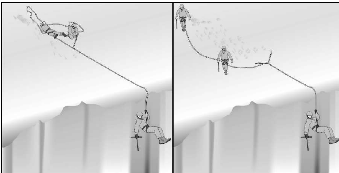
Figure 14-11. Construct the anchor and transfer the load
