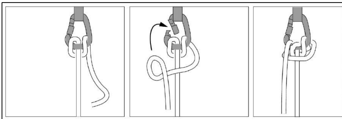
Figure 8-31. Super Munter hitch
