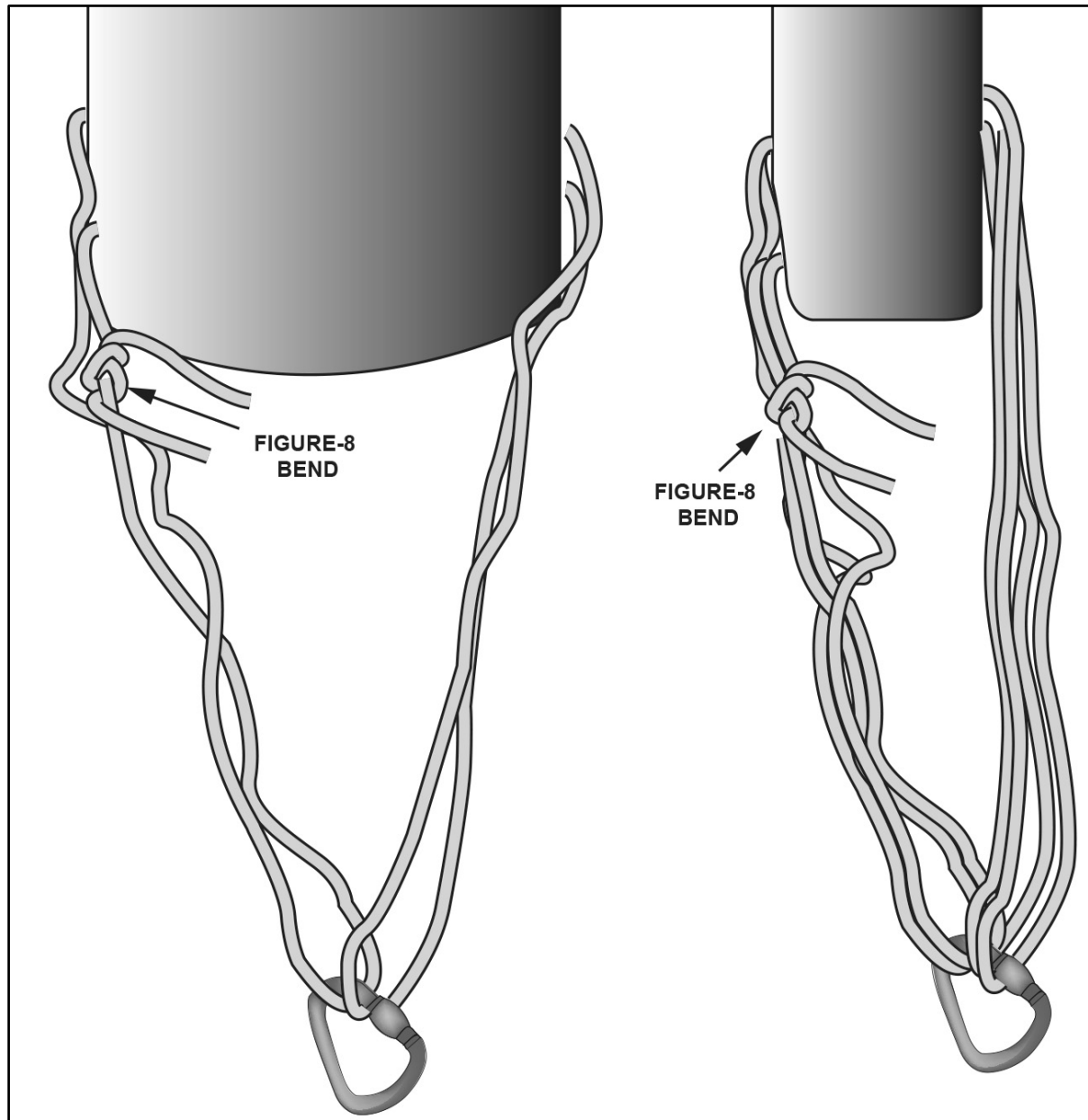
Figure 9-3. Single and double basket hitch
