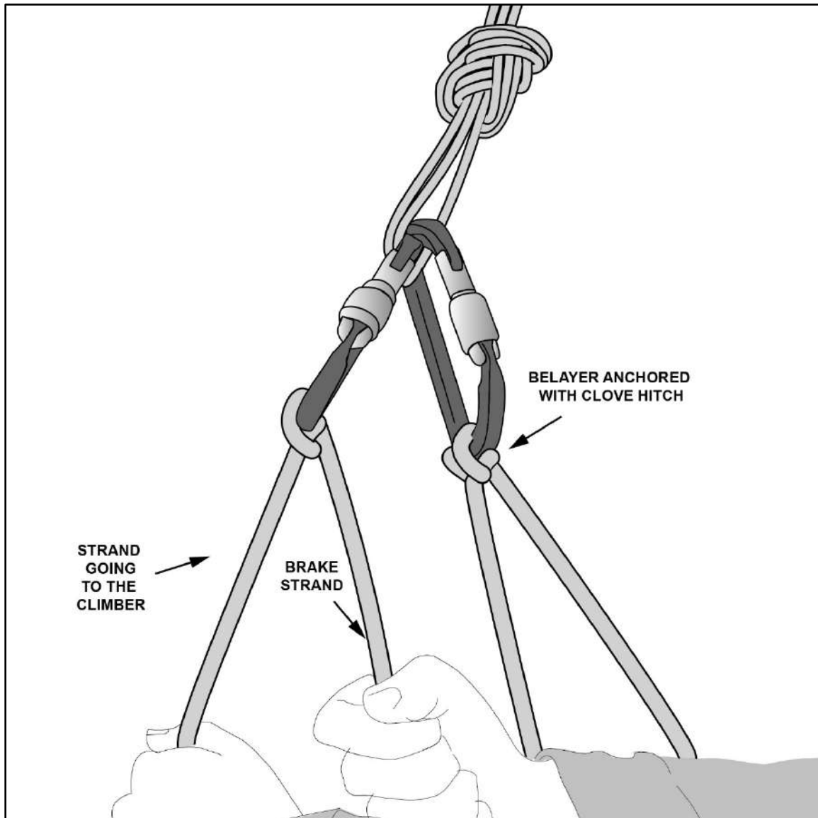
Figure 10-19. Belaying using a Munter hitch
