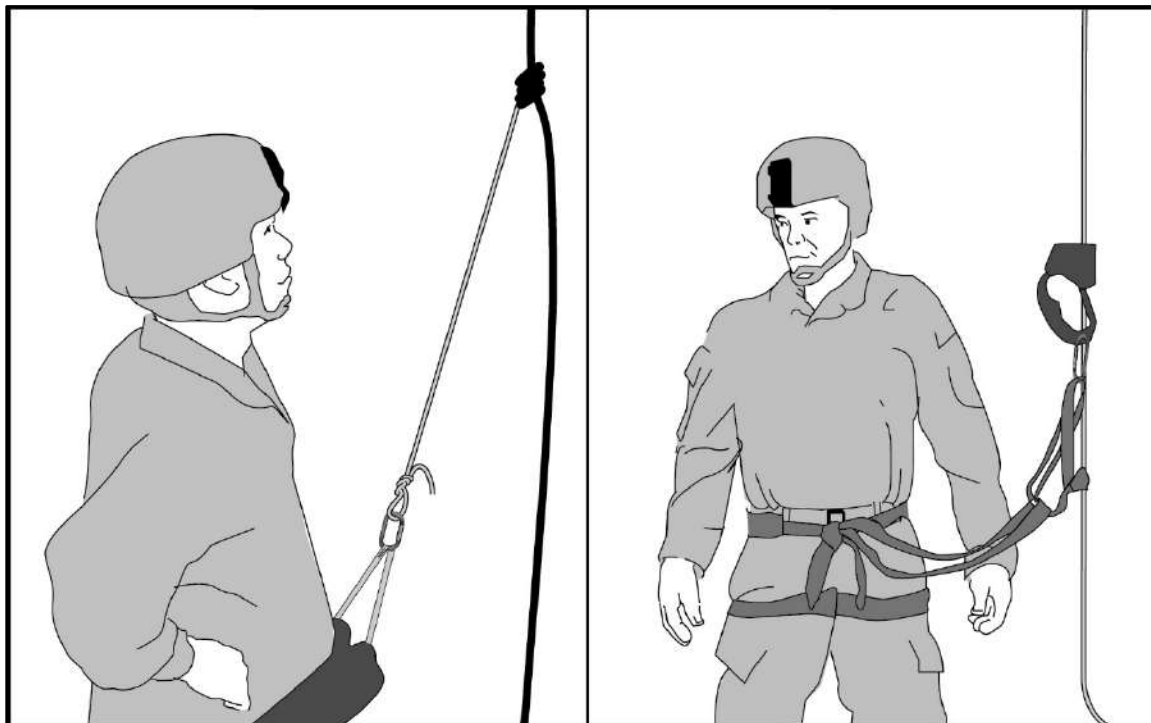
Figure 11-2. Simple fixed-rope attachments in moderate terrain
