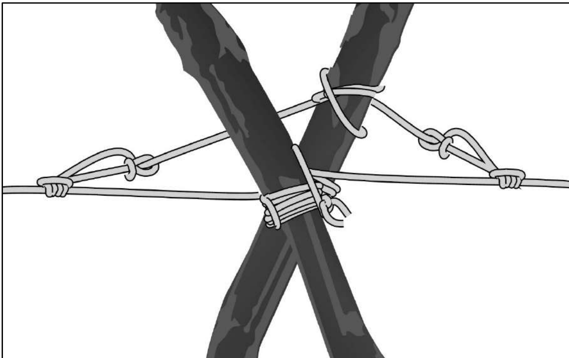
Figure 16-9. Anchoring the A-frame to the installation rope
