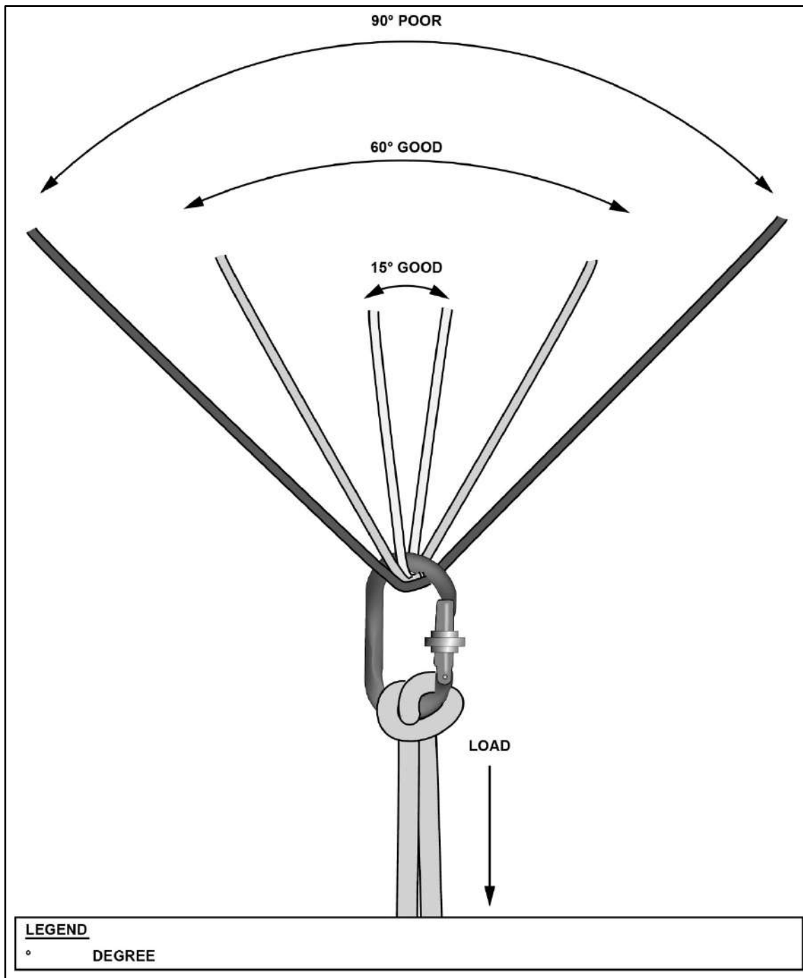
Figure 9-5. Ideal angle required between anchor points to reduce force
