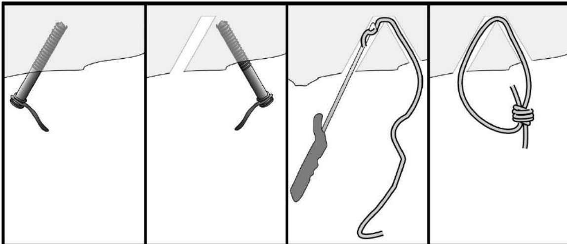
Figure 9-27. Constructing a V-thread anchor
