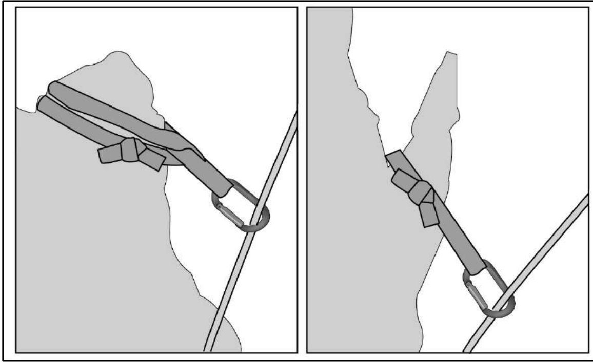
Figure 9-10. Boulders and protrusions used as anchors
