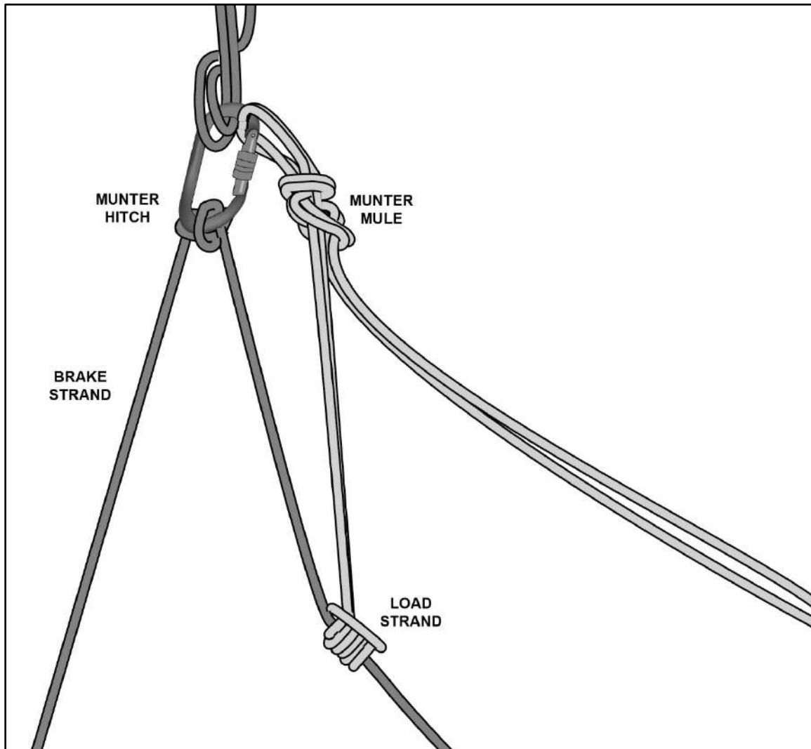
Figure 12-16. Friction hitch on load strand (releasable)
