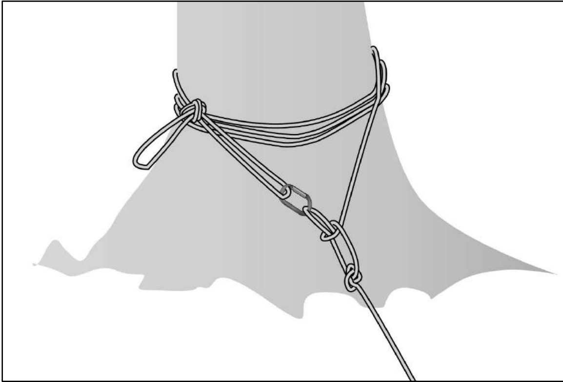
Figure 16-3. Round turn around anchor and two half hitches on a bight
