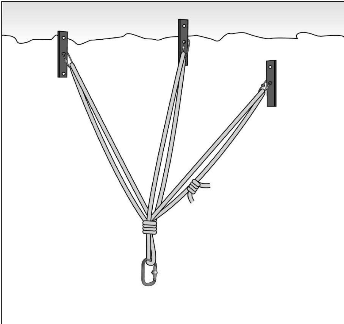
Figure 9-30. Multipoint snow anchor
