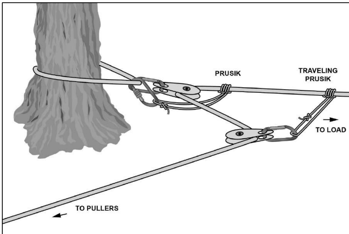
Figure 12-4. Simple 3:1 hauling system
