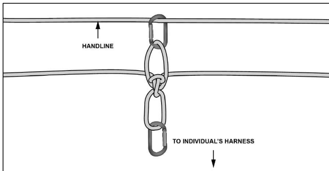
Figure 13-4. Belay with handline
