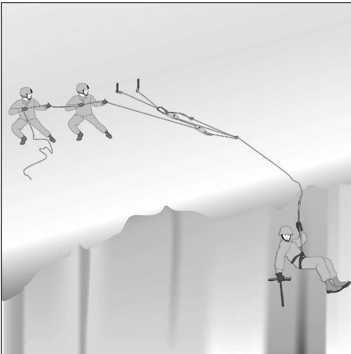
Figure 14-12. Direct haul using a 3:1 hauling system
