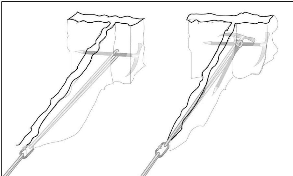
Figure 9-31. Deadman anchor/T-trench anchor in snow with ice axe
