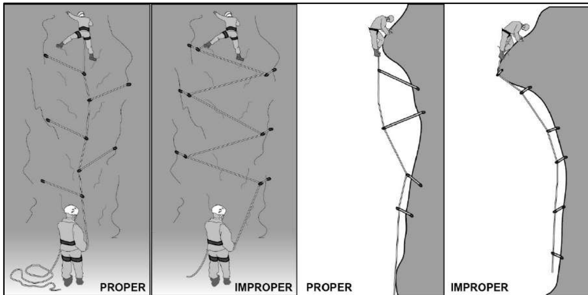
Figure 10-16. Use of runners to extend and reduce rope drag
