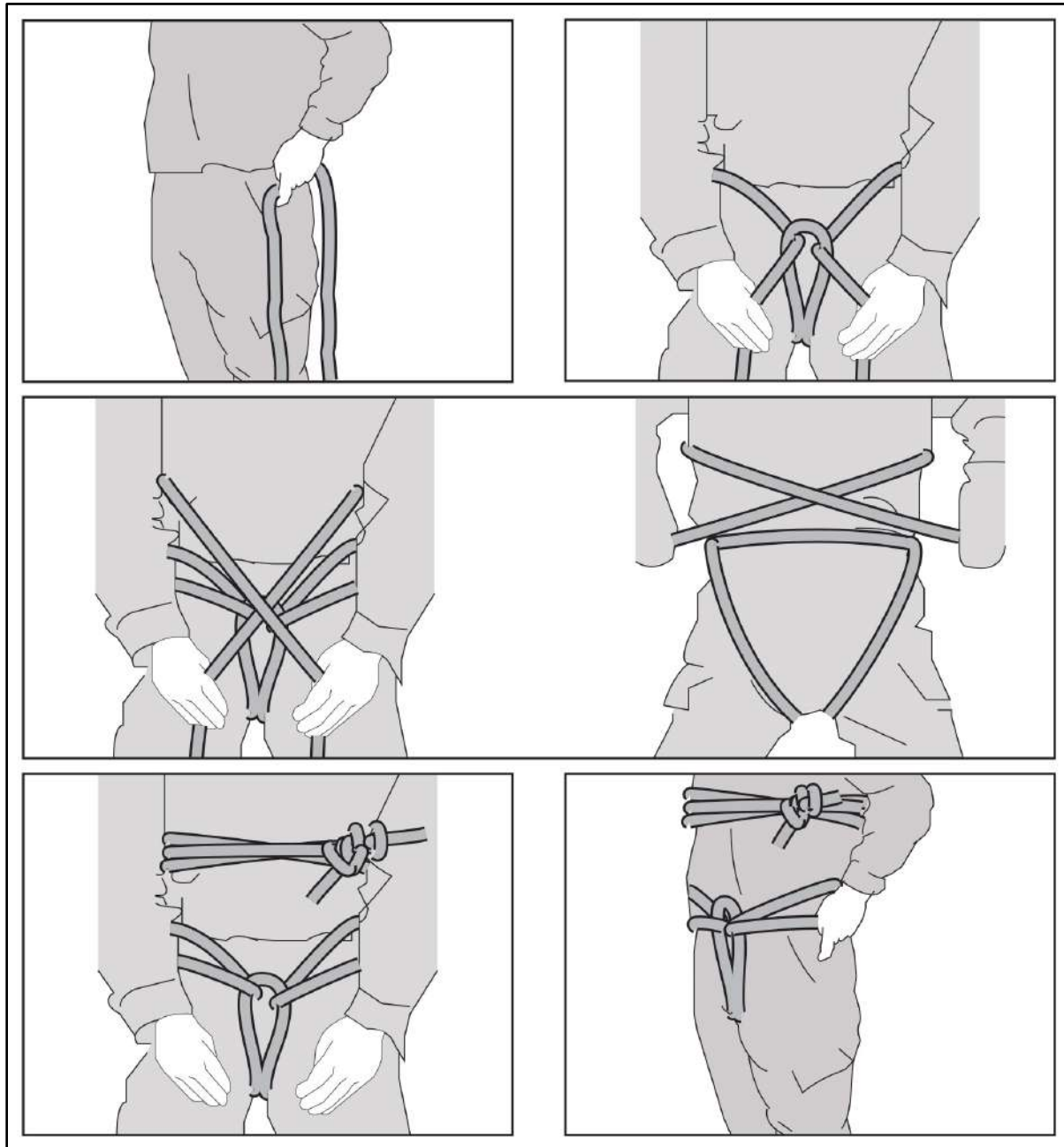
Figure 8-36. Field expedient harness
