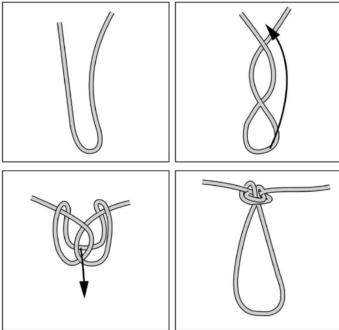
Figure 8-13. Alpine butterfly knot
