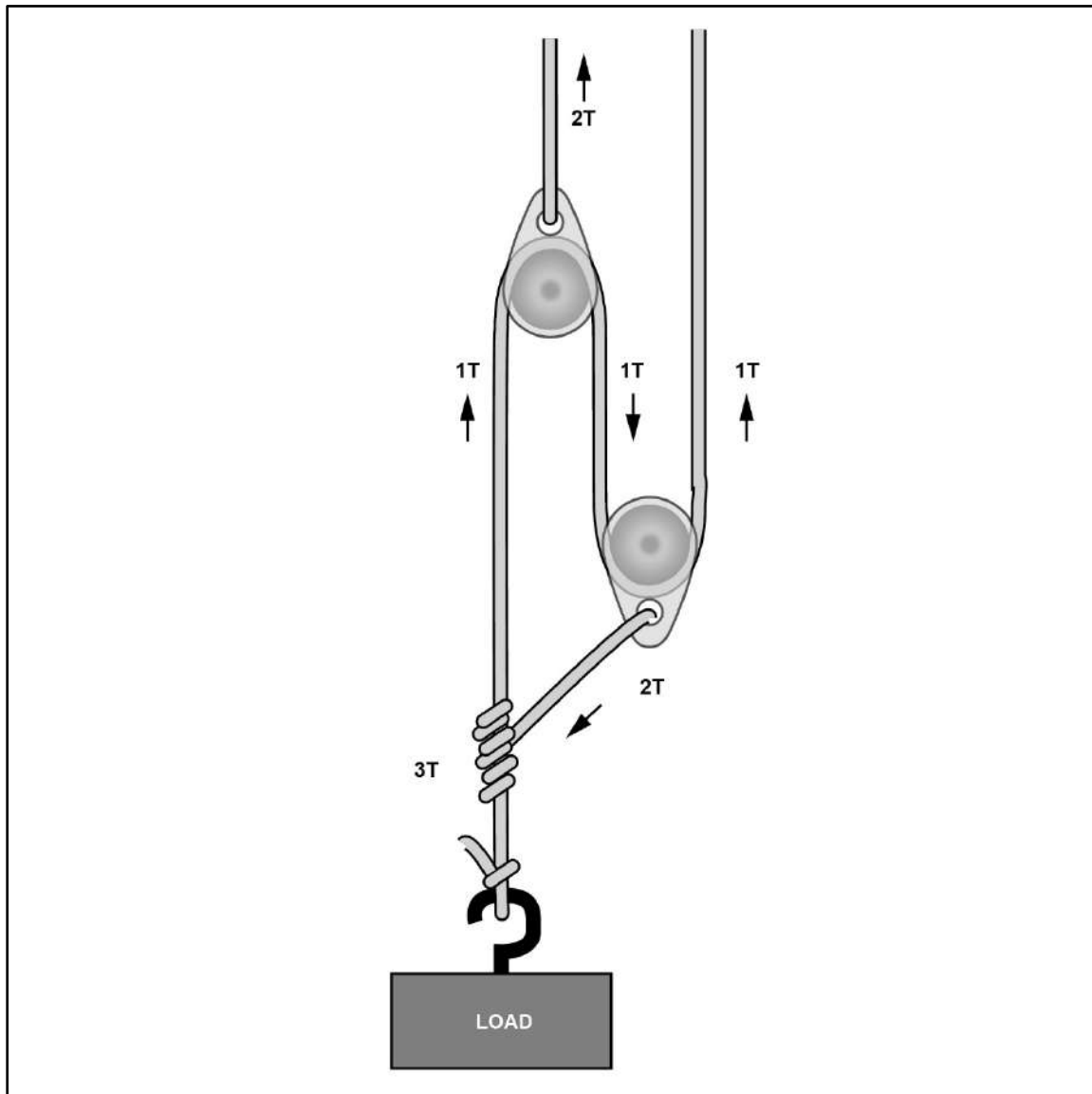
Figure 12-2. T-Method for simple 3:1 system
