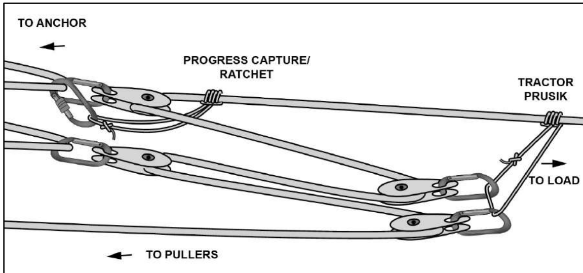
Figure 12-5. Simple 5:1 hauling system
