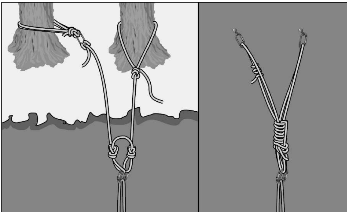
Figure 10-9. Top rope climbing set up
