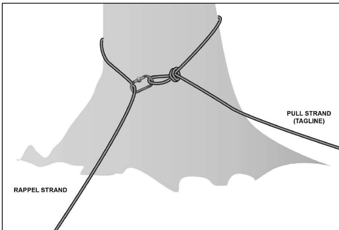
Figure 11-9. Tagline retrievable rappel using a tagline
