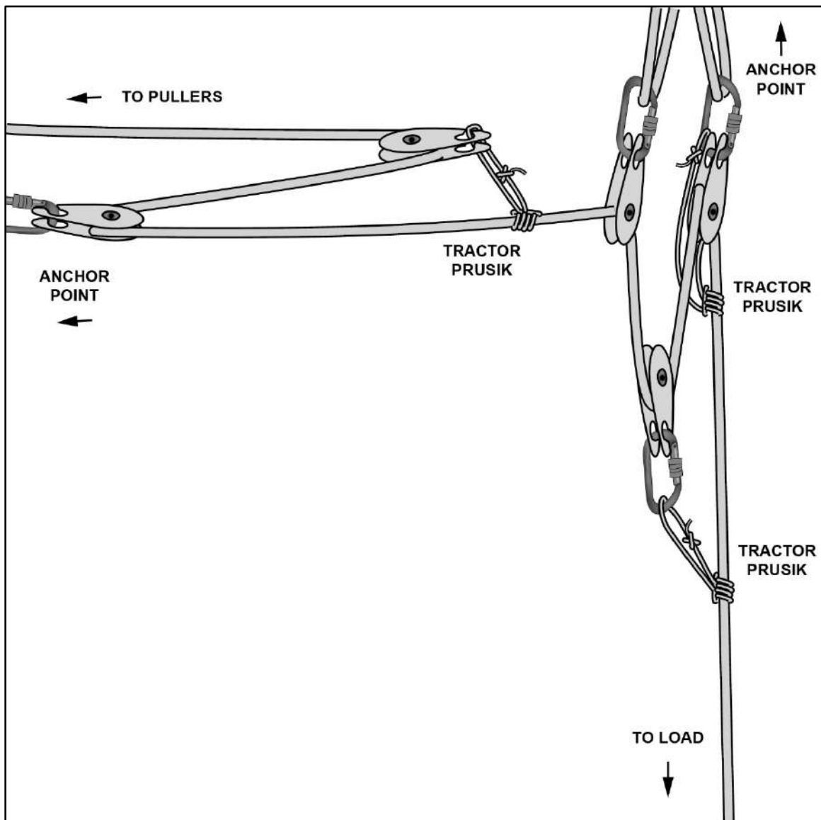
Figure 12-12. Redirected and offset compound hauling system
