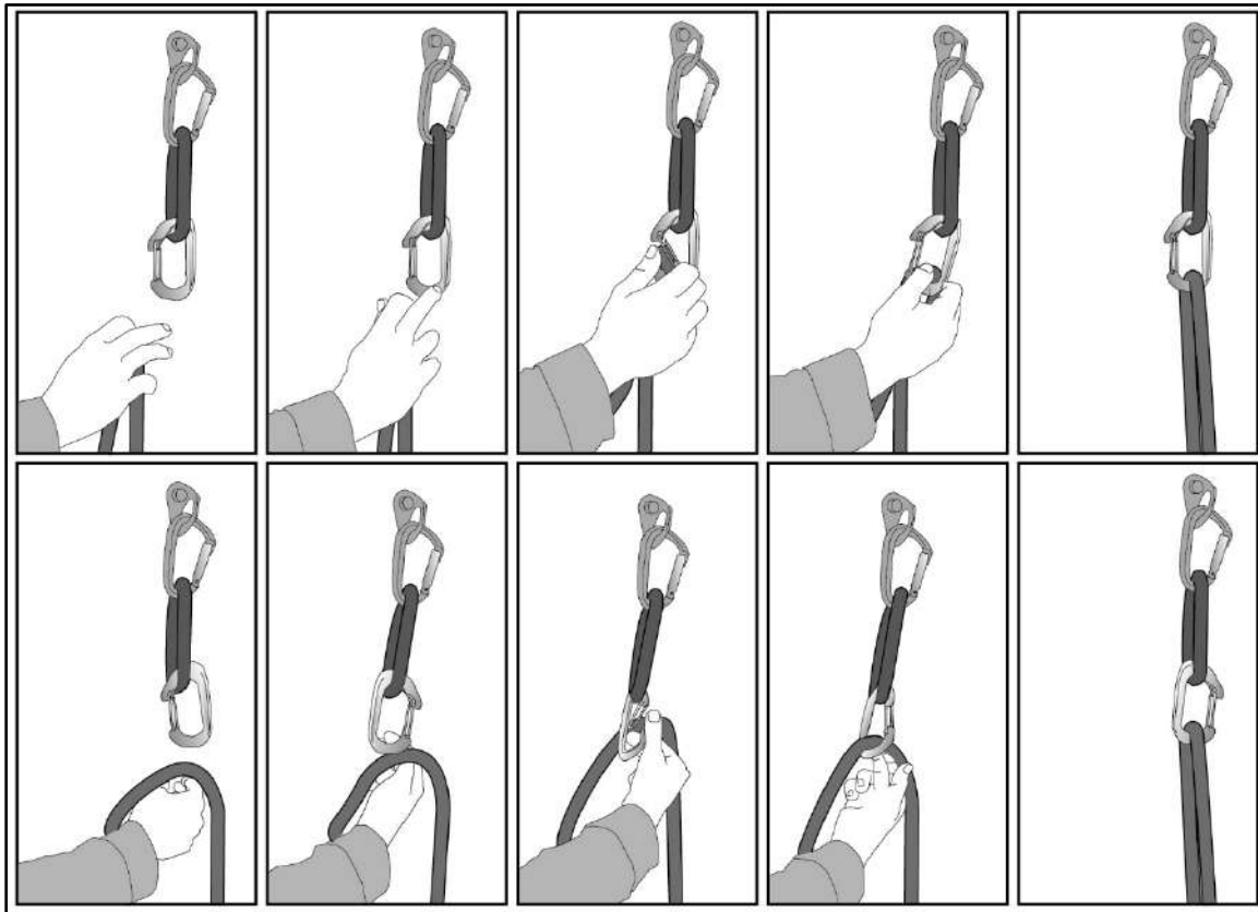
Figure 10-18. Proper clipping techniques
