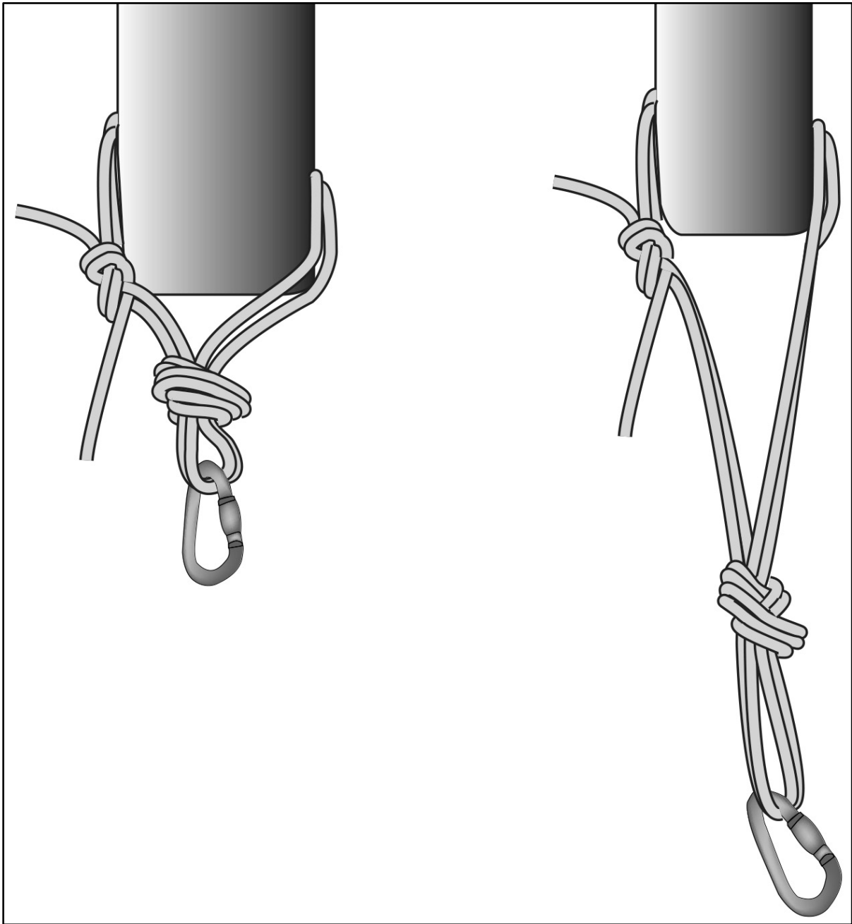
Figure 9-4. Single and double basket hitch with master point
