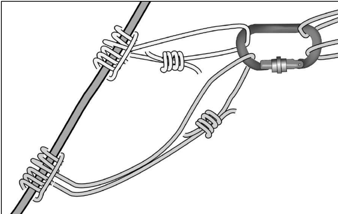
Figure 15-11. Tandem prusik belay
