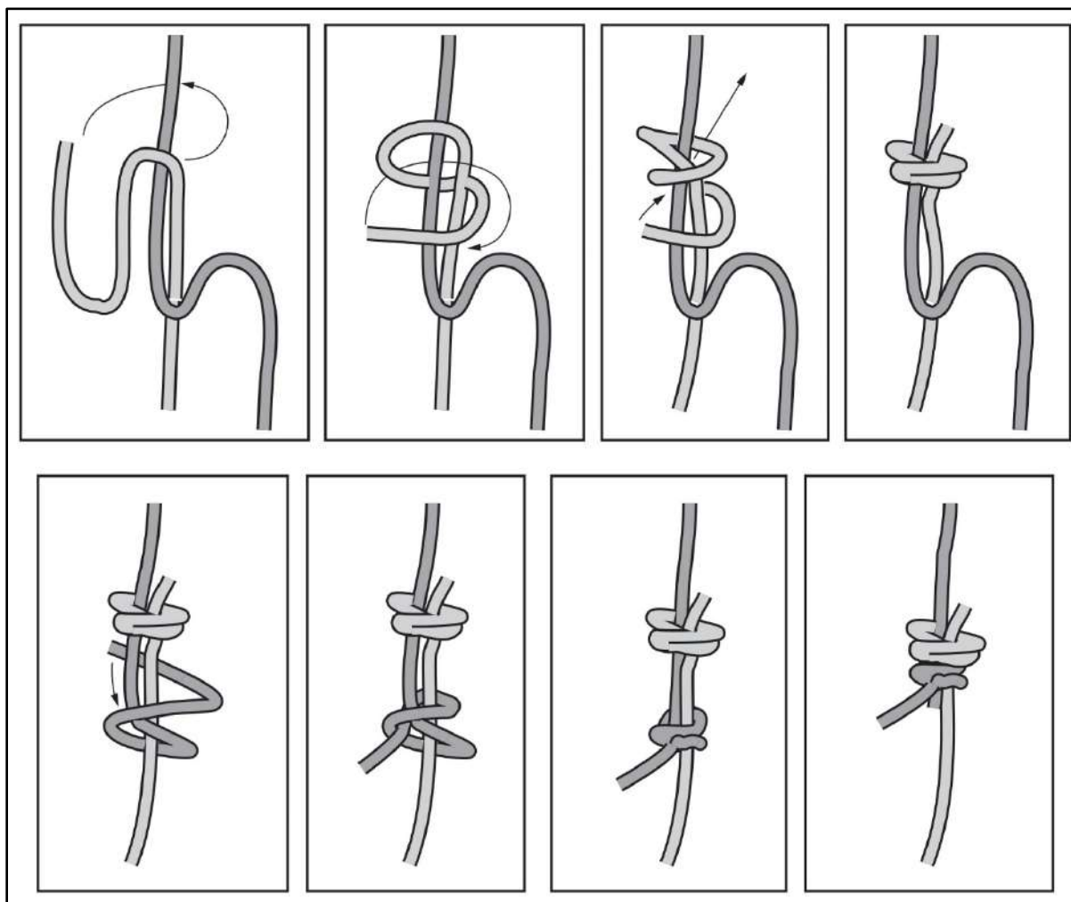
Figure 8-17. Double fisherman's knot
