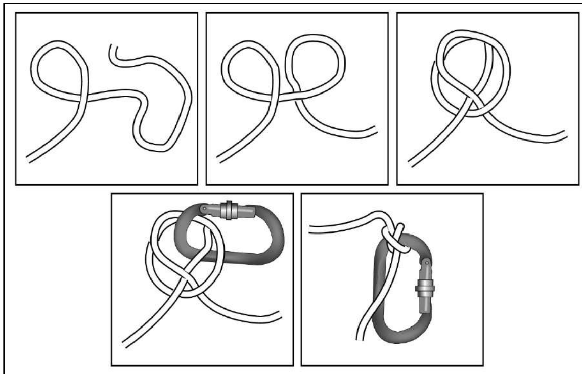
Figure 8-28. Middle-of-the-rope clove hitch
