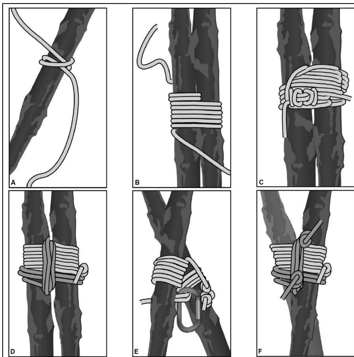
Figure 16-7. A-frame horizontal and vertical wraps
