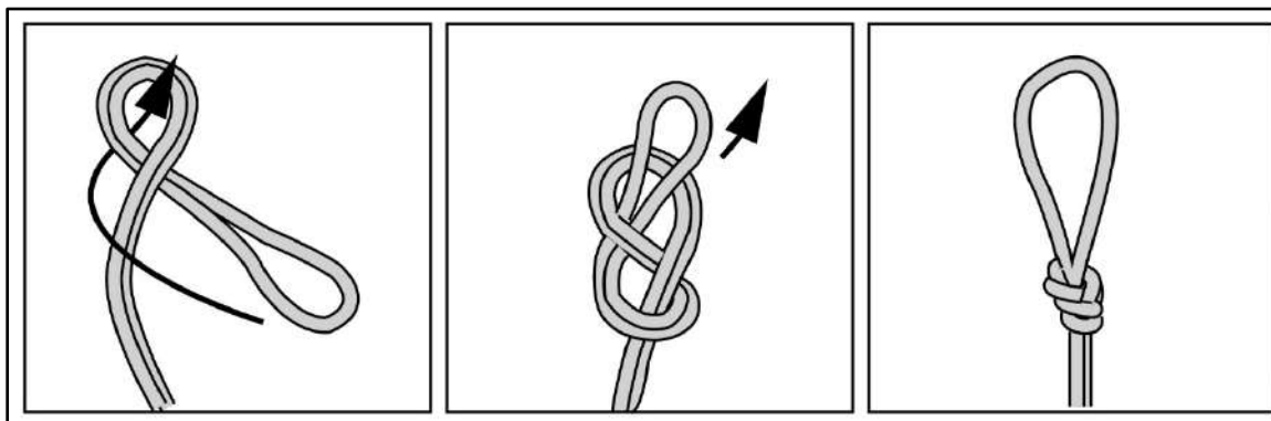
Figure 8-9. Figure eight on a bight
