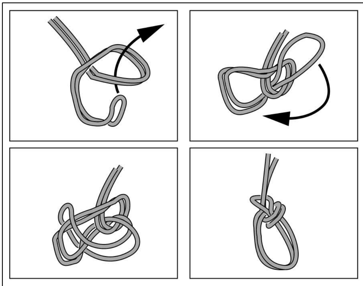
Figure 8-21. Bowline on a bight
