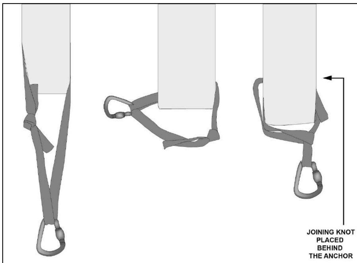
Figure 9-2. Single-point webbing anchors: single loop, double bight, and girth hitch
