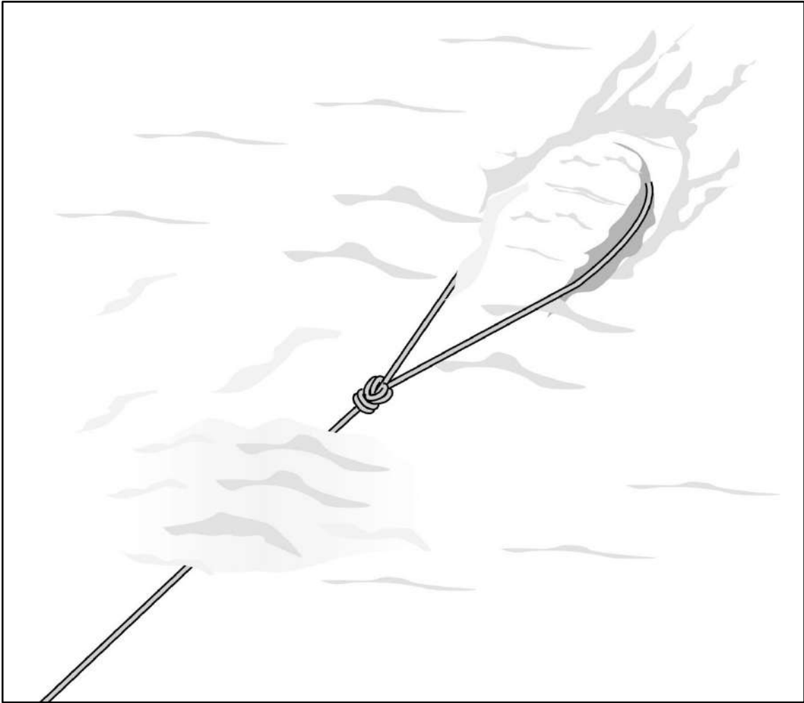
Figure 9-32. Snow bollard anchor
