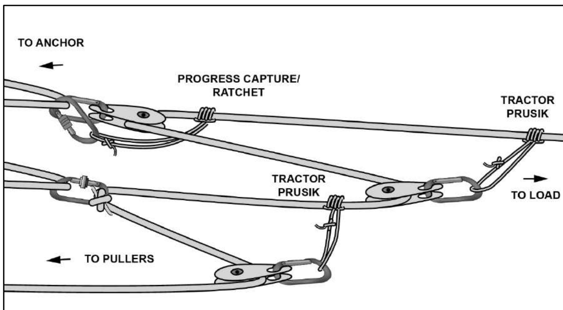
Figure 12-6. Compound 6:1 hauling system
