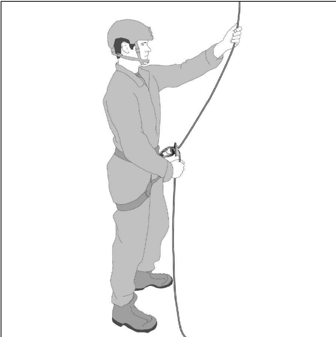
Figure 10-10. Top rope belay with tube-style device
