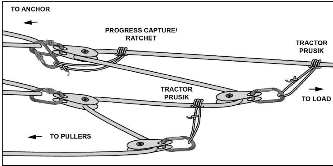
Figure 12-7. Compound 9:1 hauling system
