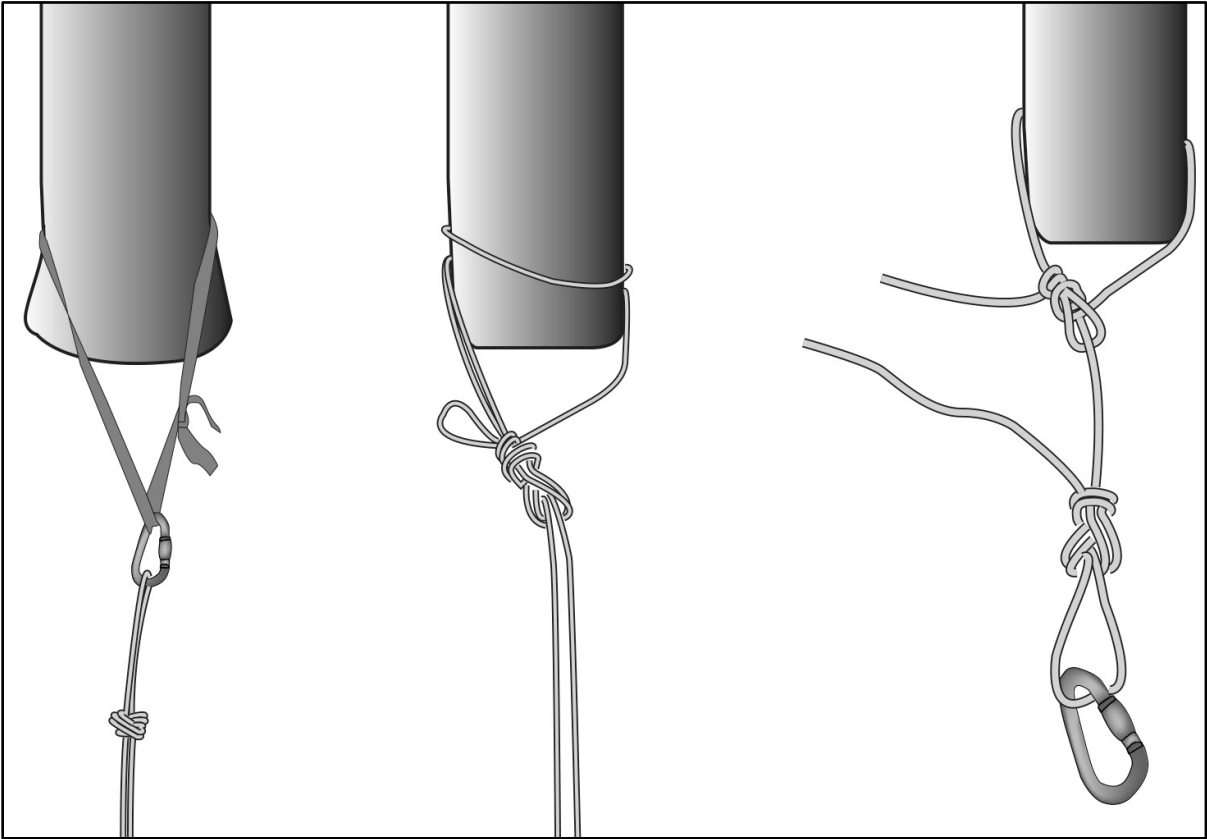
Figure 9-8. Anchoring a rope to a single-point tree anchor
