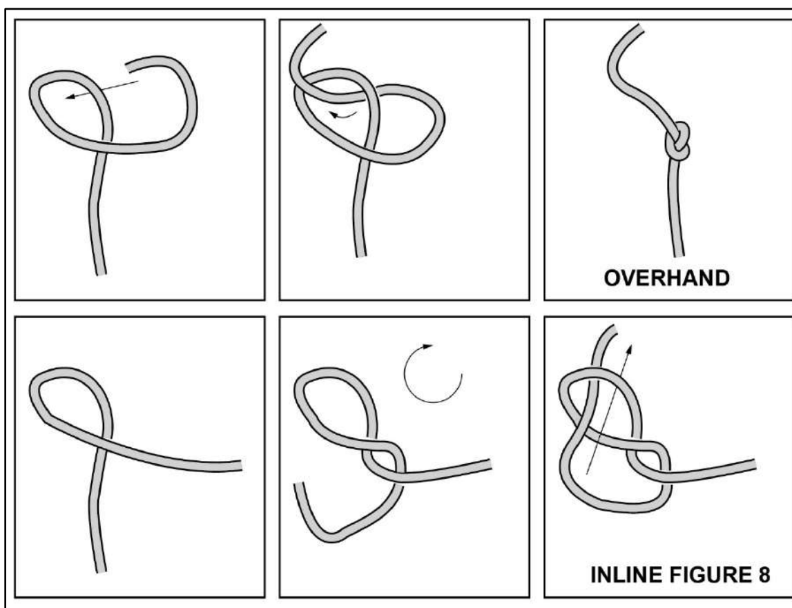
Figure 8-7. Overhand and inline figure eight
