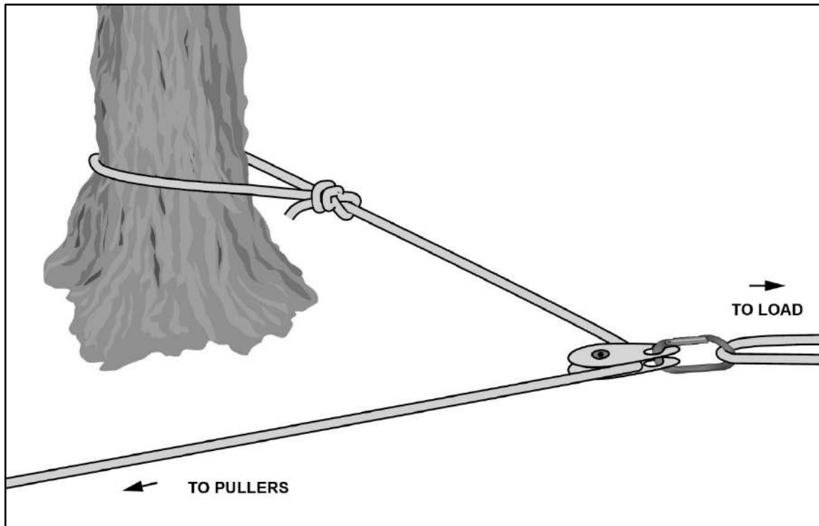
Figure 12-3. Simple 2:1 hauling system
