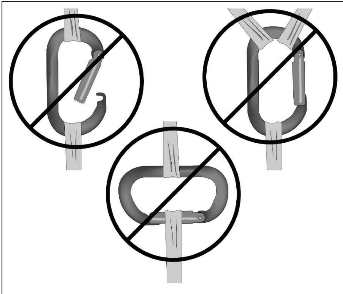
Figure 8-5. Improper carabiner loading
