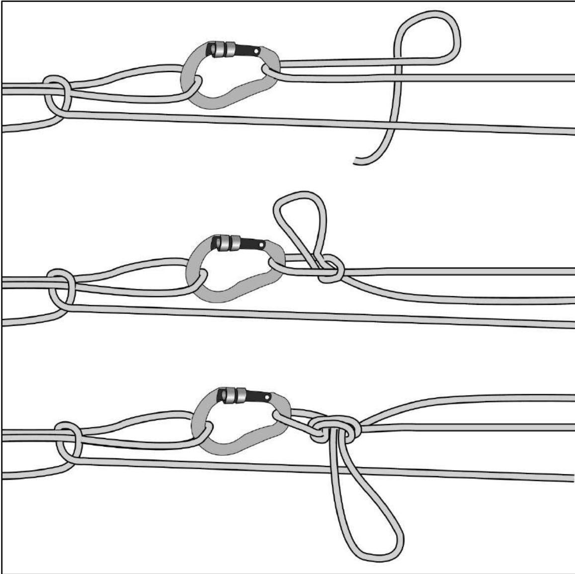
Figure 16-2. Mule knot secured with an overhand knot
