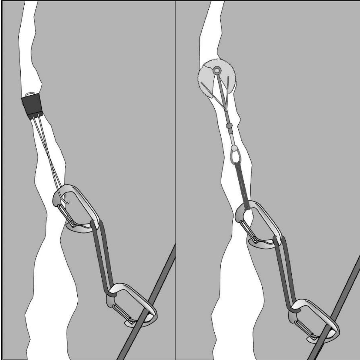
Figure 10-17. Proper extension of cams and chocks using runners
