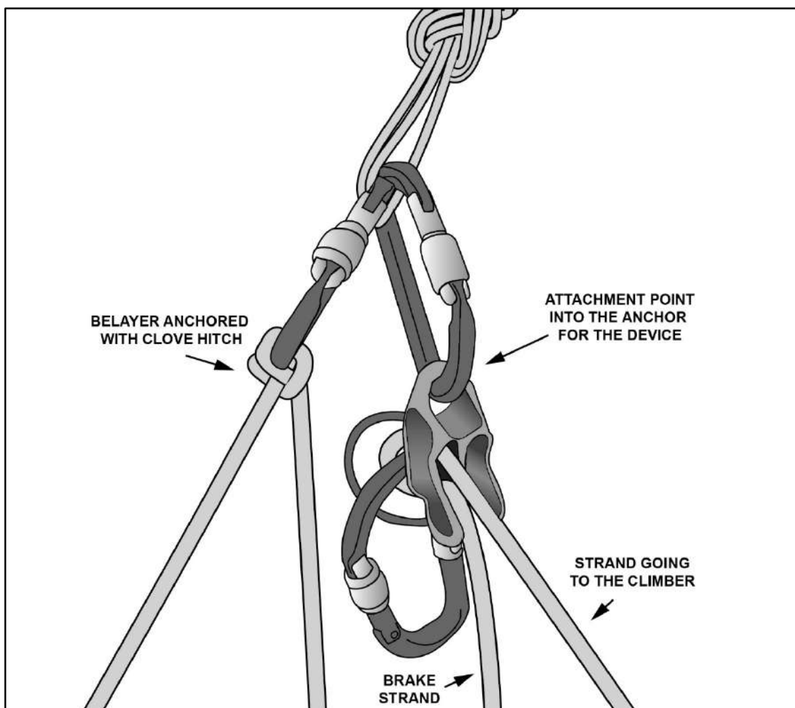
Figure 10-20. Belaying a climber using an autolocking device in guide mode
