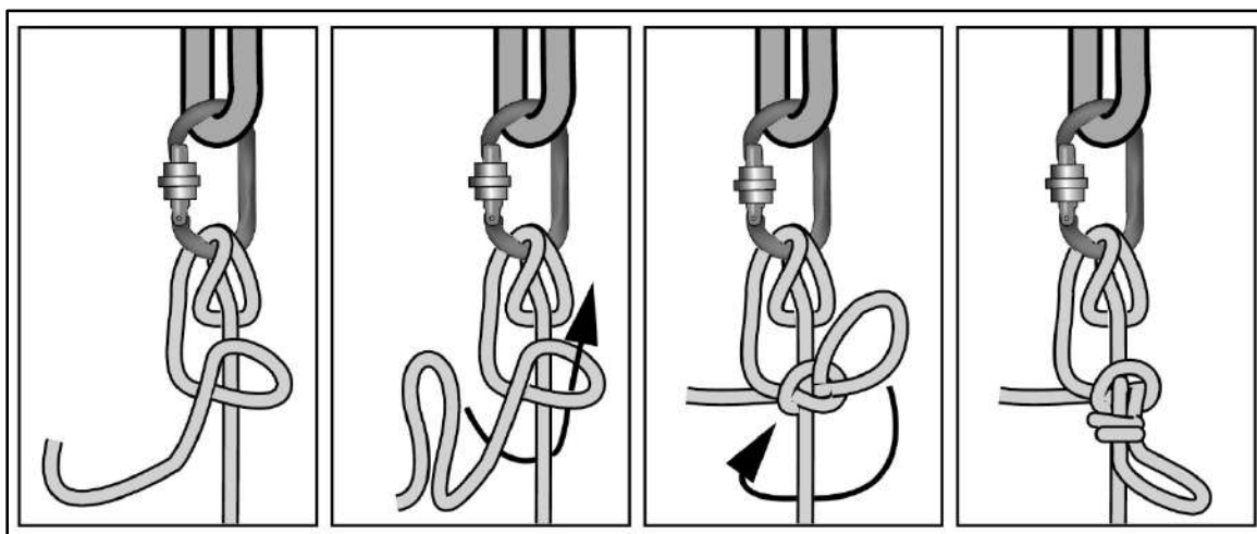
Figure 8-33. Munter mule knot using installation rope
