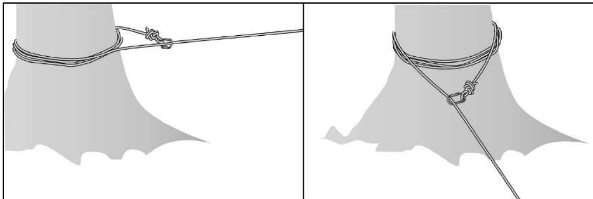
Figure 16-4. High strength tie off (tensionless hitch)
