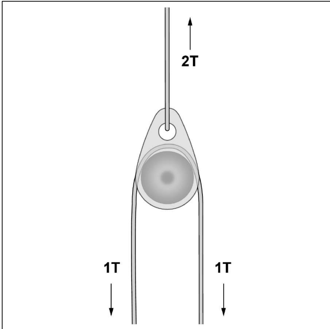
Figure 12-1. T-Method for simple 2:1 system
