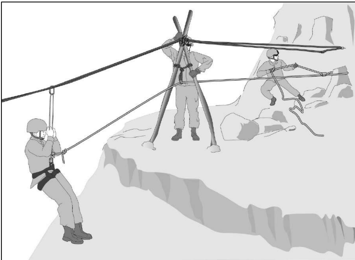
Figure 16-6. Artificial height (A-frame) used with high line
