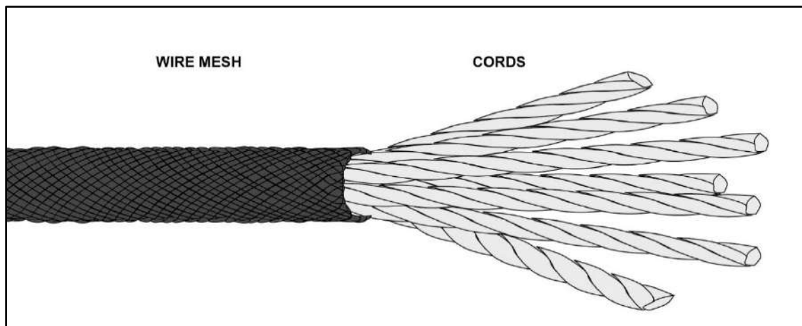
Figure 8-1. Kernmantle rope construction
