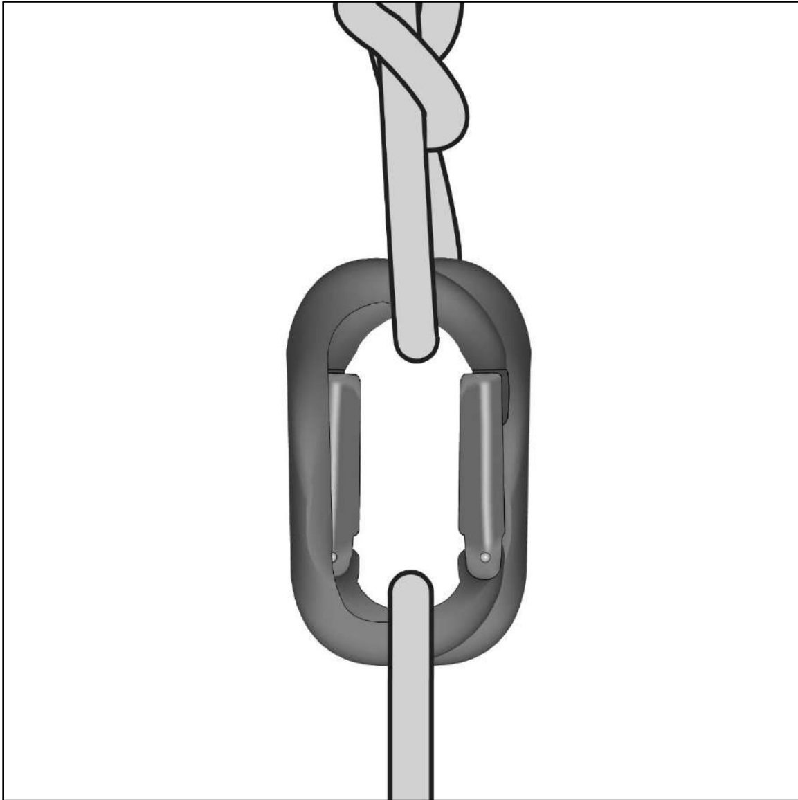
Figure 9-1. Opposite and opposed carabiners
