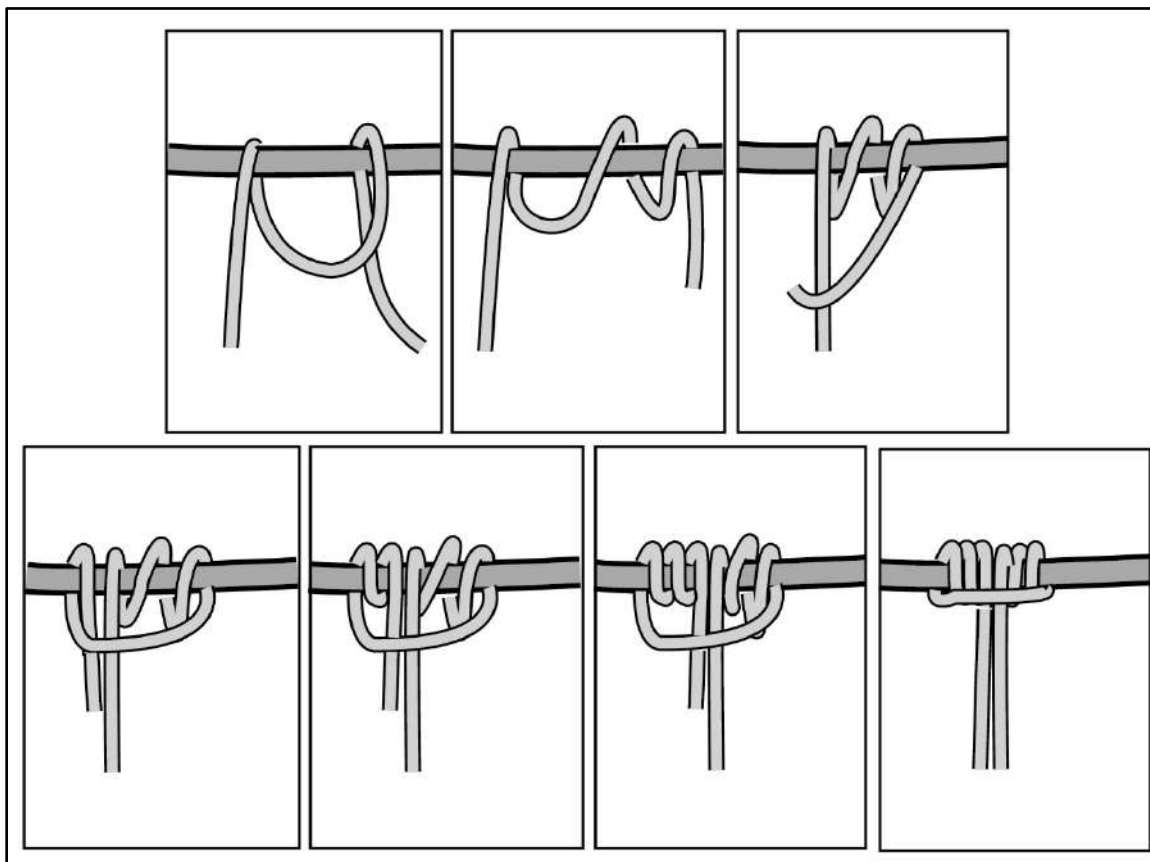
Figure 8-24. End-of-the-rope prusik knot
