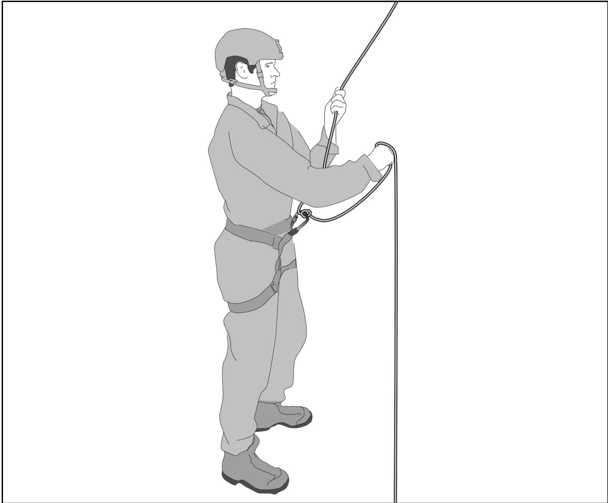
Figure 10-12. Munter belay technique
