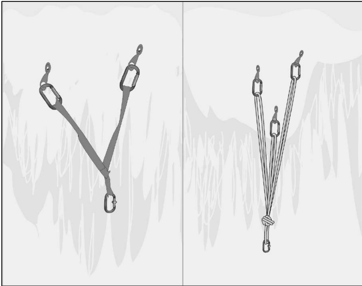
Figure 9-24. Multipoint ice anchor construction
