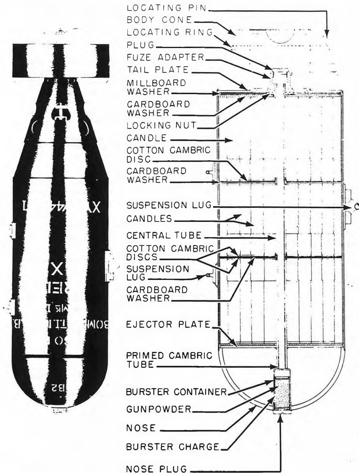
Figure 81—T.I. 1,000-lb. Bomb No. B. 2 Mk I
