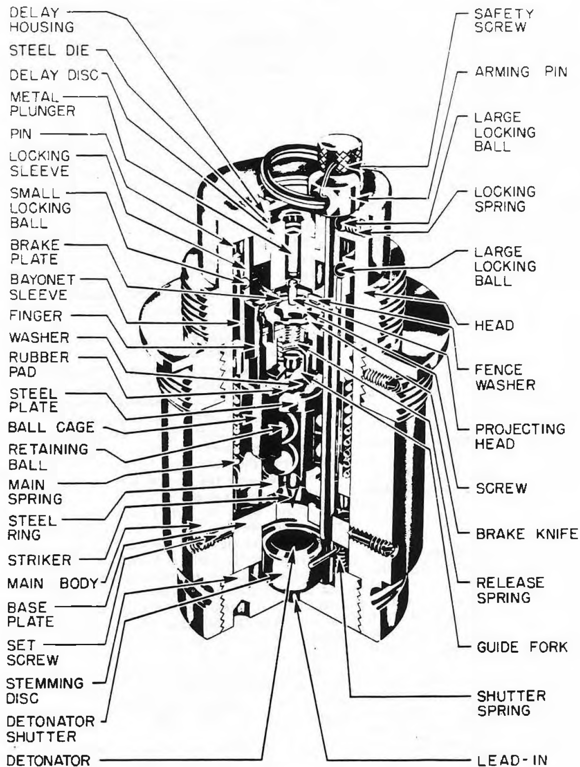
Figure 174—Tail Fuze No. 881 Mk 1
