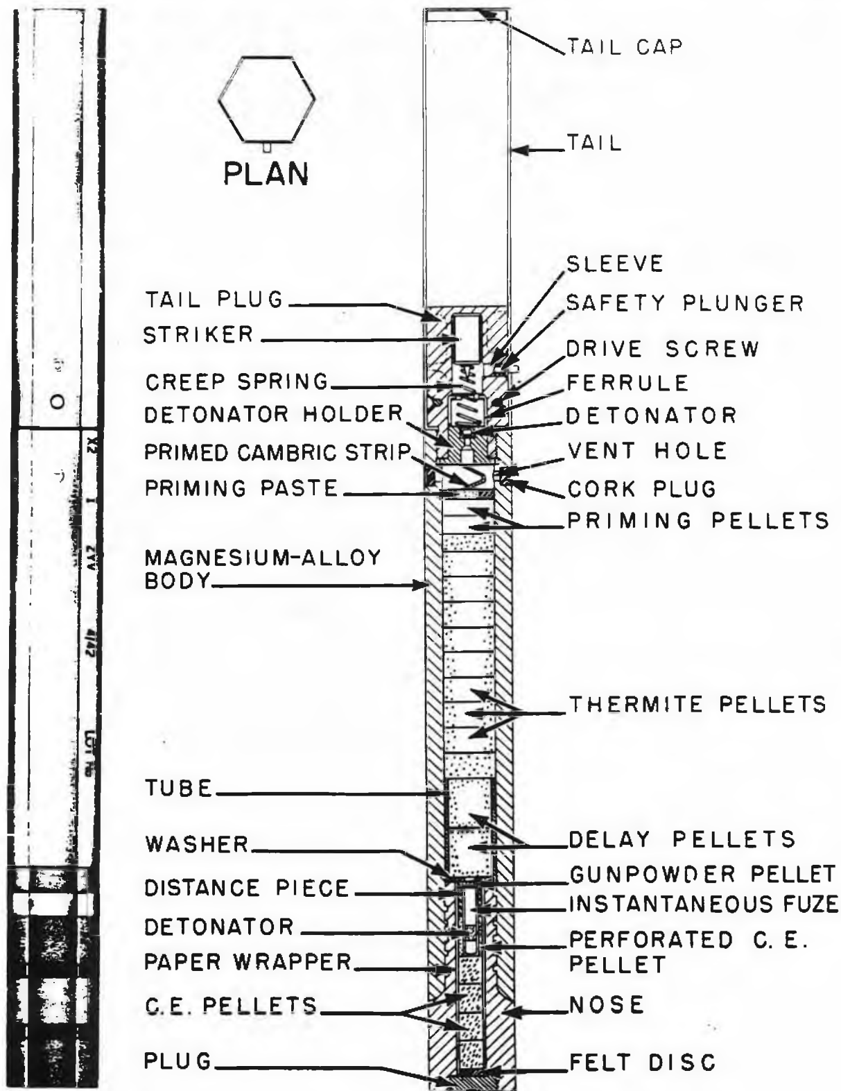
Figure 38—l.b. 4-lb. "X" with 2-minute delay, Mk I
