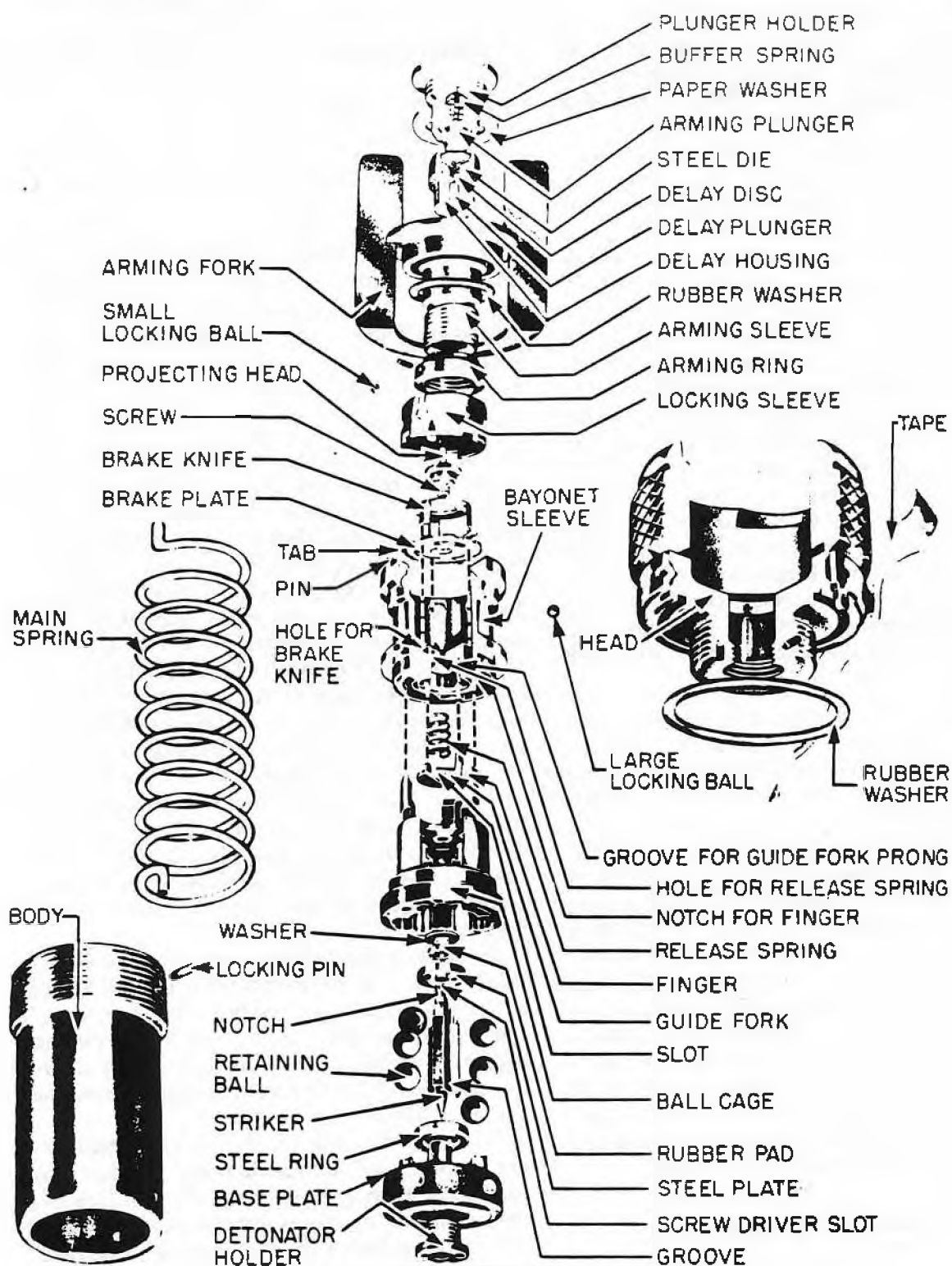
Figure 170—Exploded view of Tail Fuze No. 871 Mk 1
