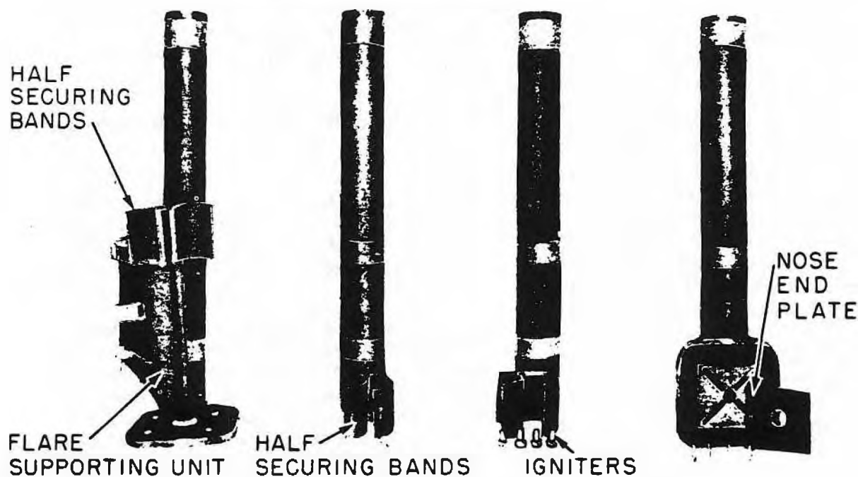
Figure 105—Cluster Projectile 400-lb. No. 3 Mk I
