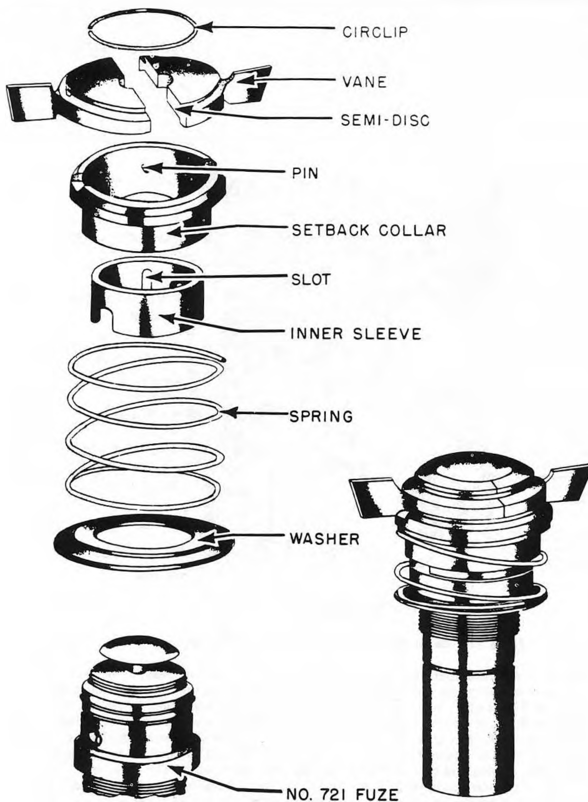
Figure 230—Nose Fuze No. 899 Mk I
