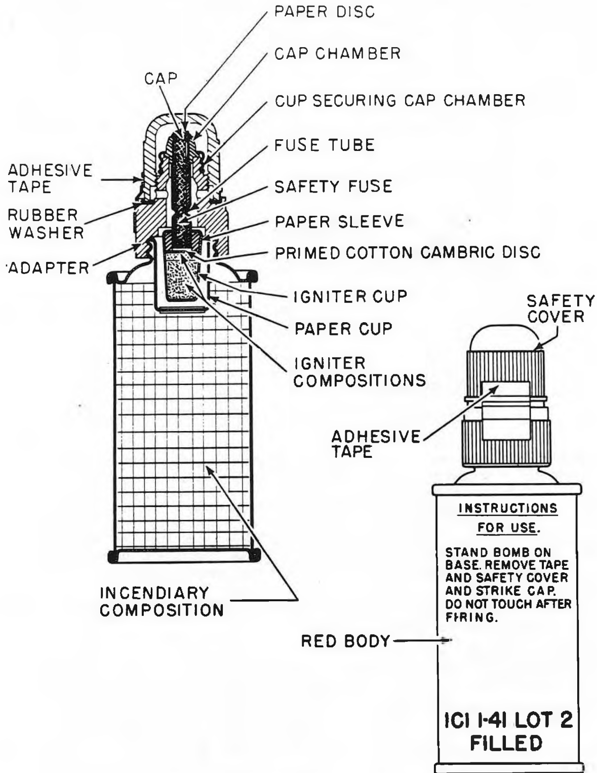
Figure 252—1 1/4-lb. Incendiary Bomb Mk I
