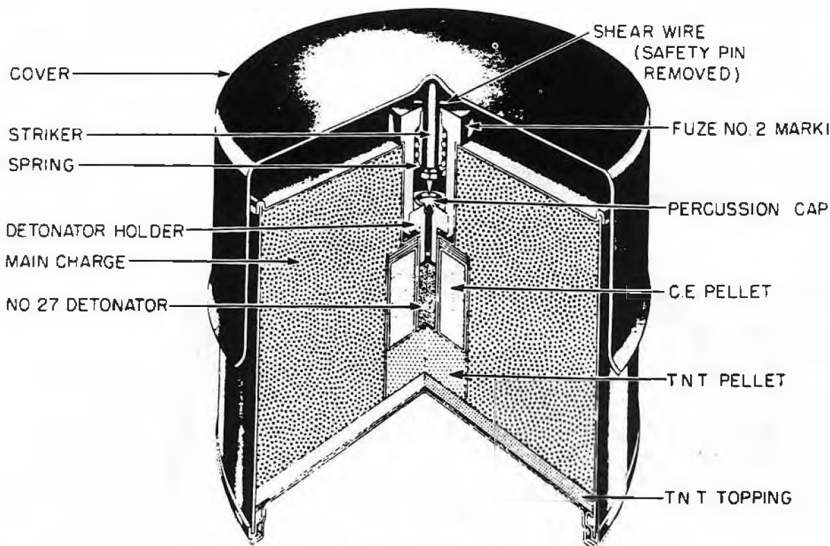
Figure 254—A./T. Mine G.S. Mk III
