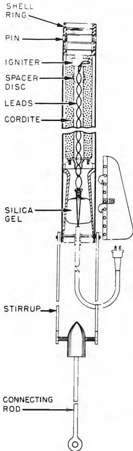
MOTOR NO. 3 MK II
