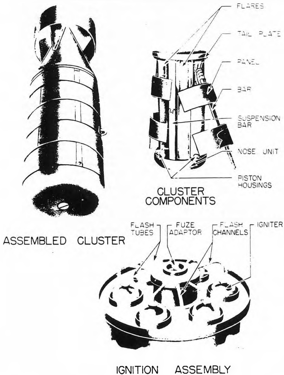
Figure 103—Cluster Projectile 270-lb. No. 1 Mk 1
