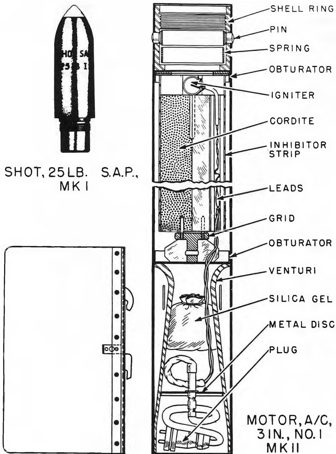
Figure 192—3-in. Aircraft Rocket Components
