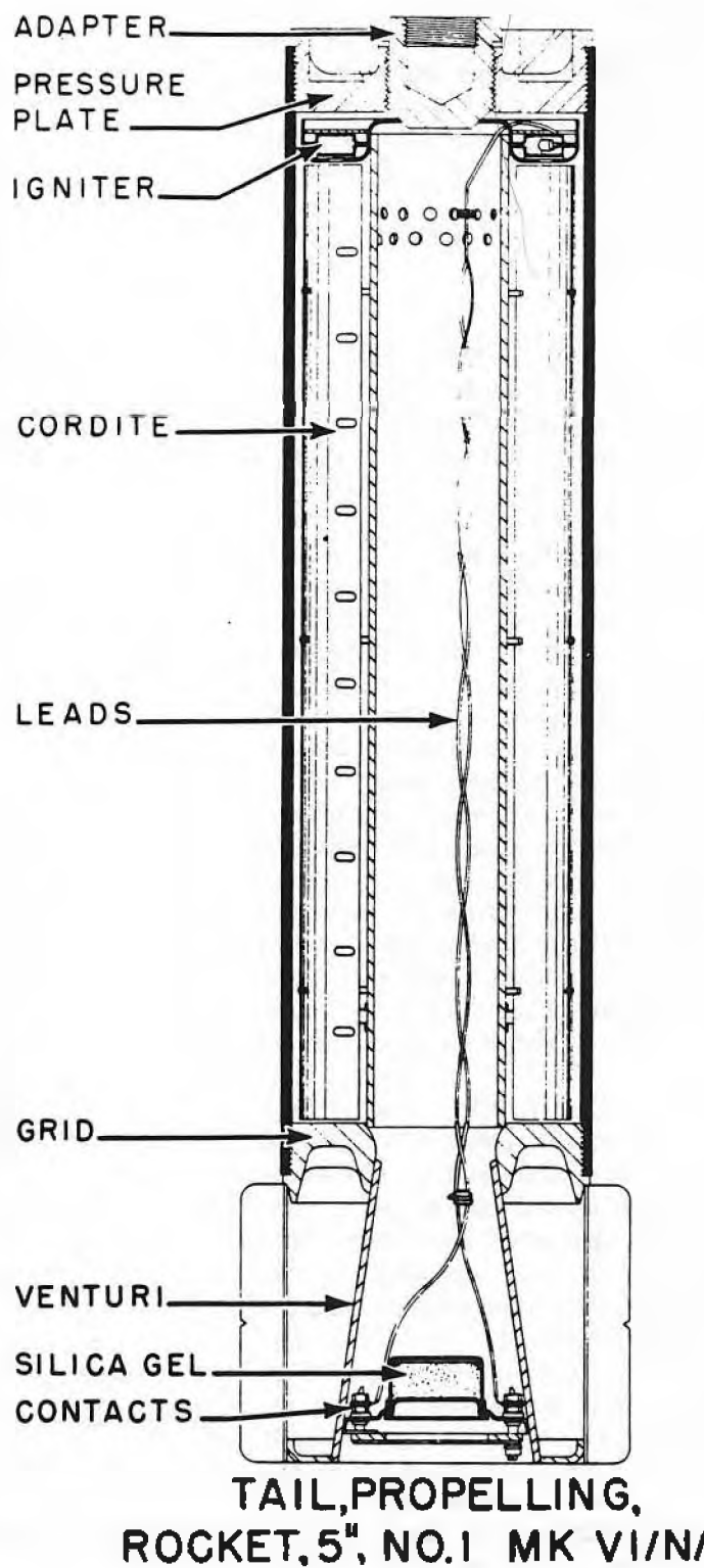
Figure 195—5-in. Barrage Rocket Components
