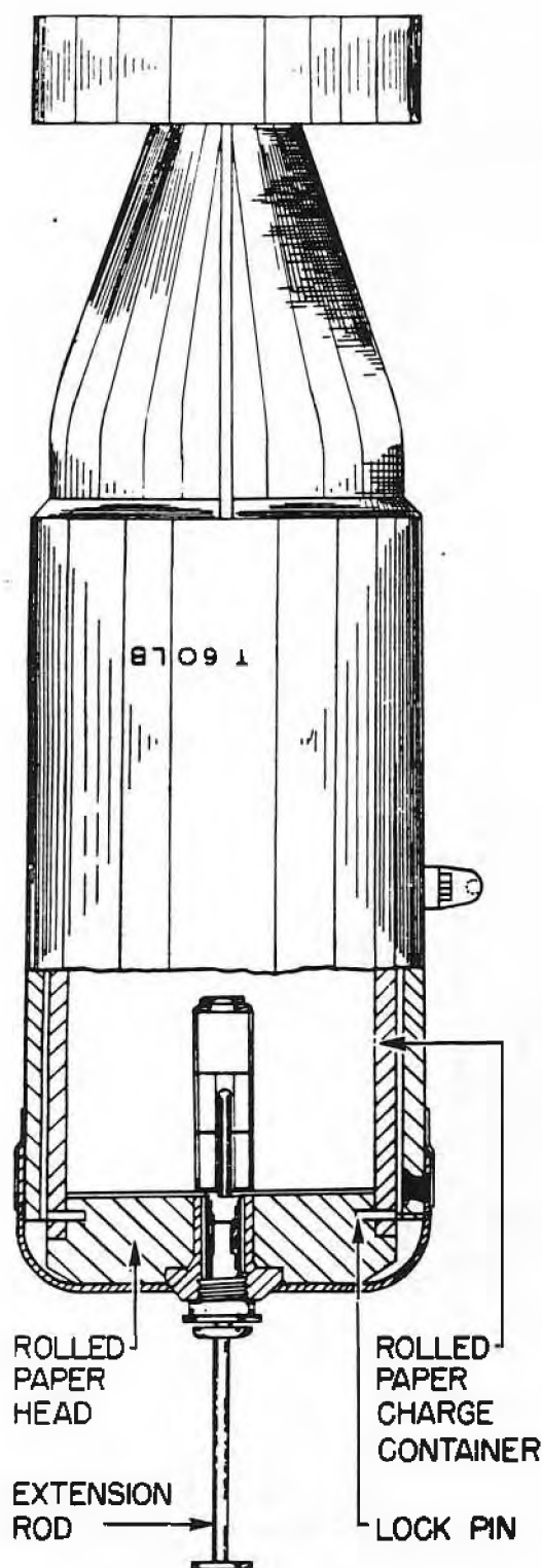
Figure 60—I.T. 60-lb. Bomb
