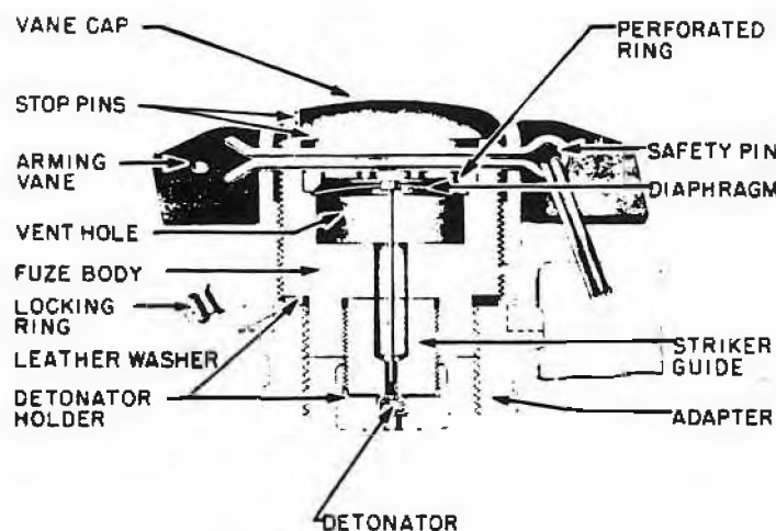
Figure 172—Nose Fuze No. 874 Mk I
