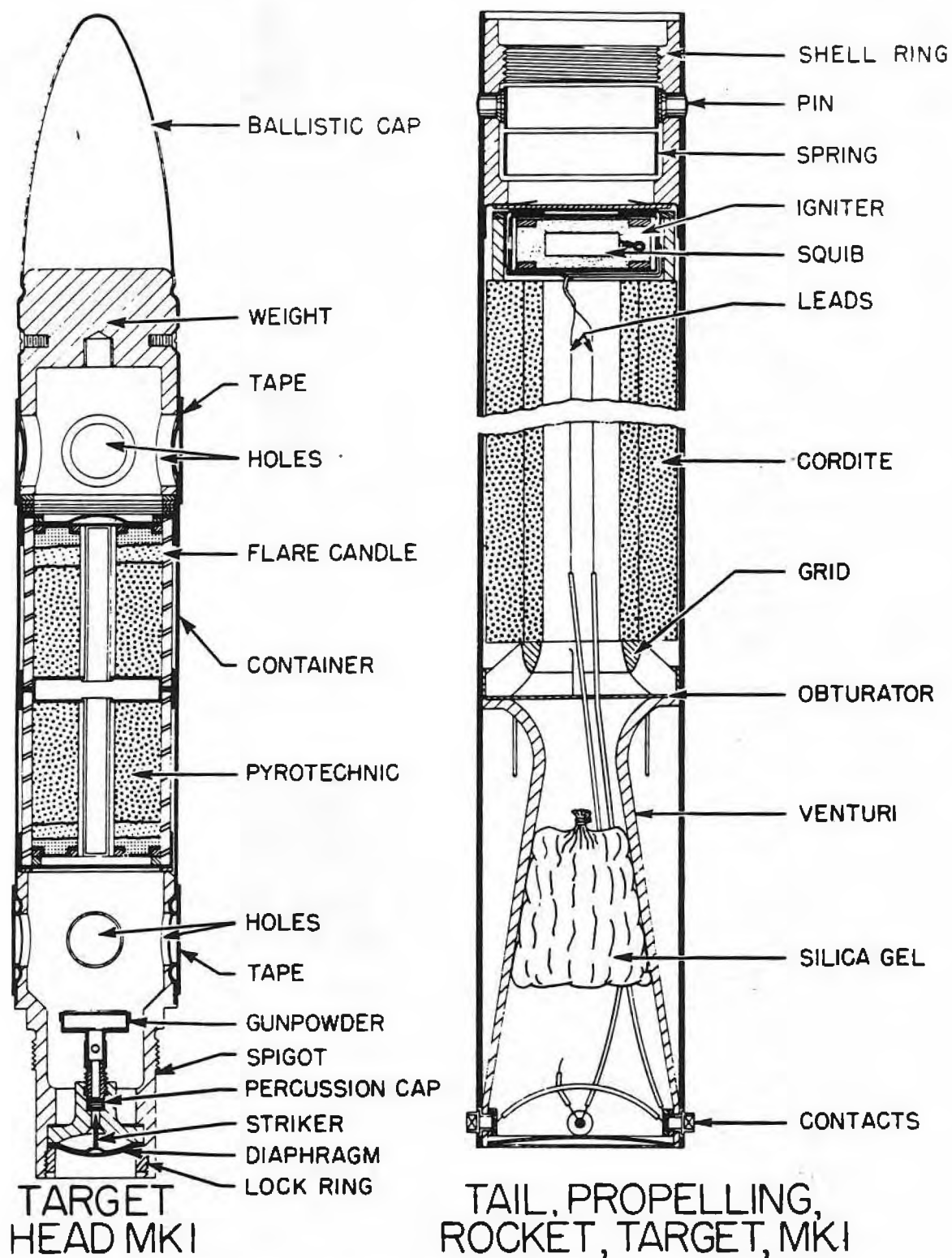
Figure 202—2-in. U.P. Target Rocket Components
