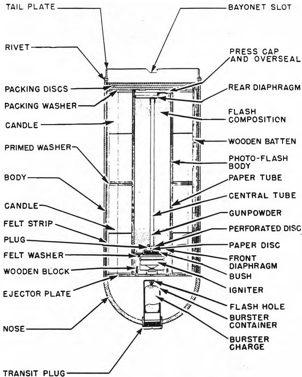
Figure 78—T.I. 250-lb., Photoflash, Bomb No. 13 Mk 1
