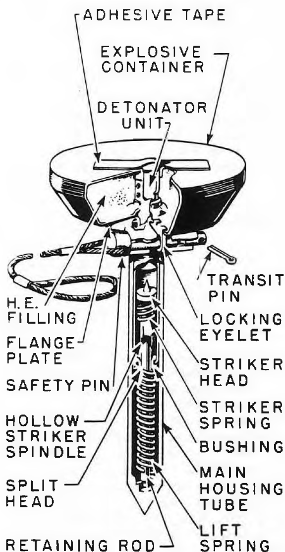
Figure 278—Release Switch No. 12 Mk I
