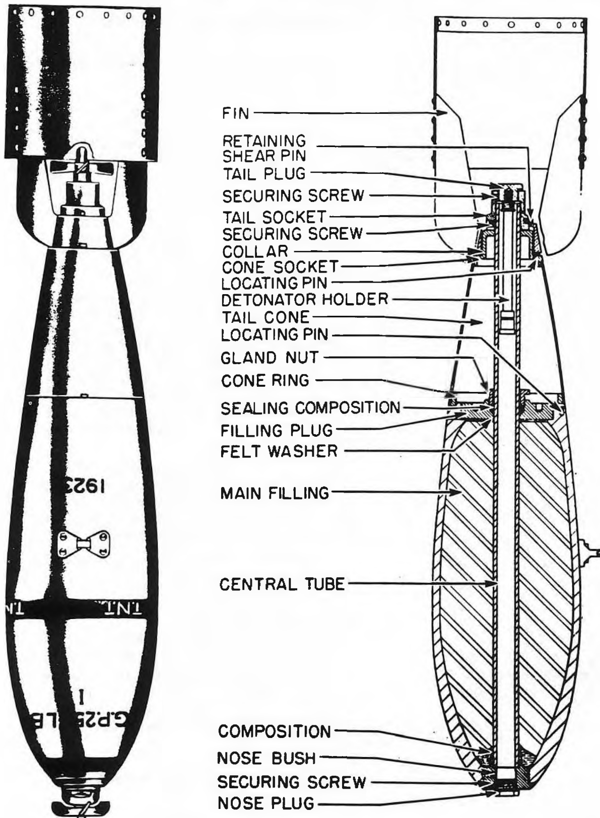
Figure 9—G.P. 250-lb. Bomb Mk I
