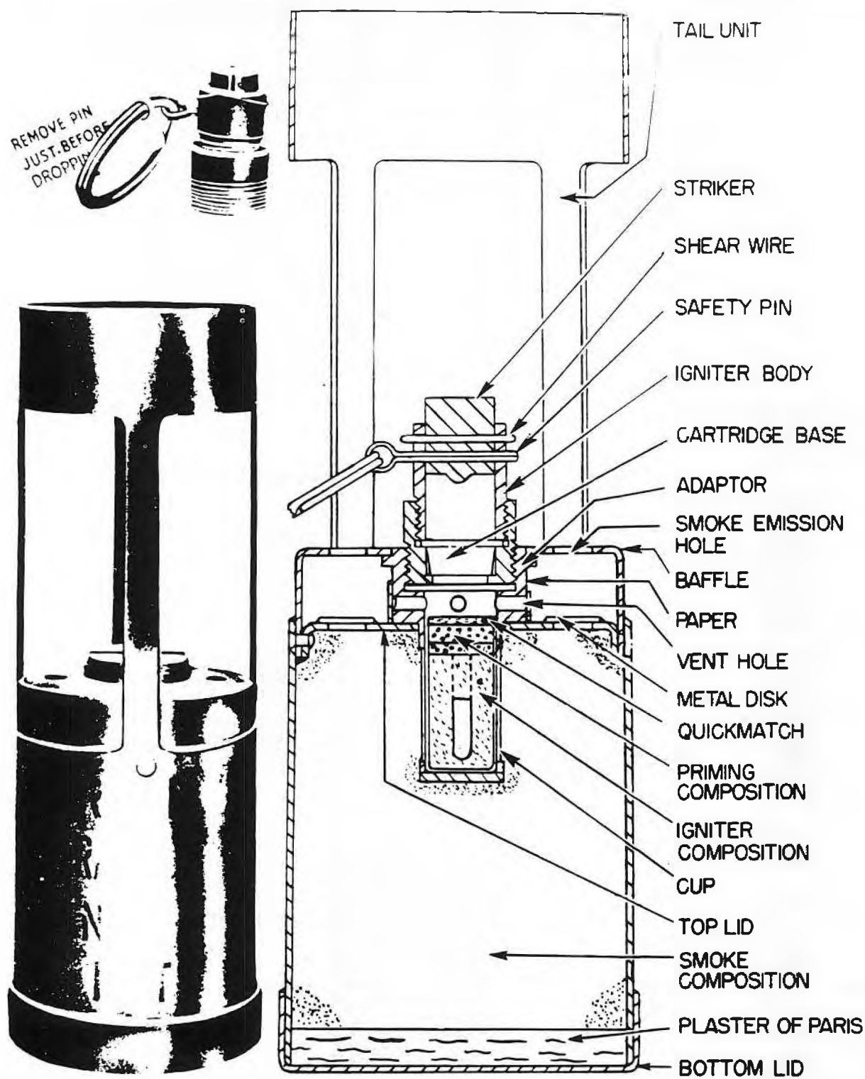
Figure 102—Smoke Generator No. 6
