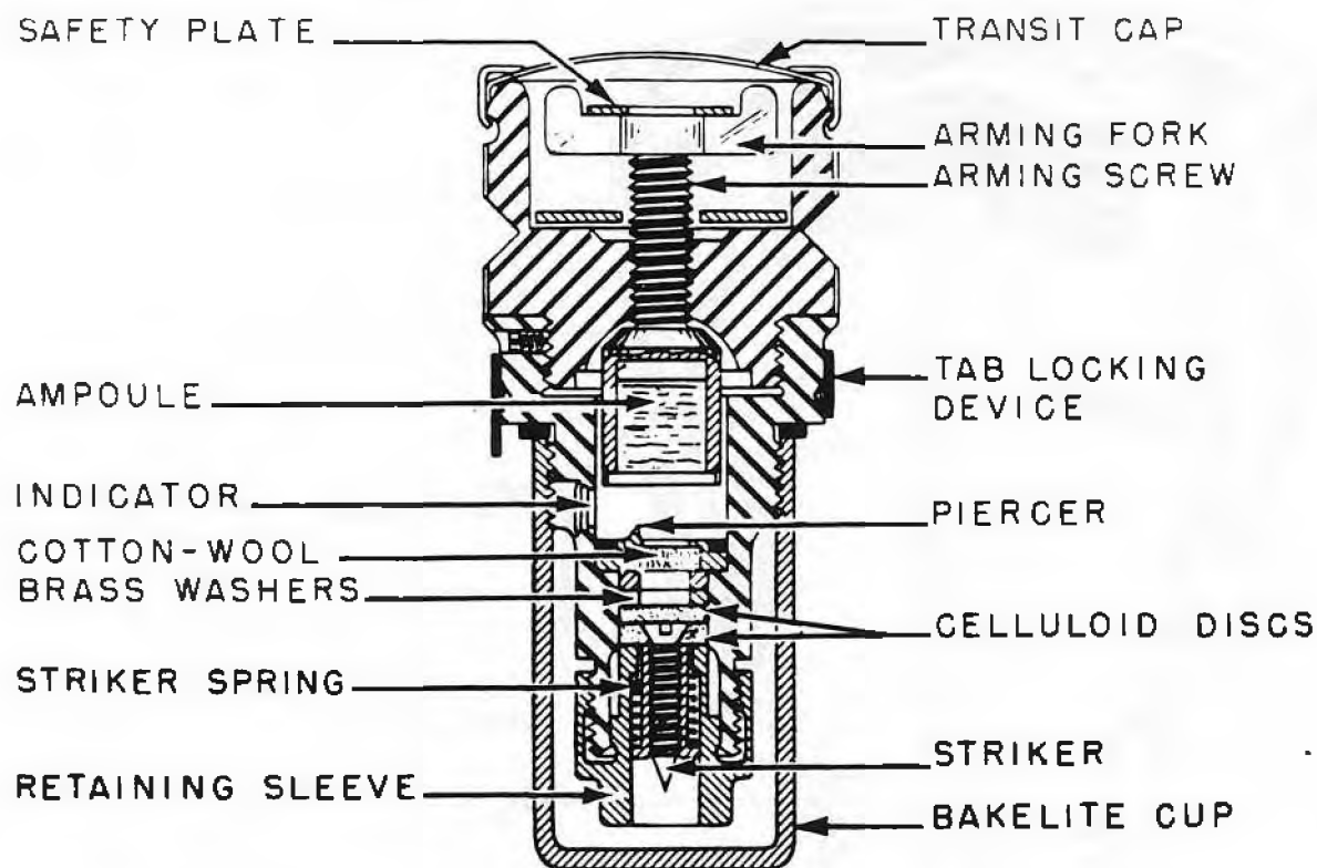
Figure 142—Tail Pistol No. 62 Mk I
