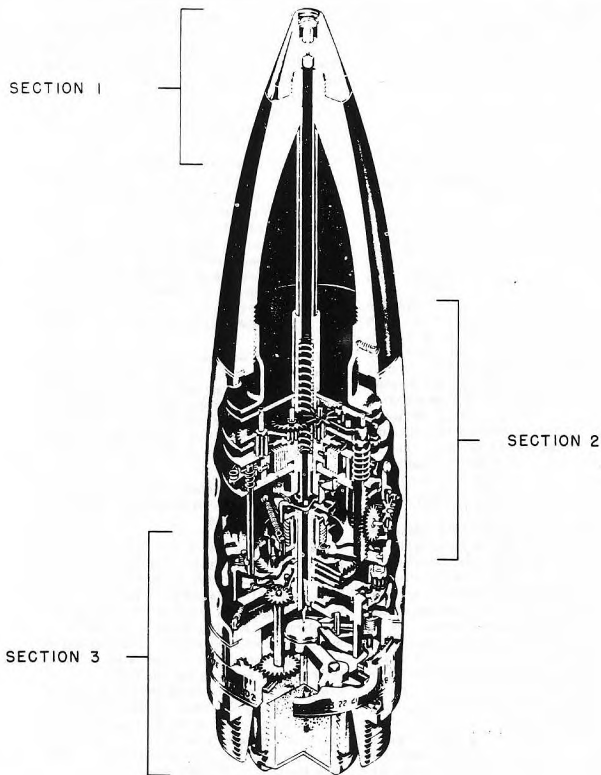
Figure 227—Nose Fuze No. 731 Mk 1
