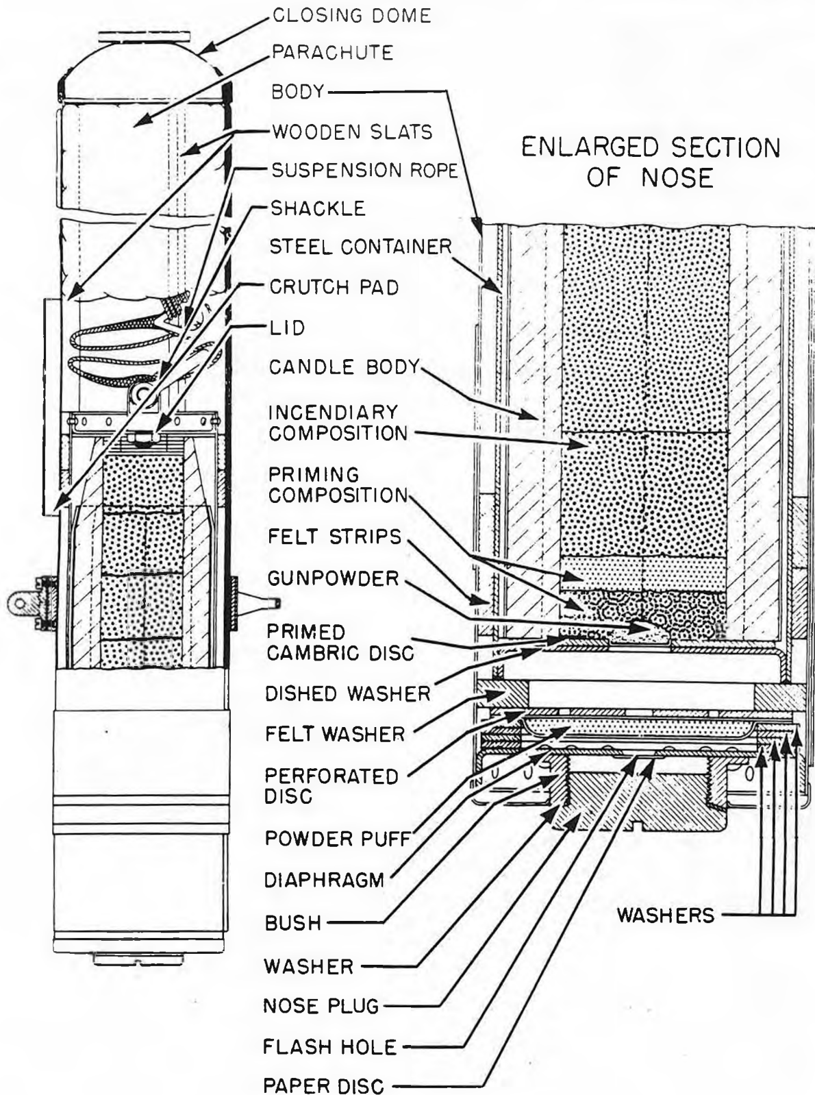
Figure 86—4.5-in. Skymarker Flare No. 1 Mk 1
