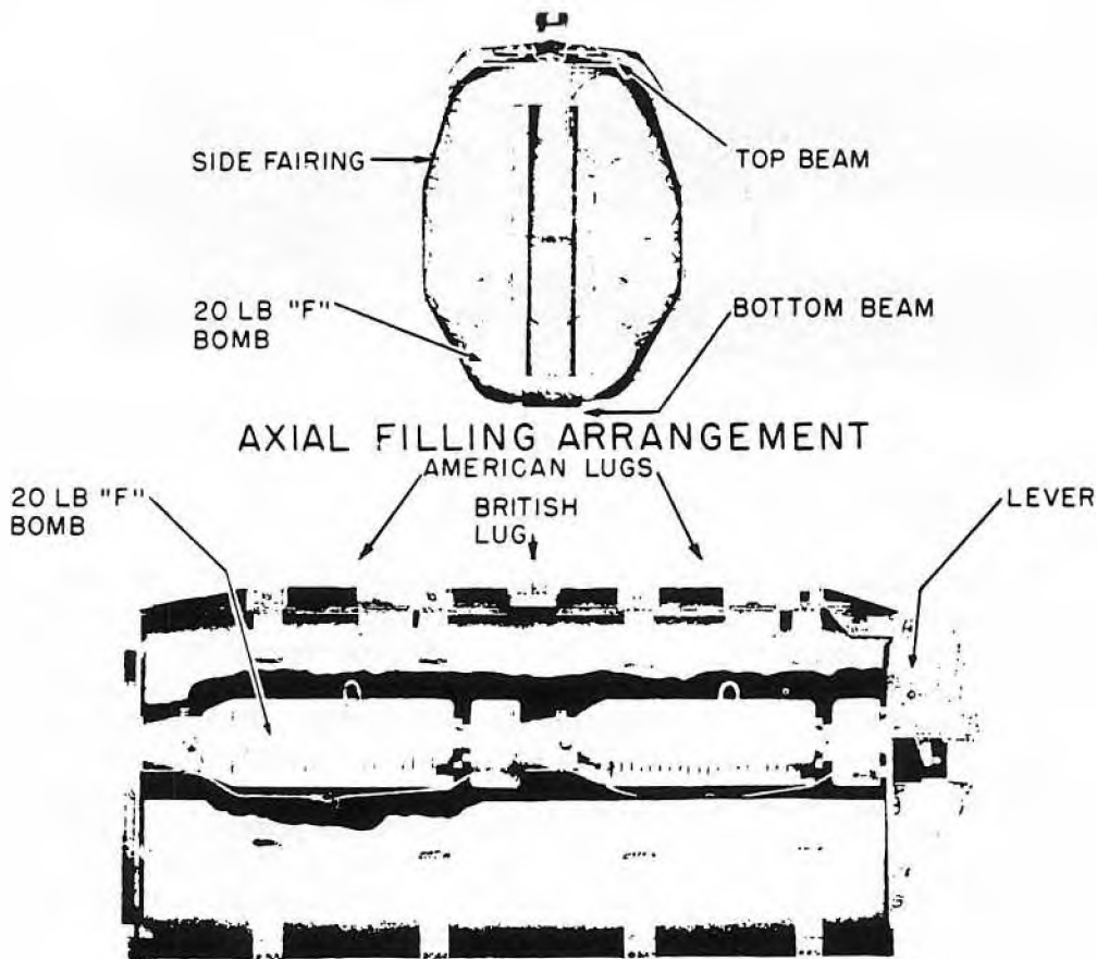
Figure 116—Cluster Projectile 500-lb. No. 24 Mk I
