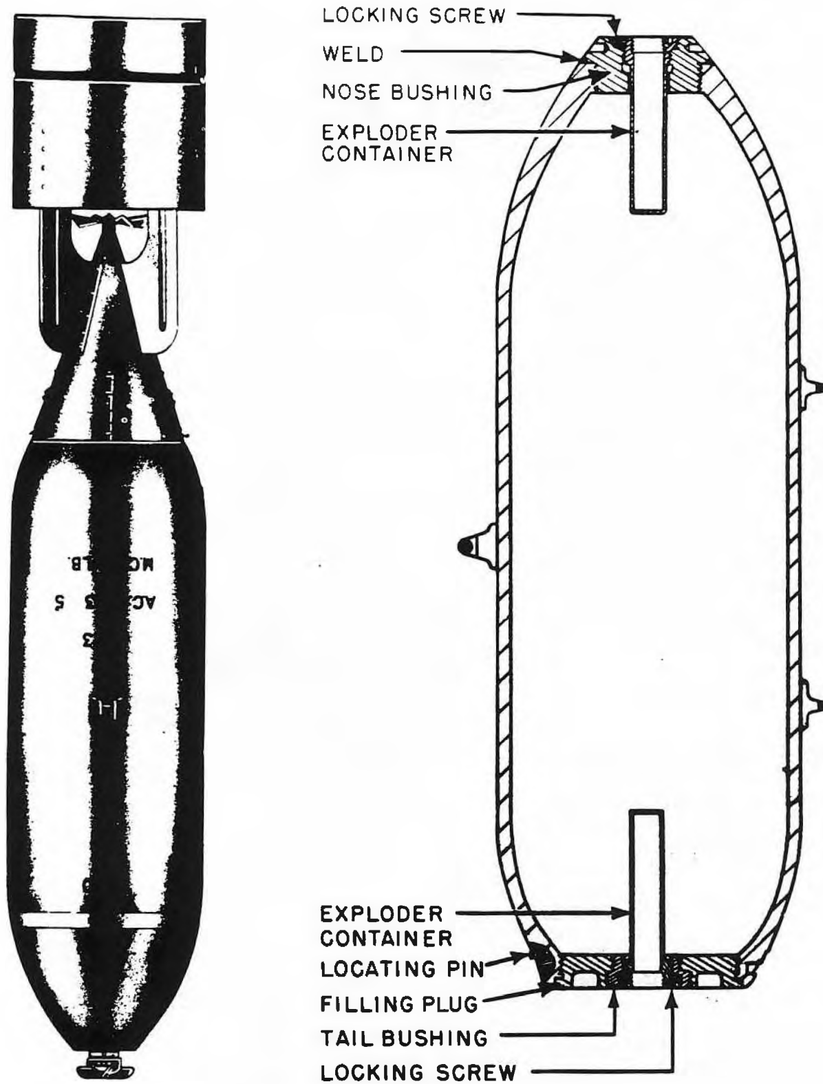
Figure 16—M.C. 500-lb. Bomb
