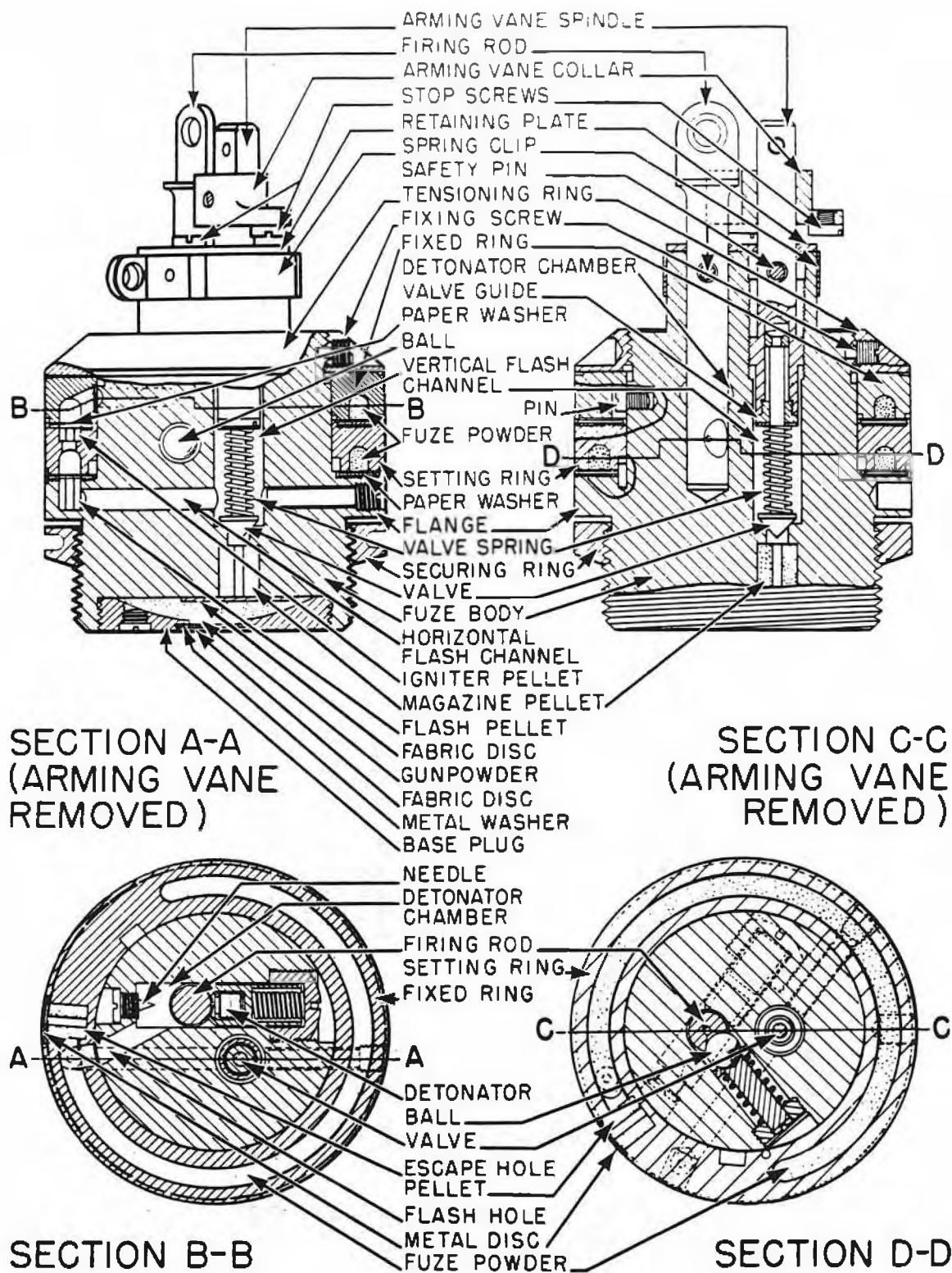
Figure 146—Nose Fuze No. 288
