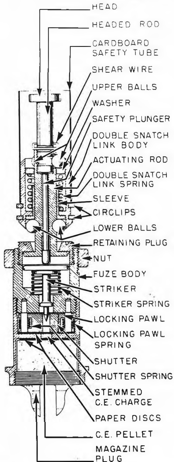
Figure 64—Special H.E. bomb fuze and double snatch link for Type H., A.D. Apparatus
