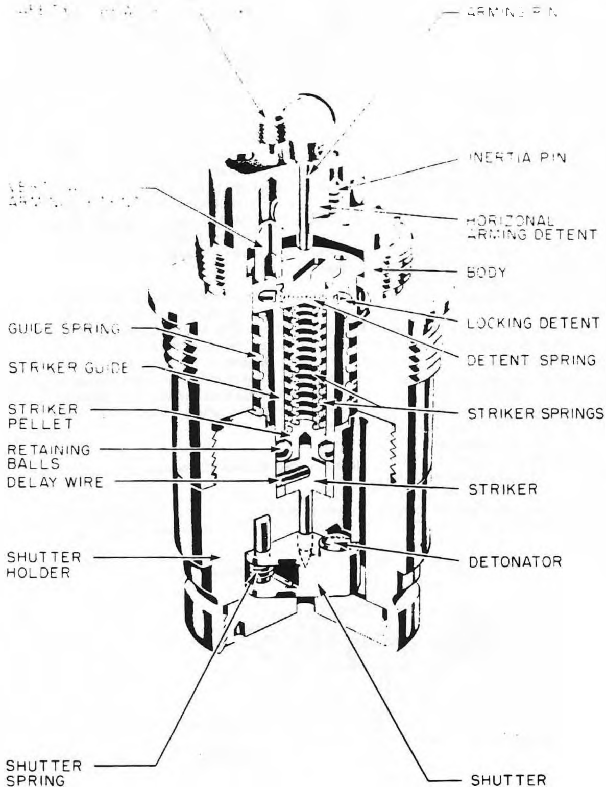
Figure 173—Tail Fuze No. 880 Mk II
