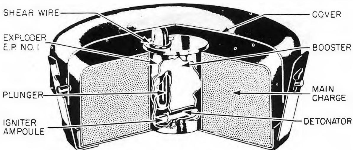
Figure 258—A./T. Mine E.P. Mk V
