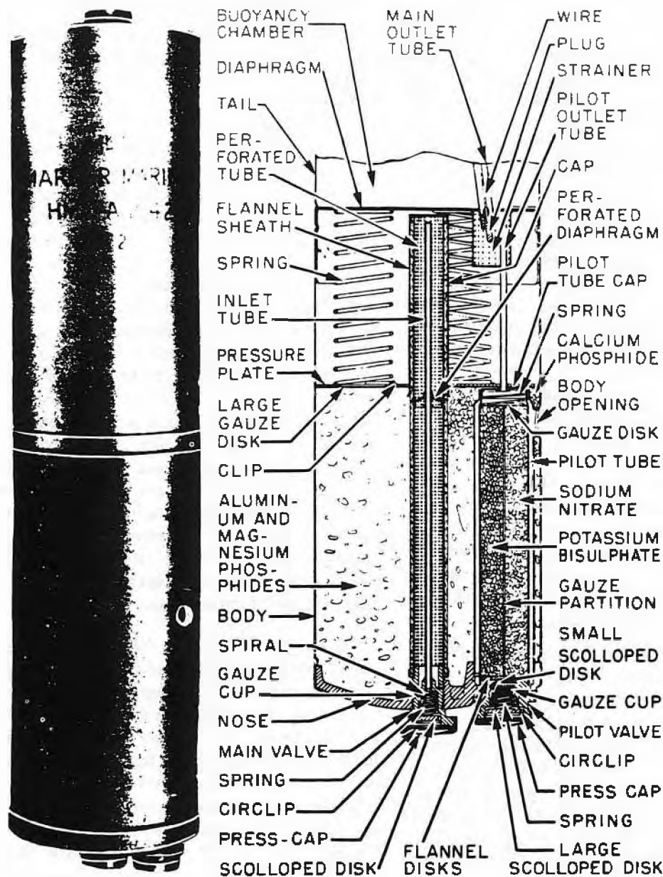
Figure 93—Marine Marker Mk I
