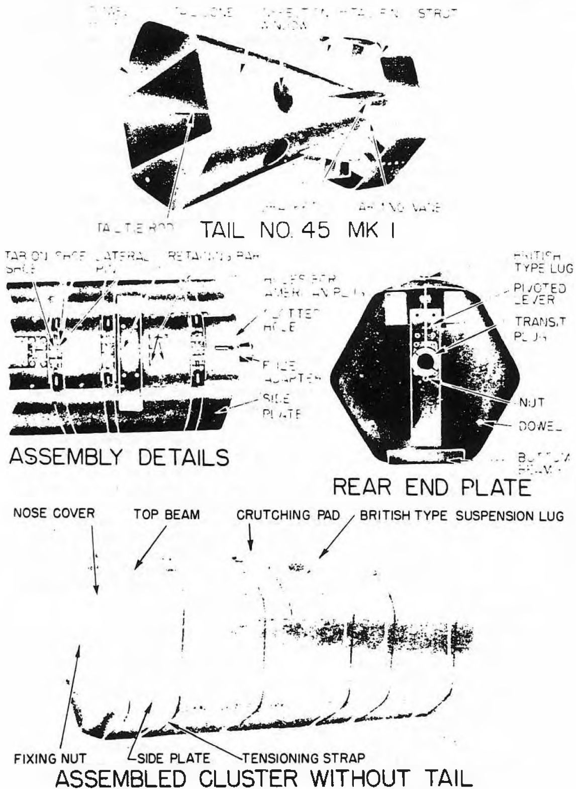
Figure 107—Cluster Projectile 500-lb. No. 6
