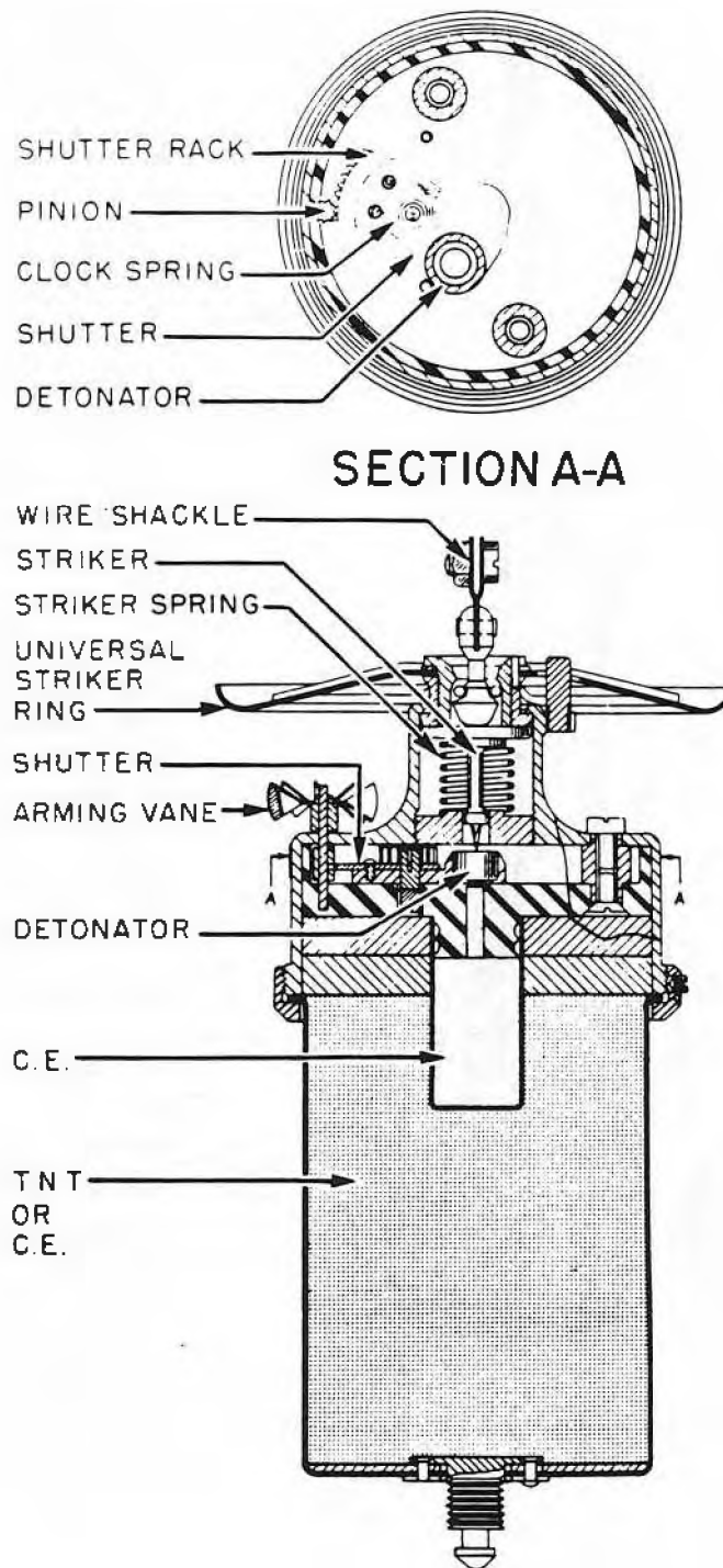
BOMB A.A.D. NO. 8 MK I
