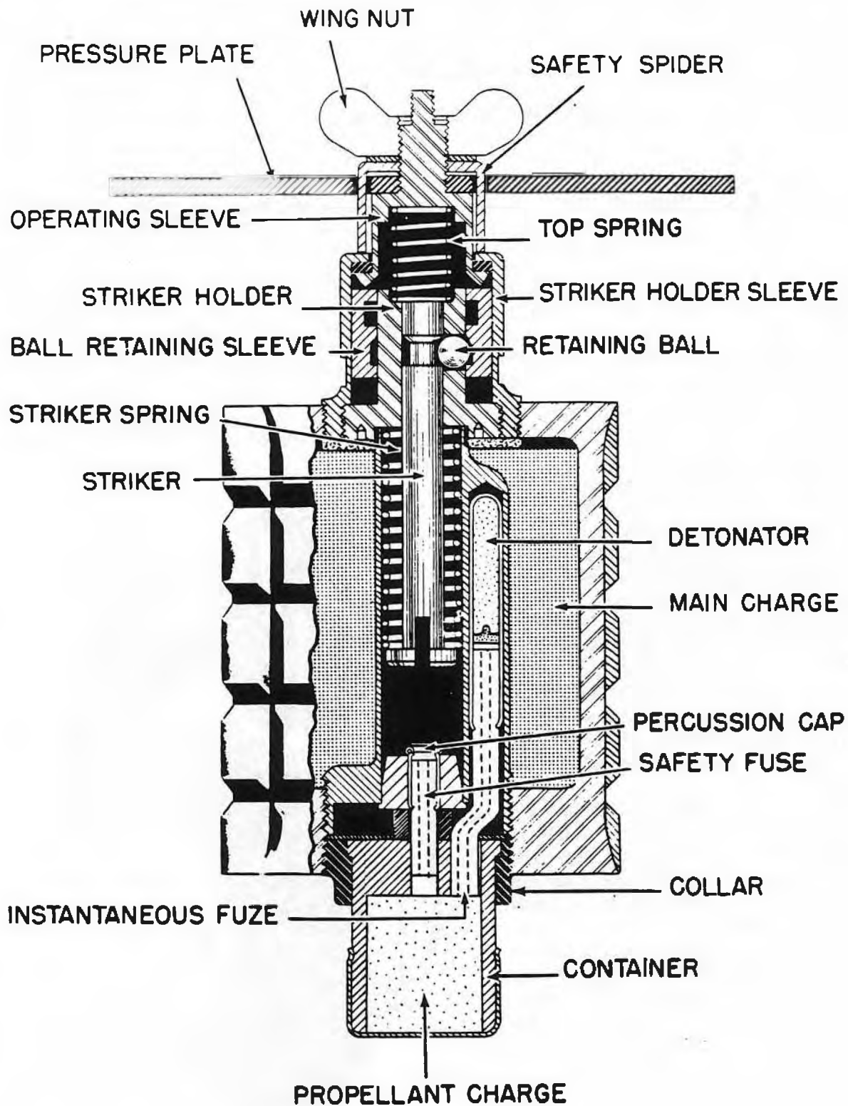
Figure 262—A./P. Mine No. 3 Mk I
