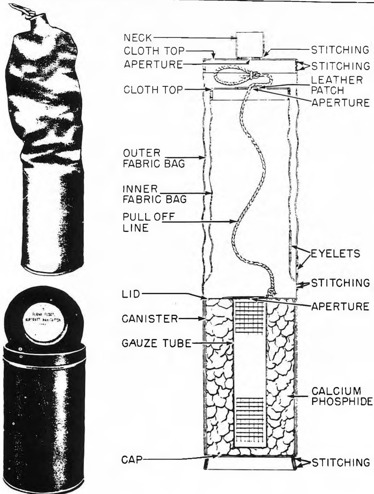
Figure 90—Navigation Flame Float Mk I
