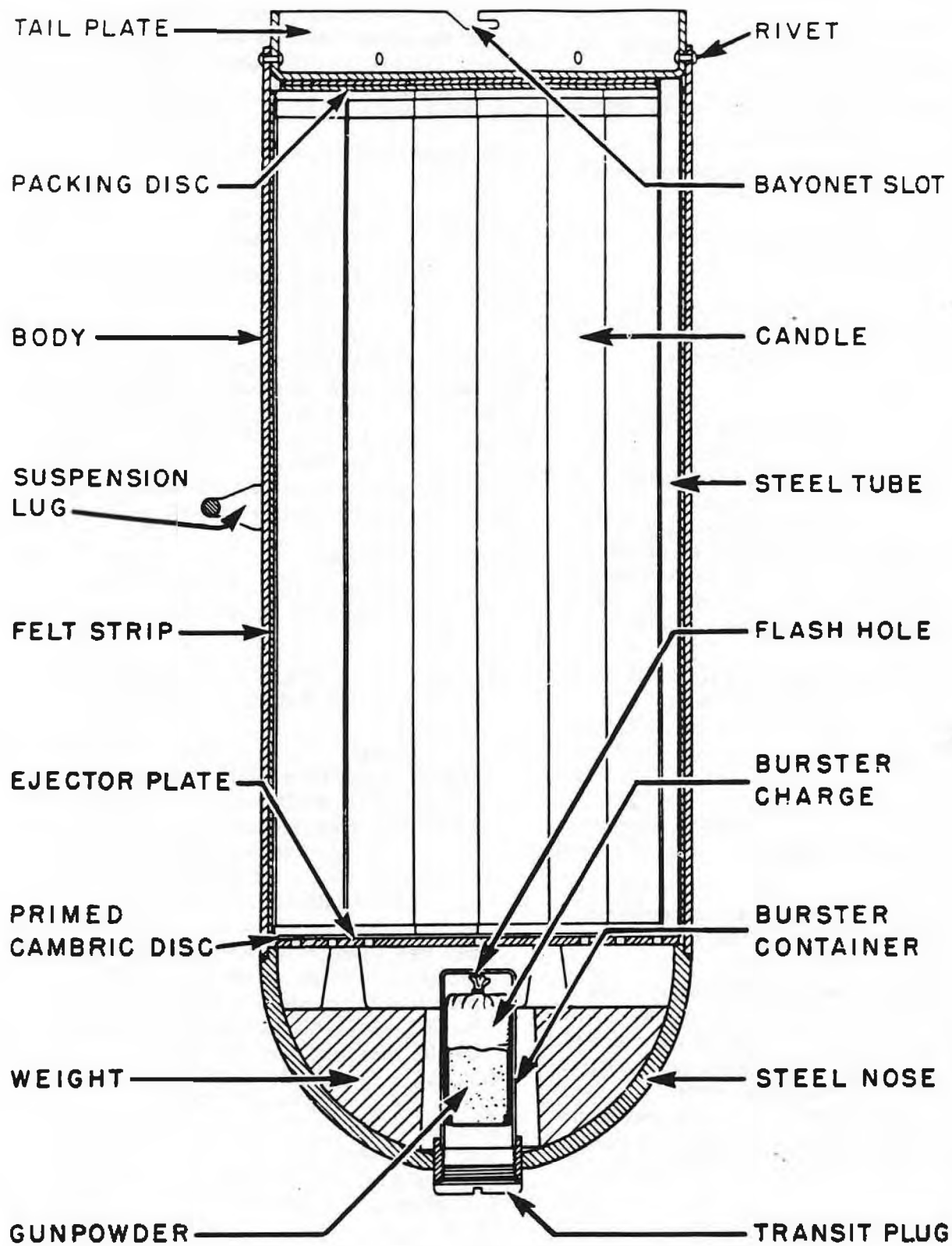
Figure 79—T.I. 250-lb., Skymarker, Bomb No. 14 Mk 1
