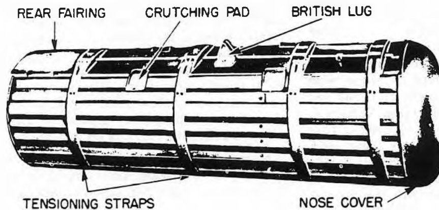
ASSEMBLED CLUSTER WITHOUT TAIL
