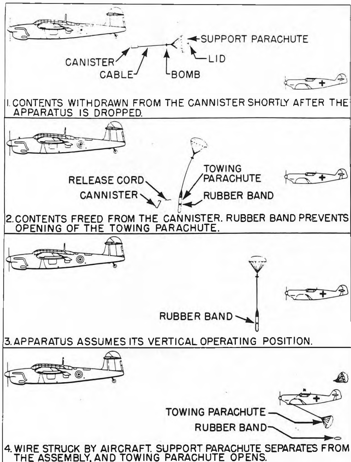
Figure 65—Operating sequence of the Type H., A.D. Apparatus
