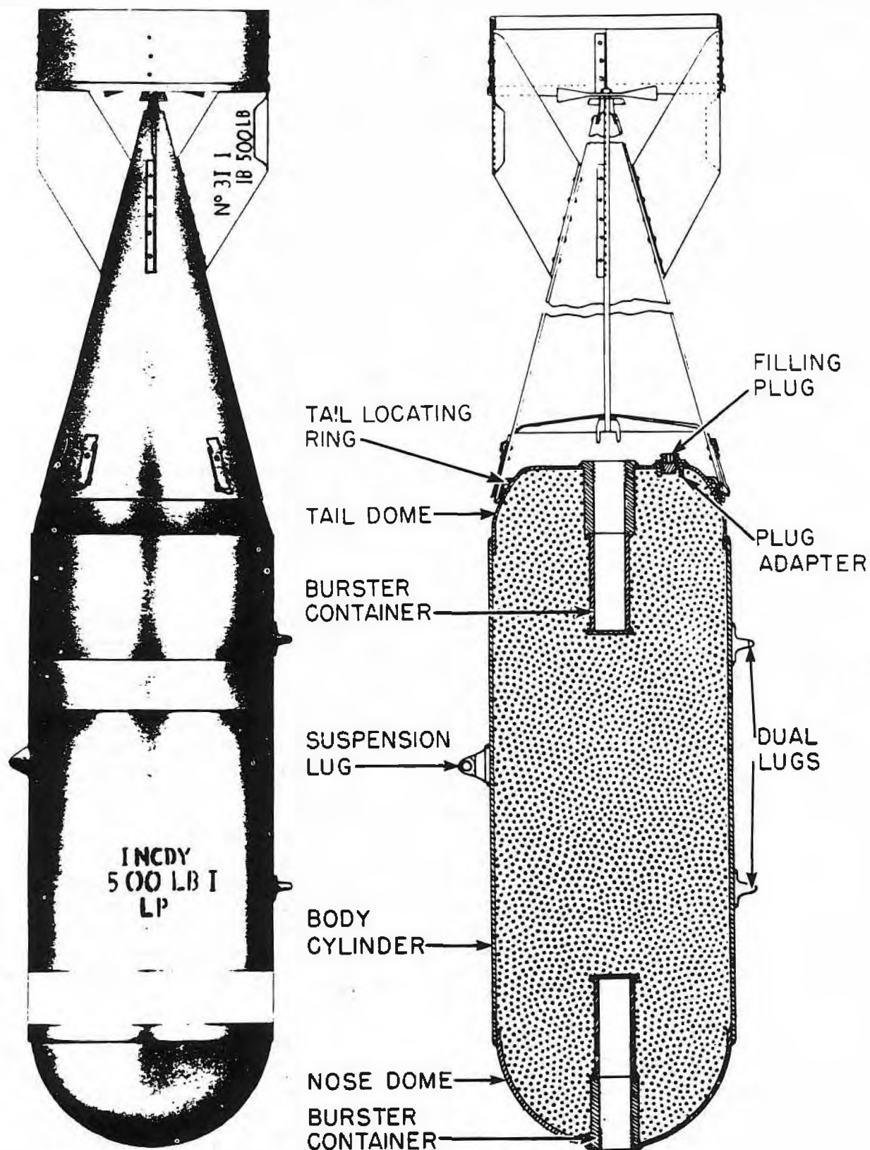
Figure 45—I.B. 500-lb. Mk I
