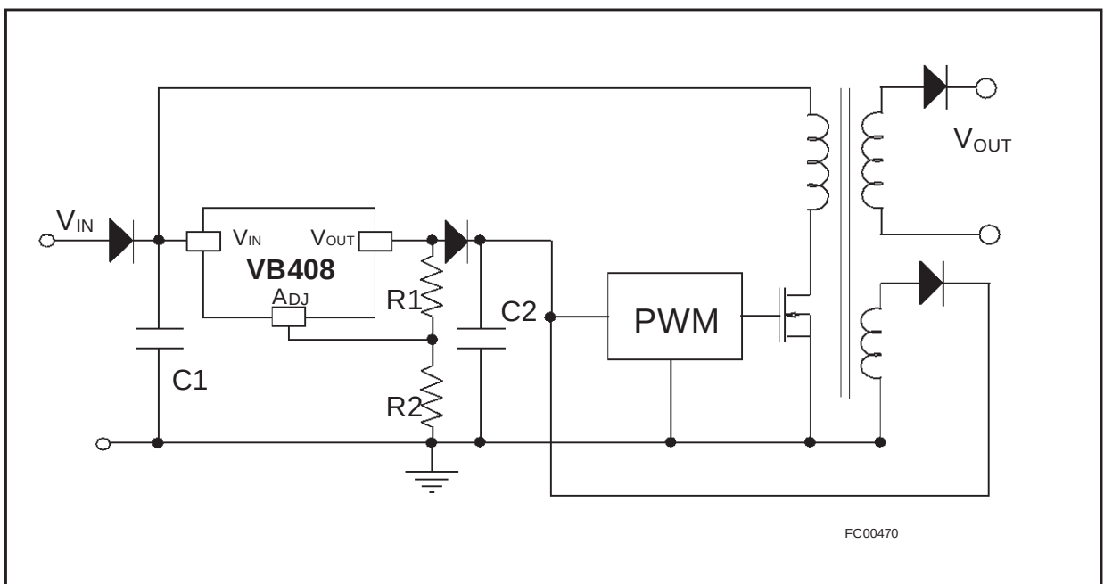
Figure 3: Start-up circuit
