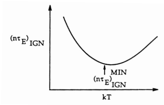
Figure 2: Ignition parameter.
