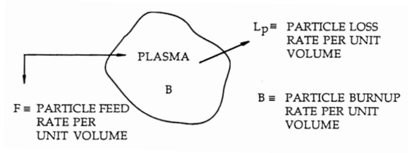
Figure 3: Particle balance.
