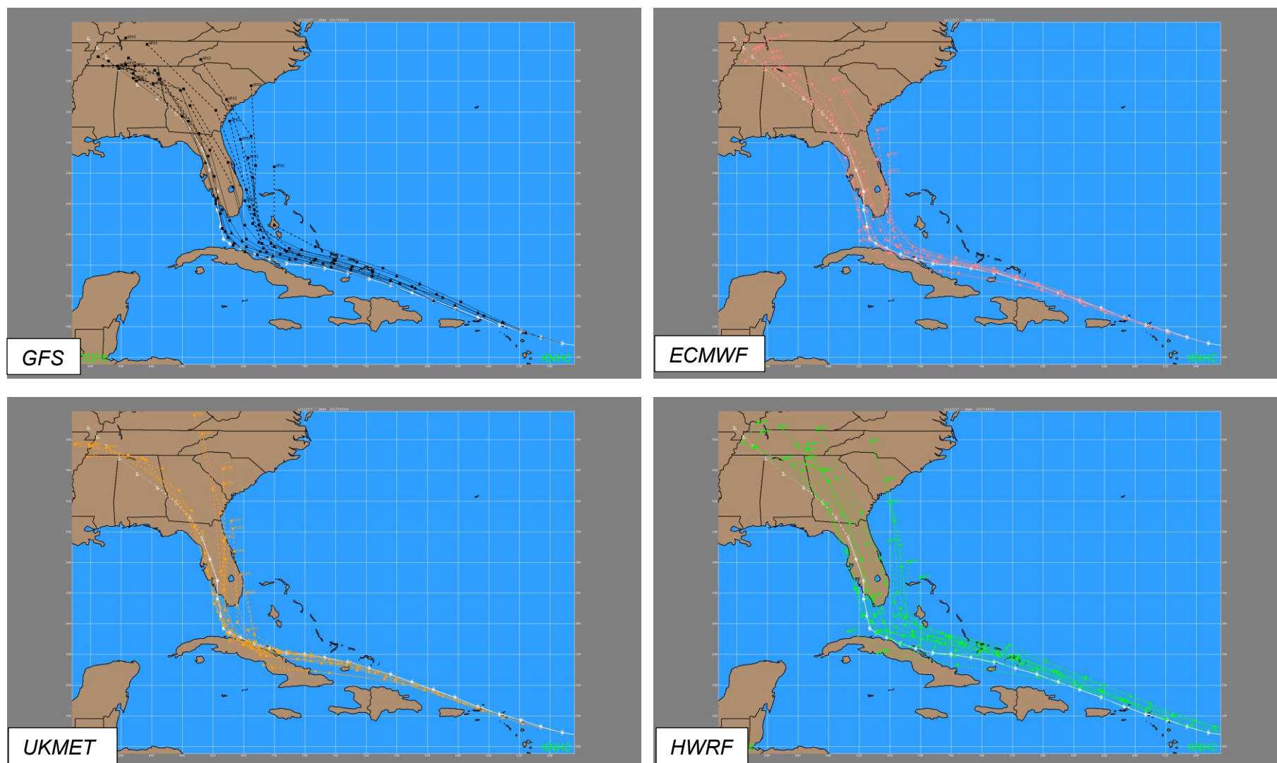
Figure 18. Selected model tracks from 1800 UTC 5 September to 1800 UTC 9 September. The best track is given by the white line with positions shown at 6 h intervals.
