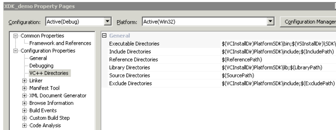
Figure 18-1 The Property Pages
