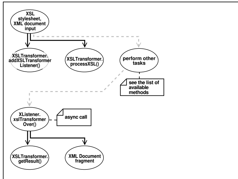
Figure D-2 XSLTransformer JavaBean Usage
