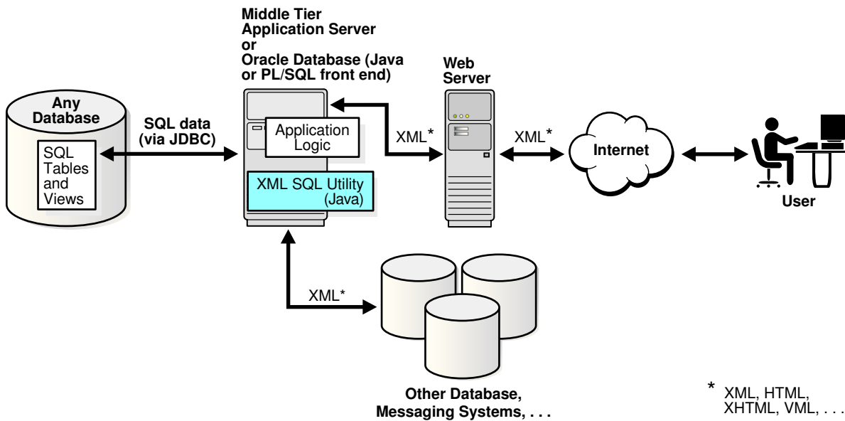
Figure 13-4 Running XSU in the Middle Tier
