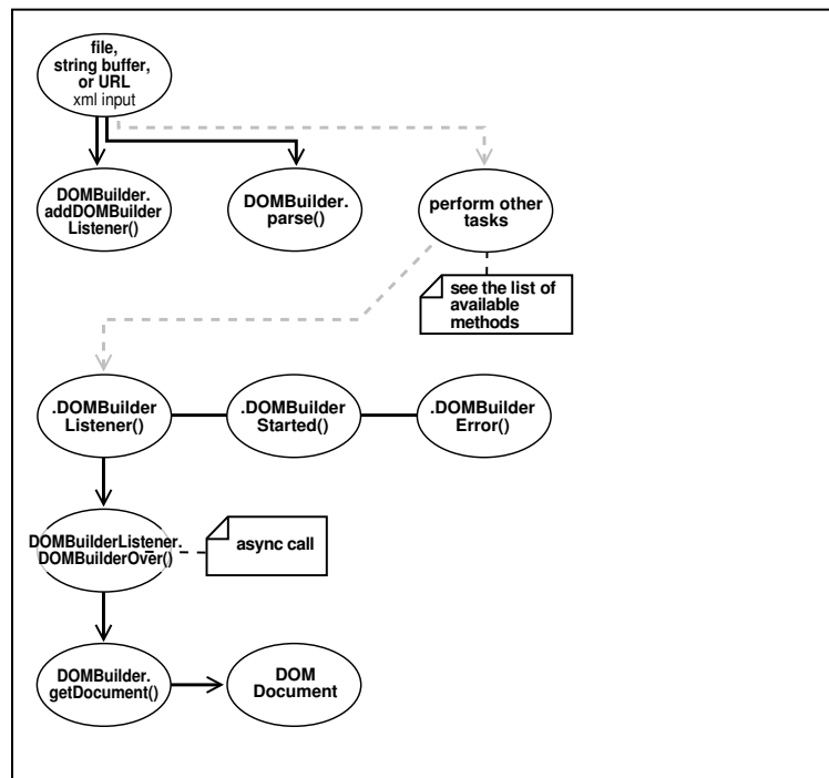
Figure D-1 DOMBuilder JavaBean Usage
