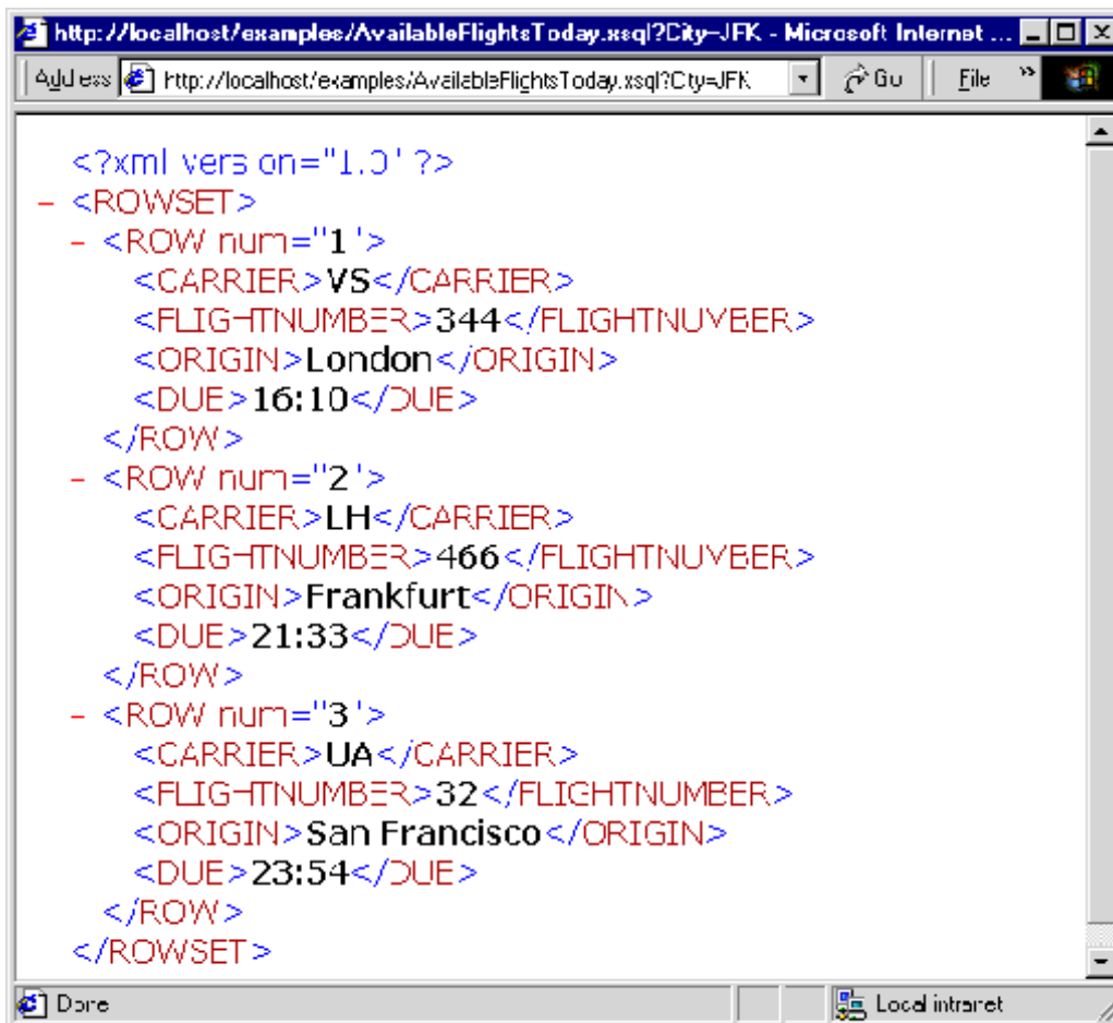
Figure 16-4 XML Result from XSQL Page (AvailableFlightsToday.xsql) Query
